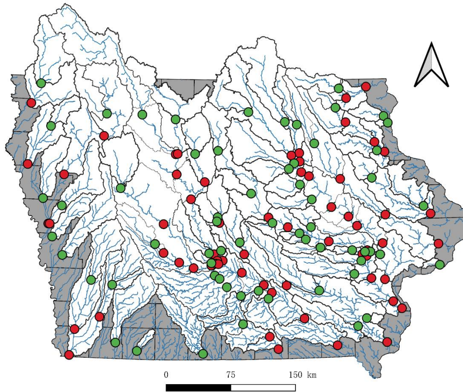
Figure 1. The location of 125 USGS gauges in the State of Iowa with single for upstream sub-basins (green dot) or multiple and large downstream basins (red dot) stream-gages.
