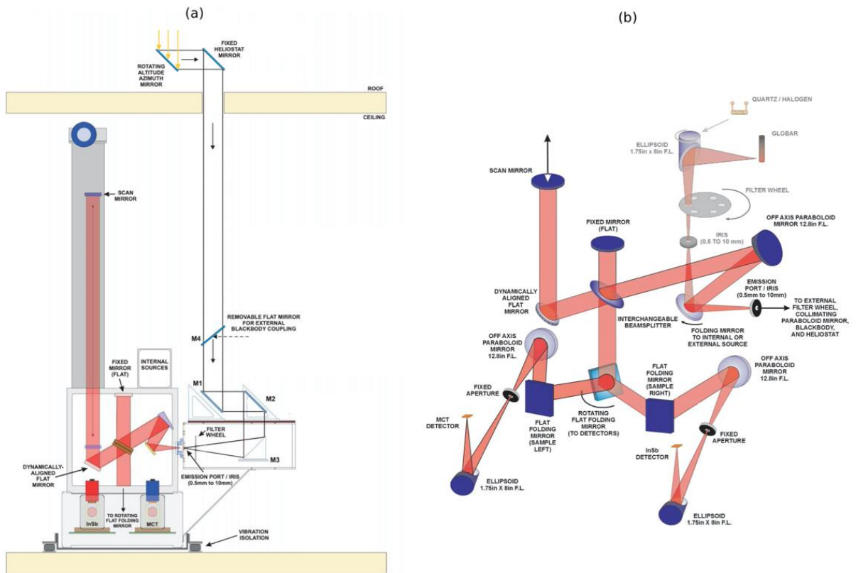
934 Figure 1: (a) The FTIR spectrometer and solar tracker installation at TAO: mirrors M1, M2 and M3 couple the 935 heliostat optics to the DA8 and M4 is a removable mirror. (b) The optical layout of the DA8 FTIR: a moving folding 936 mirror selects between the emission port used for solar absorption measurements and internal sources (shown in grey). 937 Figures taken from Wiacek (2006), adapted from ABB Bomem Inc. facility schematics.
