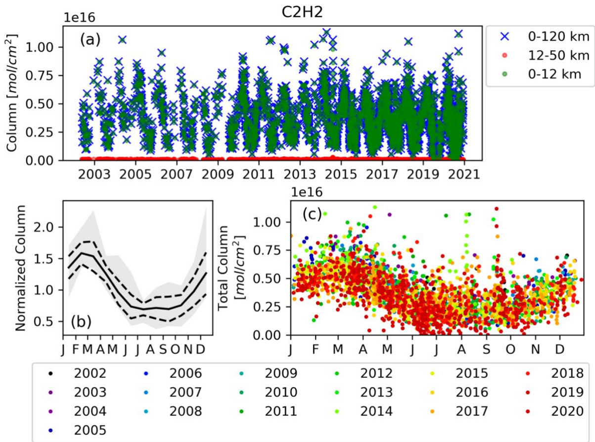
1025 Figure 33: Same as Figure 24 but for C 2 H 2 .
