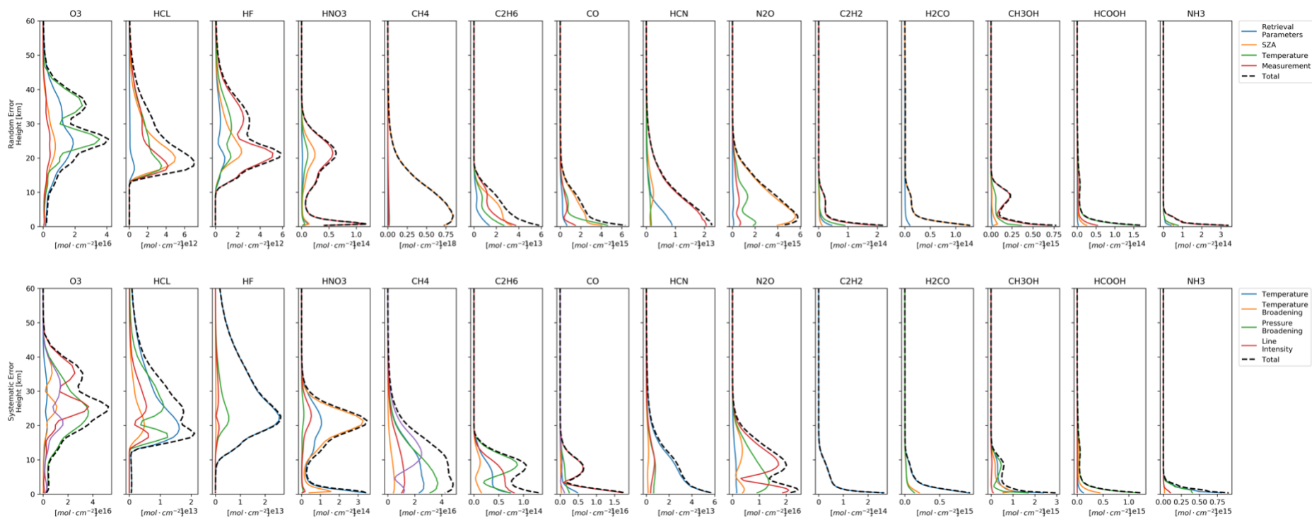
998 Figure 23: Mean systematic and random error profiles (diagonal elements of S_{\text{sys}} and S_{\text{ran}} ) of \text{O}_3 , \text{HCl} , \text{HF} , \text{HNO}_3 , \text{CH}_4 , \text{C}_2\text{H}_6 , \text{CO} , \text{HCN} , \text{N}_2\text{O} , \text{C}_2\text{H}_2 , \text{H}_2\text{CO} , \text{CH}_3\text{OH} , \text{HCOOH} , and \text{NH}_3 999 from 2019. Upper panels: Retrieval parameter, SZA, random temperature and measurement error comprising the random uncertainty. Lower panels: Systematic temperature, line 1000 intensity, temperature-broadening and pressure-broadening error comprising the systematic error.
