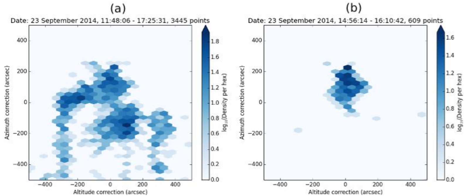
944 945 Figure 4: Solar tracker azimuth and altitude corrections for the original quadrant diode active tracking system during a day of testing in September 2014: (a) for an entire day including 946 manual realignments, and (b) at a single position.
