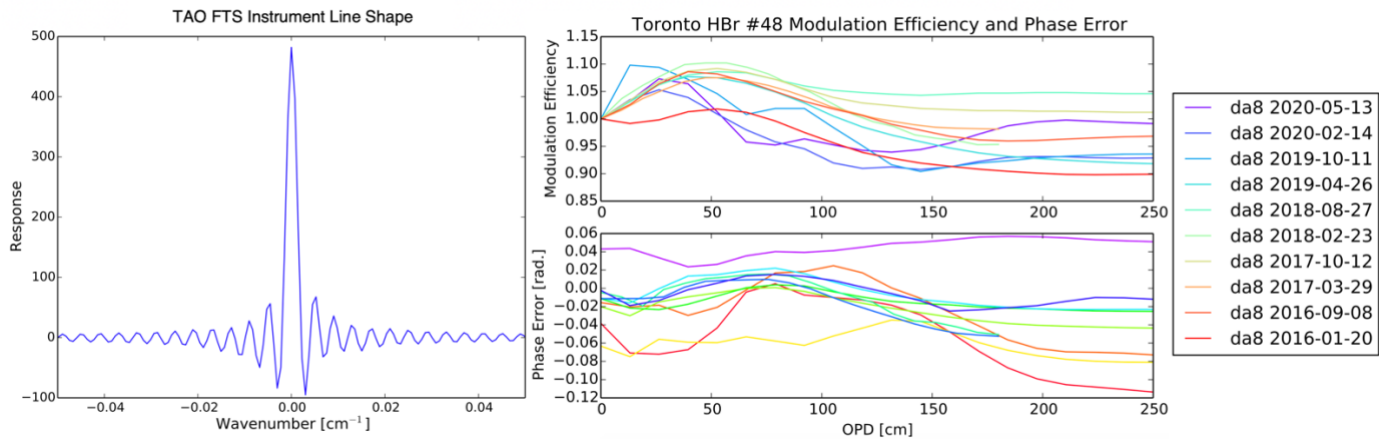
941 Figure 3: TAO DA8 solar instrument line shape (left) (taken on 13 May 2020), modulation efficiency (top, right) and 942 phase error (bottom, right) (various measurements from 2016 to 2020 shown), with HBr cell #48 at 0.004 cm -1 943 resolution, obtained using LINEFIT v14.5.
