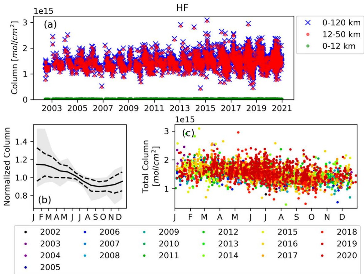
1010 Figure 26: Same as Figure 24 but for HF.
