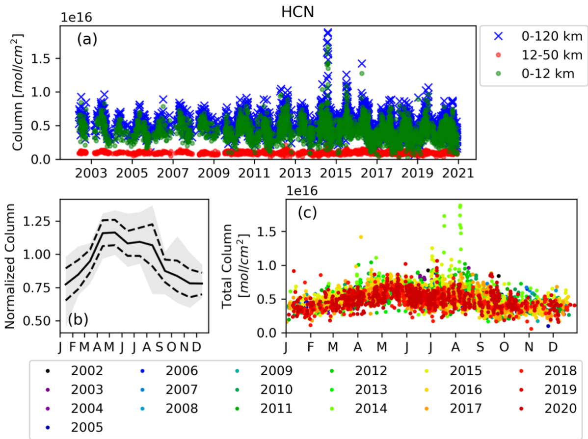
1020 Figure 31: Same as Figure 24 but for HCN.
