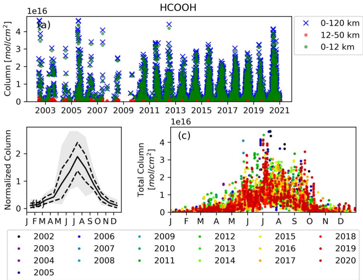
Figure 36: Same as Figure 24 but for HCOOH.
