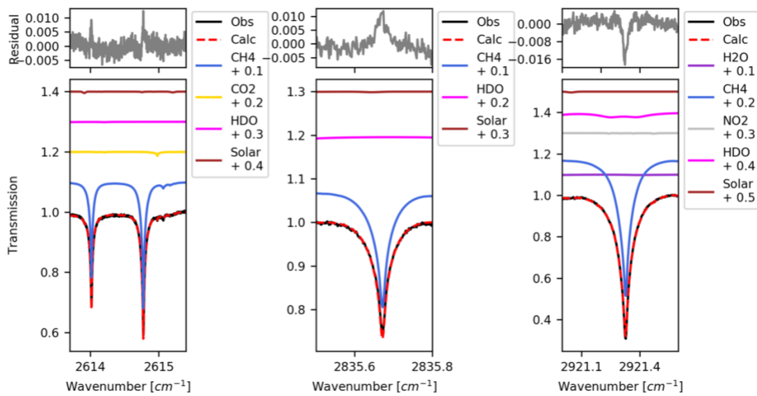
969 Figure 12: Same as Figure 8 but for CH 4 using a spectrum recorded at 16:36:54 UTC on January 11, 2019.
