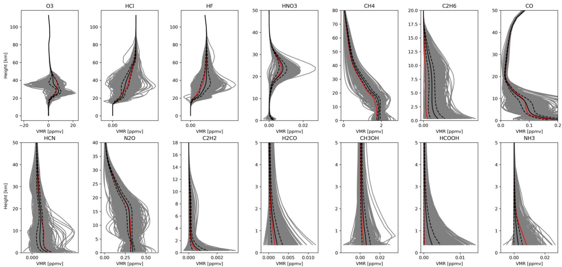
954 Figure 7: Retrieved profiles of O 3 , HCl, HF, HNO 3 , CH 4 , C 2 H 6 , CO, HCN, N 2 O, C 2 H 2 , H 2 CO, CH 3 OH, HCOOH, and NH 3 from 2002 to 2020. The mean profile is plotted in black with 955 the two black dashed lines corresponding to \pm 1\sigma standard deviation from the mean. The a priori profile is plotted as a red line.
