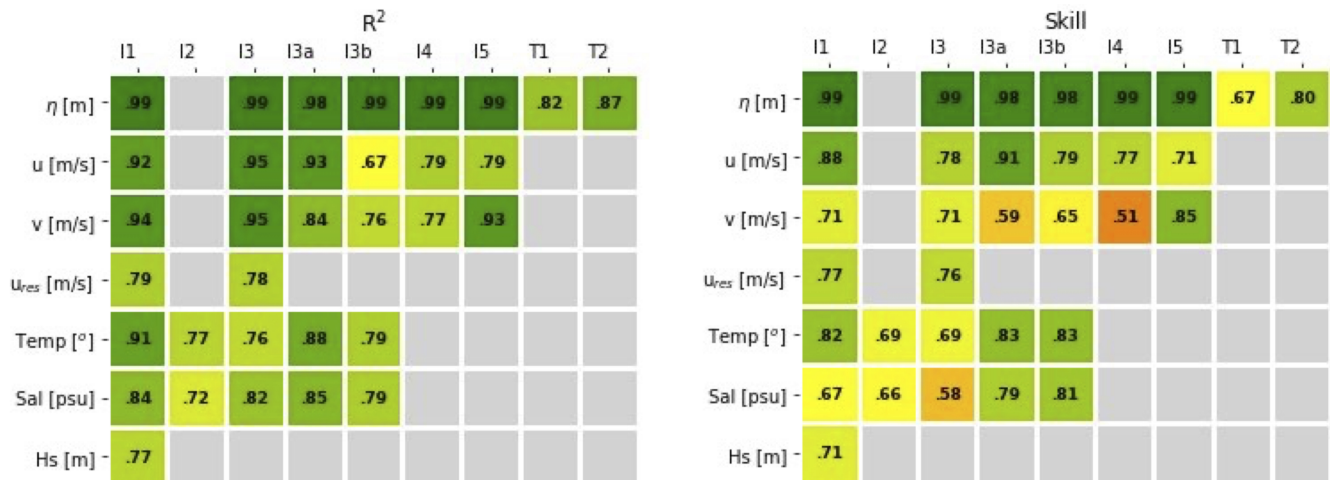
Figure 2. (a) Correlation coefficient ( R^2 ) and (b) skill coefficient (formulation proposed by Willmott (1981)) of the water level, east and north instantaneous velocity, residual velocity, temperature, salinity and wave height for each station. The color indicates the degree of accuracy (green excellent agreement, yellow–orange good agreement and red poor agreement).
