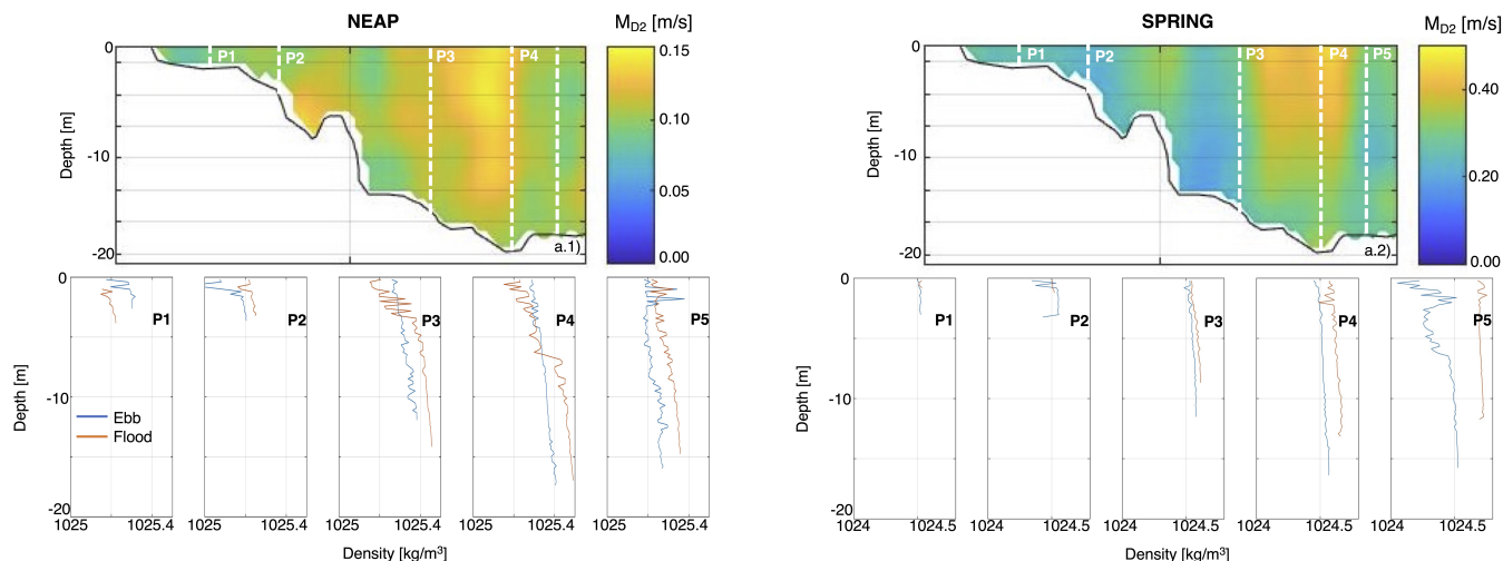
Figure 6. Amplitude of the tidal harmonic species D2 of the current during Neap2013 (a.1) and Spring2013 (a.2). The second rows show the density profile (P1-P5) during Neap2013 and Spring2013 at maximum flood (orange line) and ebb (blue line). The location of each profile is indicated by white dashed lines in a.1 and a.2.
