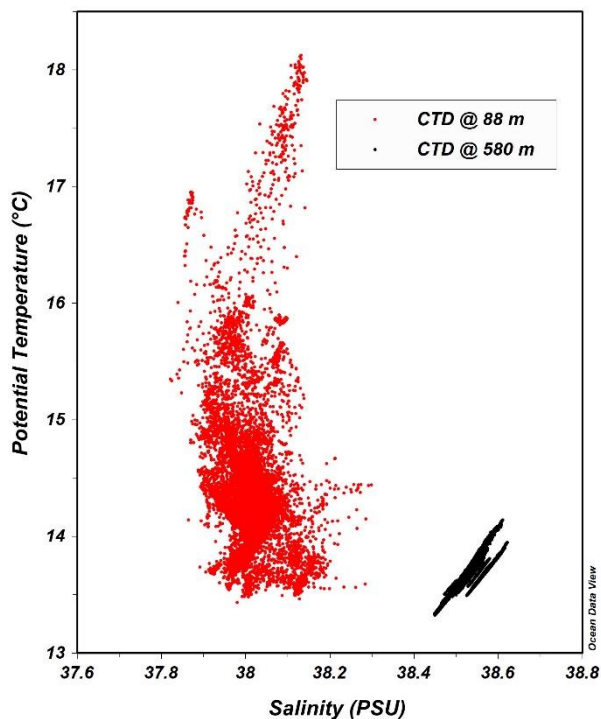
245 Figure 5: Temperature-salinity (T-S) diagram for the LCM site, obtained from CTD measurements covering the period November 2020 – October 2022.
