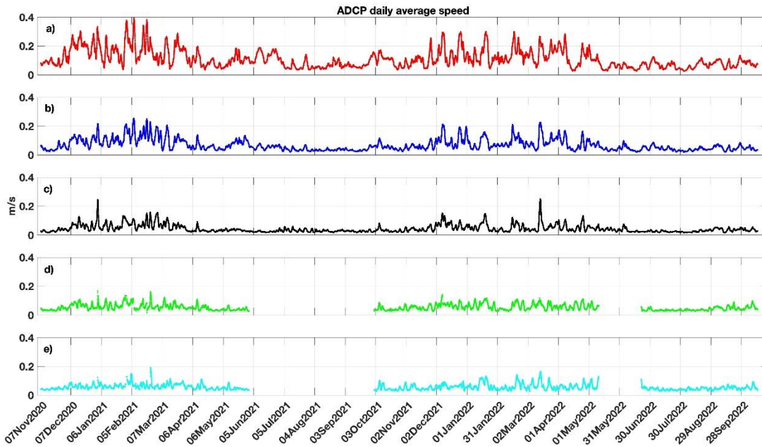
Figure 8: Time series of the current speed (m/s) in the 5 different layers assumed in the analysis by applying a daily average smoothing (UL: Upper Layer; UIL: Upper Intermediate Layer; IL: Intermediate Layer; LIL: Lower Intermediate Layer; BL: Bottom Layer).
