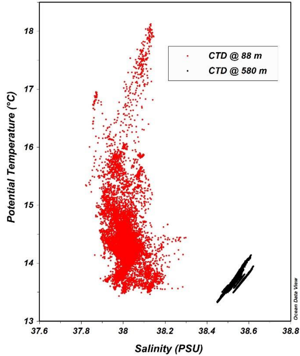
245 Figure 5: Temperature-salinity (T-S) diagram for the LCM site, obtained from CTD measurements covering the period November 2020 – October 2022.
