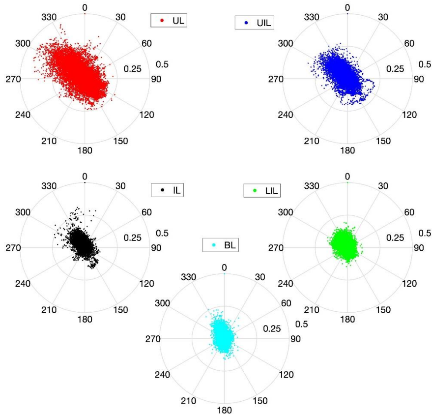
275 Figure 7: Polar scatter plot of observed directional current velocity (m/s) on the LCM site. (UL: Upper Layer; UIL: Upper Intermediate Layer; IL: Intermediate Layer; LIL: Lower Intermediate Layer; BL: Bottom Layer).
