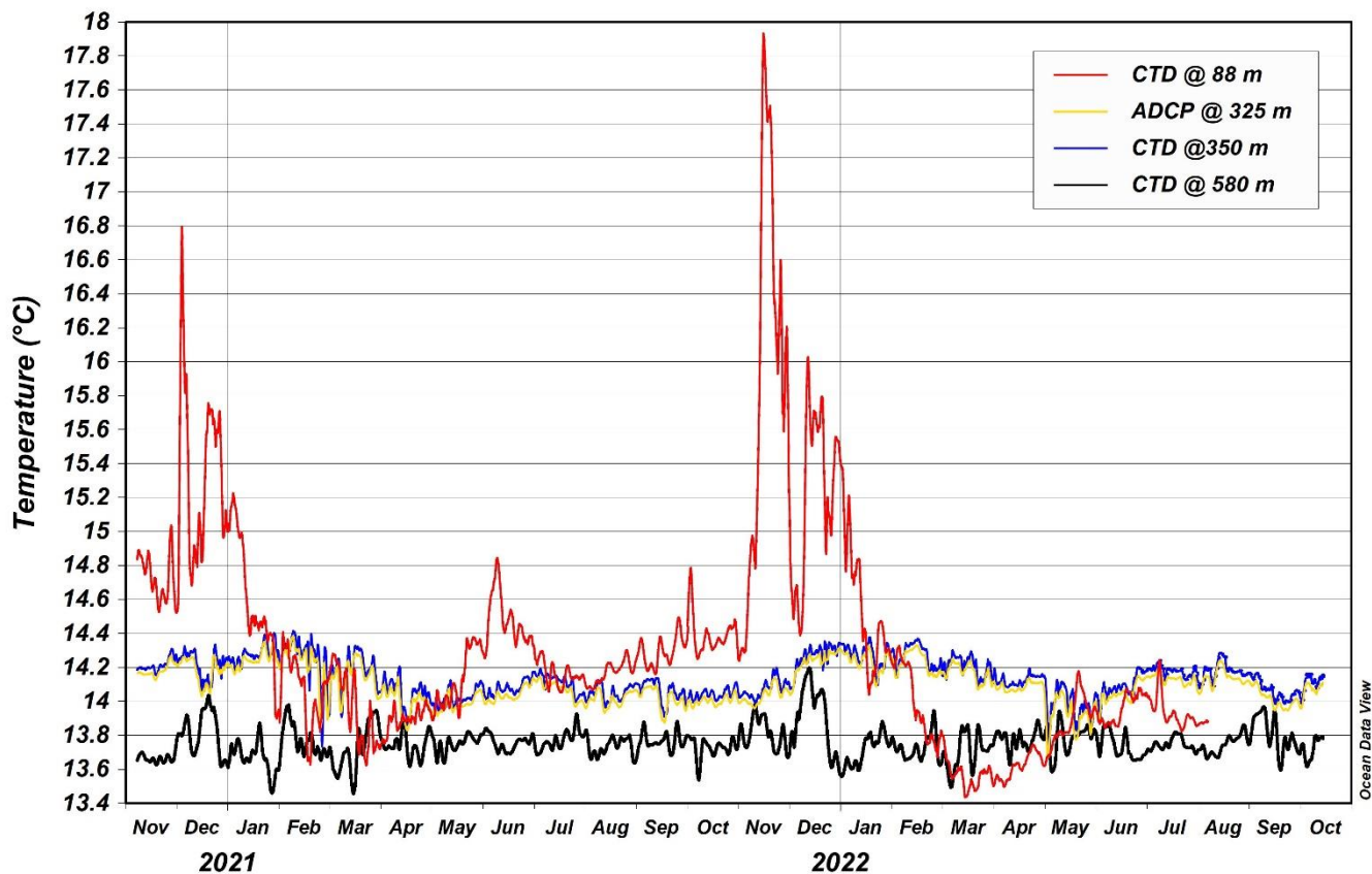
Figure 3: CTD and ADCP temperature records on LCM site. The data are presented with a 3-day smoothing window.
