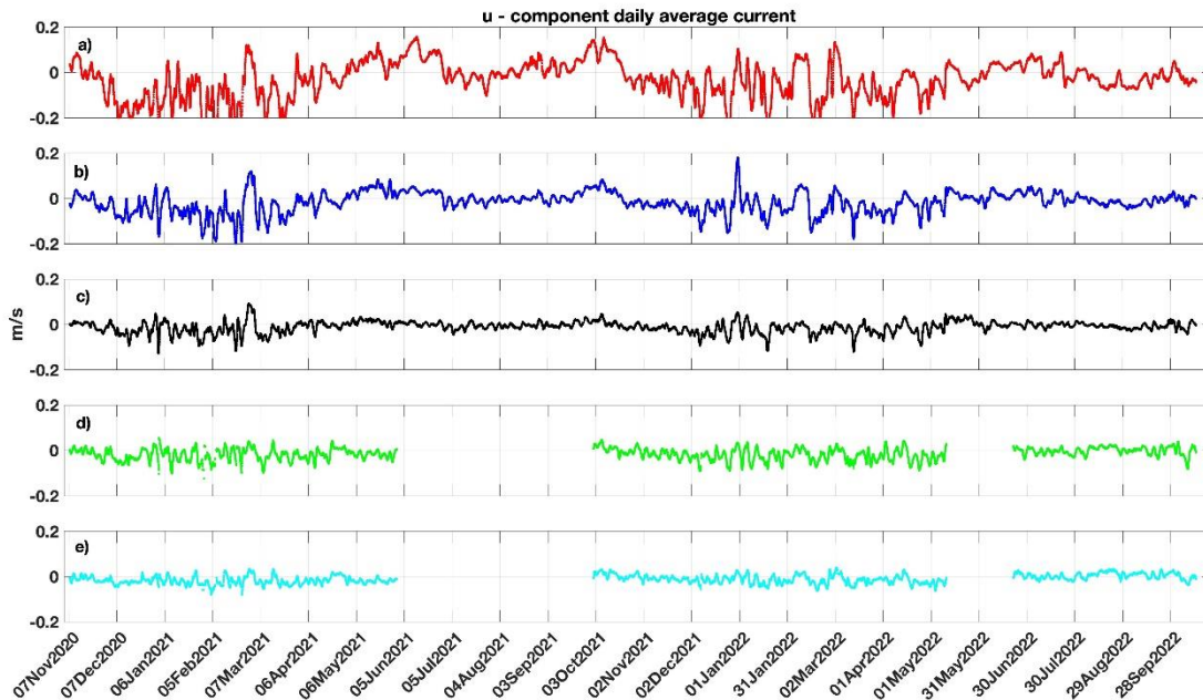
Figure 9: Time series of the East component of the current speed (m/s) in the 5 different layers assumed in the analysis by applying a daily average smoothing (UL: Upper Layer; UIL: Upper Intermediate Layer; IL: Intermediate Layer; LIL: Lower Intermediate Layer; BL: Bottom Layer).
