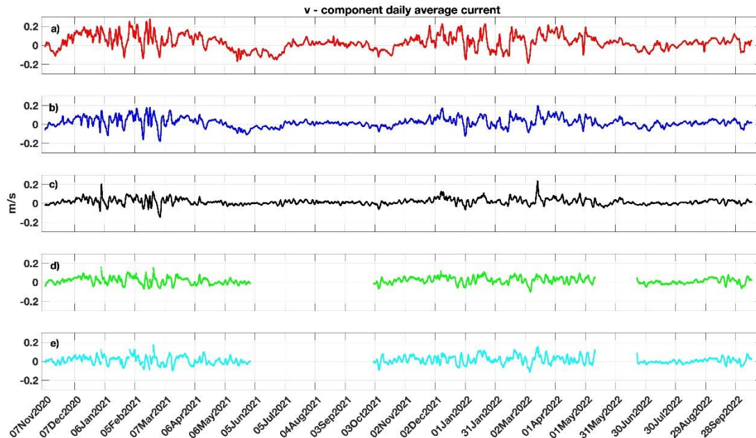
295 Figure 10: Time series of the of the North component of the current speed (m/s) in the 5 different layers assumed in the analysis by applying a daily average smoothing (UL: Upper Layer; UIL: Upper Intermediate Layer; IL: Intermediate Layer; LIL: Lower Intermediate Layer; BL: Bottom Layer).
