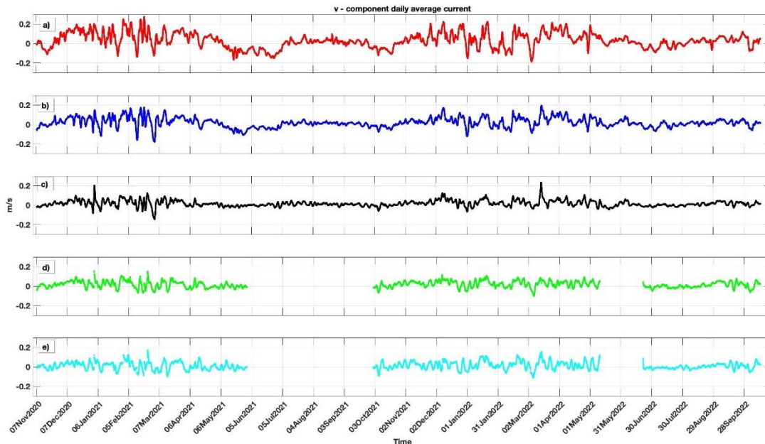
300 Figure 10: Time series of the of the North component of the current speed in the 5 different layers assumed in the analysis by applying a daily average smoothing (UL: Upper Layer; UIL: Upper Intermediate Layer; IL: Intermediate Layer; LIL: lower intermediate layer; BL: Bottom Layer).
