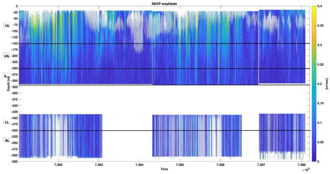
275 Figure 6: Currents speed records along the LCM water column (data filtered as described in the data quality check section), boxes on the left and straight lines indicate the 5 different layers assumed in the analysis (UL: Upper Layer; UIL: Upper Intermediate Layer; IL: Intermediate Layer; LIL: lower intermediate layer; BL: Bottom Layer)
