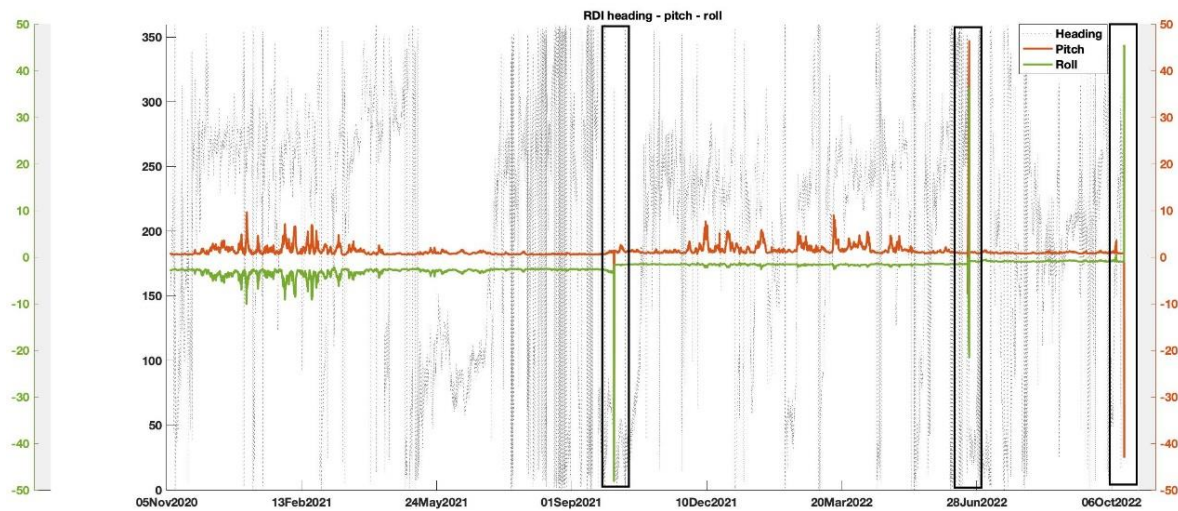
180 Figure 2: Measurements of heading, pitch and roll from the RDI ADCP. The black boxes indicate each recovery.
