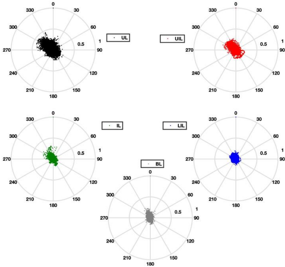
280 Figure 7: Polar scatter plot of observed directional current velocity (ms-1) on the LCM site. (UL: Upper Layer; UIL: Upper Intermediate Layer; IL: Intermediate Layer; LIL: lower intermediate layer; BL: Bottom Layer).
