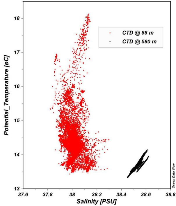
Figure 5: Temperature-salinity (T-S) diagram for the Levante Canyon Site, obtained from CTD measurements covering the period November 2020– October 2022.
