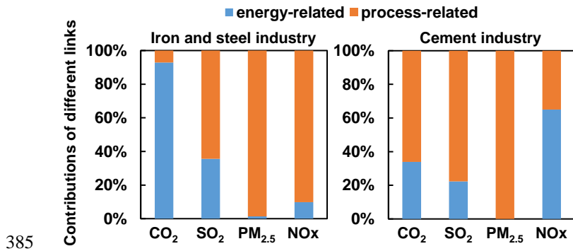
385 Figure 8: Deconstruction of emissions from major industrial sectors in 2021 in China.
