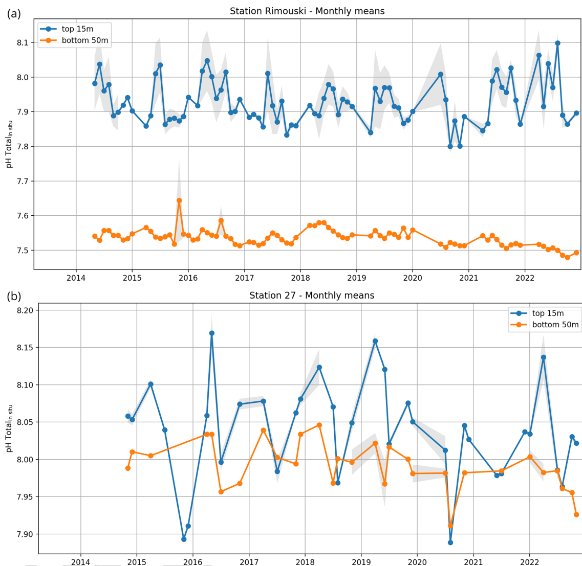
Figure 4. Monthly averages of pH data at Rimouski station (a) and Station 27 (b). Surface observations (blue curves) are considered the average of the top 15 m, and bottom observations (orange curves) are the average of the bottom 50 m. The shaded area correspond to \pm 0.5 SD of the monthly distribution (when more than one visit per month is made). The tick marks on the horizontal axis correspond to the beginning of the year.
