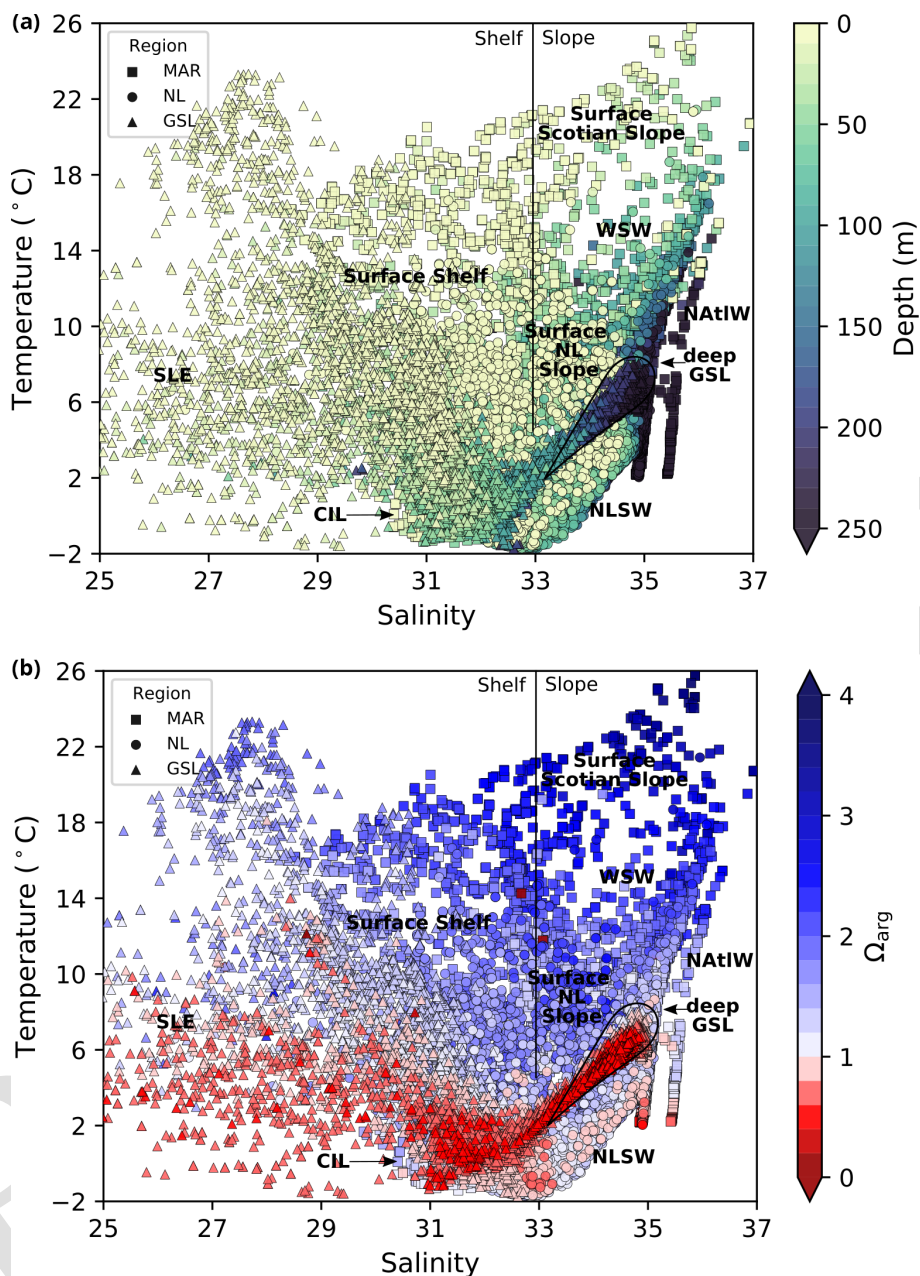
Figure 2. Diagrams of temperature and salinity vs. depth (a) and temperature and salinity vs. saturation state relative to aragonite for all bottle samples in the dataset. The three regions of the Atlantic Zone are shown using different markers. An approximate division between the shelf and slope surface waters is indicated by the vertical black line at a salinity value of 33. Various water masses are labelled as follows: WSW, Warm Slope Water; NATIW, North Atlantic Water; and NLSW, Newfoundland and Labrador Slope Water. In the absence of a clear water mass definition, the origin of the water is labelled as follows: LSLE, Lower St. Lawrence Estuary; GSL, Gulf of St. Lawrence; and LS, Labrador Shelf.
