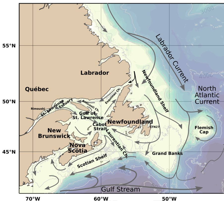
Figure 1. Bathymetric map of the Atlantic Zone (i.e., the Newfoundland and Labrador shelves and slopes, the Scotian Shelf and Slope, the Gulf of St. Lawrence, and the St. Lawrence Estuary) (CBI). Also identified are the deep channels within the Gulf of St. Lawrence: the Laurentian, Anticosti and Esquimaux channels. The approximate position and direction of the major current systems and their shelf and slope components are illustrated as arrows: the Gulf Stream (grey) and the Labrador Current (black).
