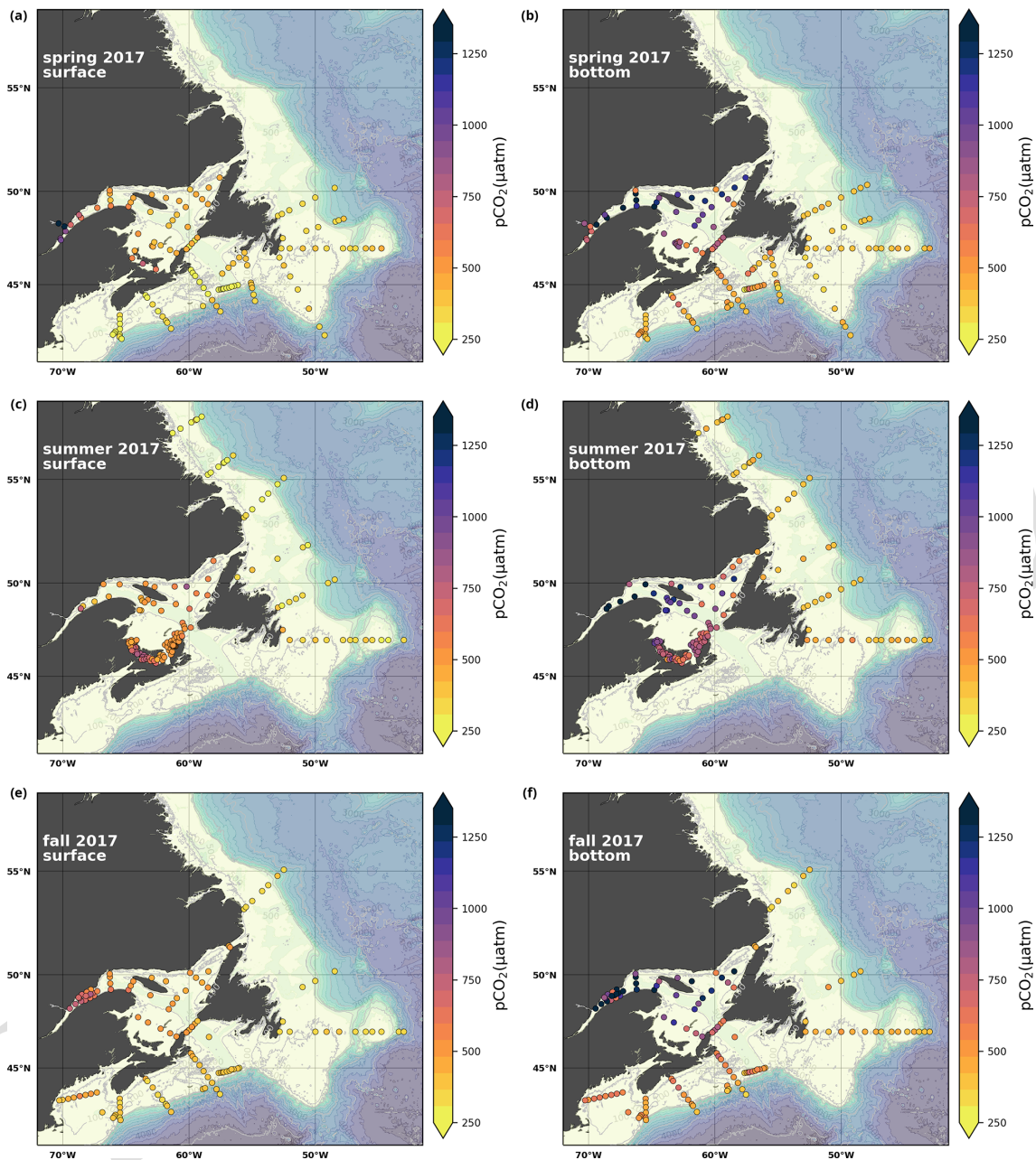
Figure A6. Same as in Fig. A1 but for pCO 2 .
