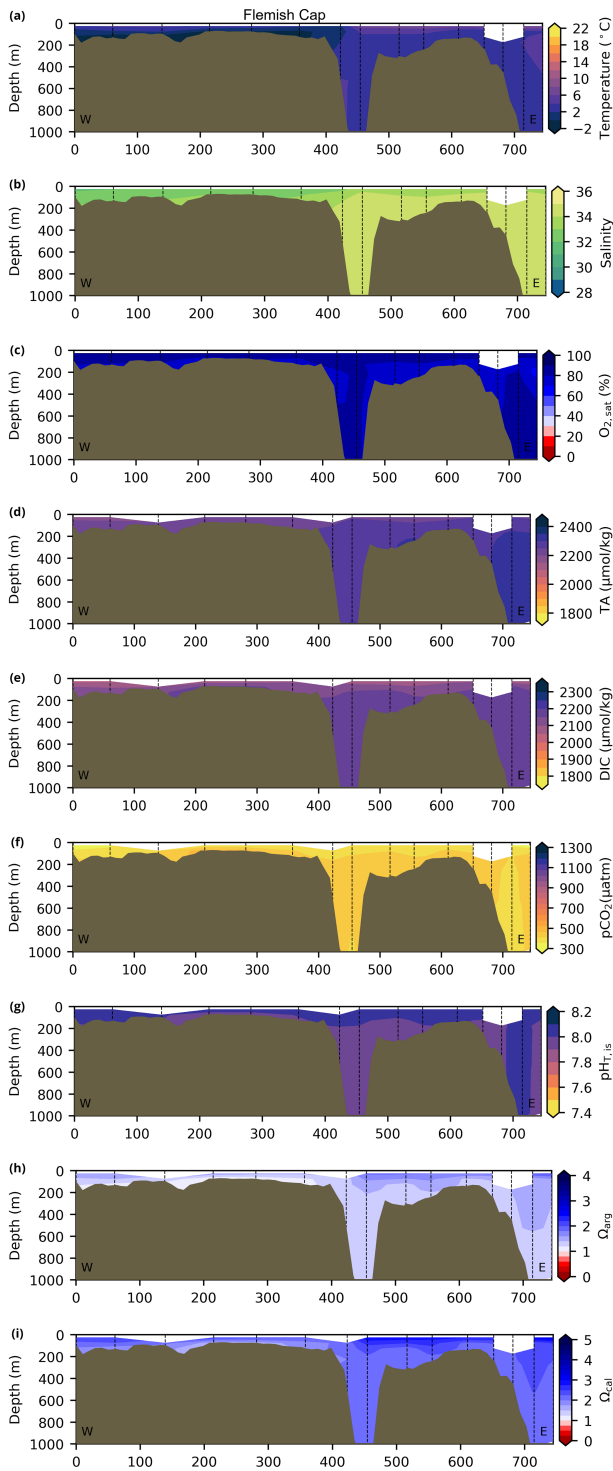
Figure B2. Same as in Fig. B1 but for the hydrographic section of Flemish Cap (NL region; see Fig. 3 for location).
