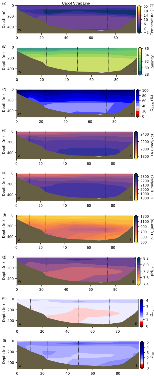
Figure B4. Same as in Fig. B1 but for the hydrographic section of Cabot Strait (GSL region; see Fig. 3 for location).
