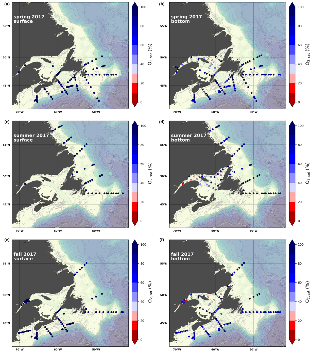
Figure A3. Same as in Fig. A1 but for O_{2,sat} .
