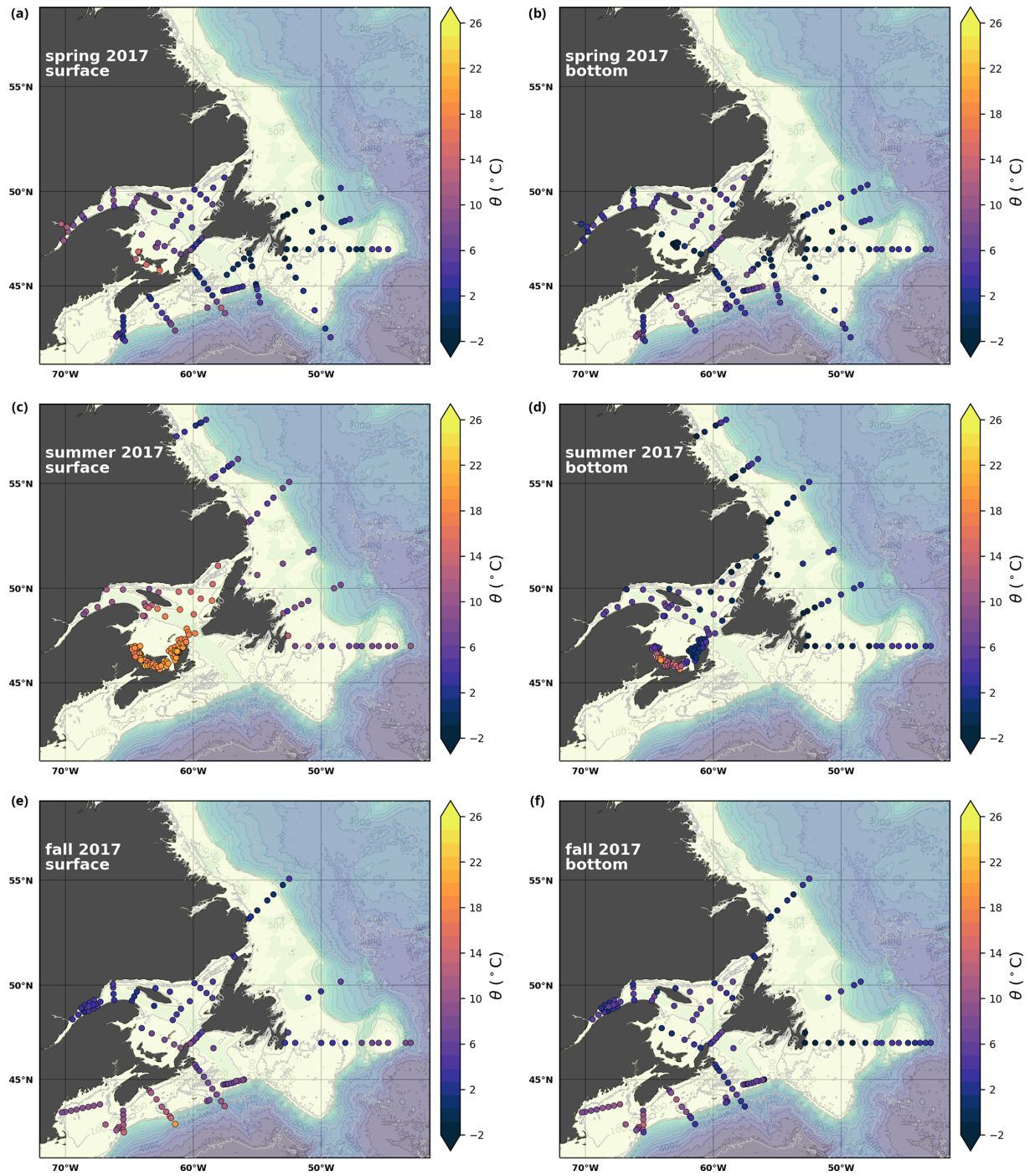
Figure A1. Surface (uppermost sample < 52\text{ m} ; a, c, e ) and near-bottom (deepest sample > 50\text{ m} ; b, d, f ) temperature sampled during the spring ( a, b ), summer ( c, d ) and fall ( e, f ) AZMP surveys. TS6
