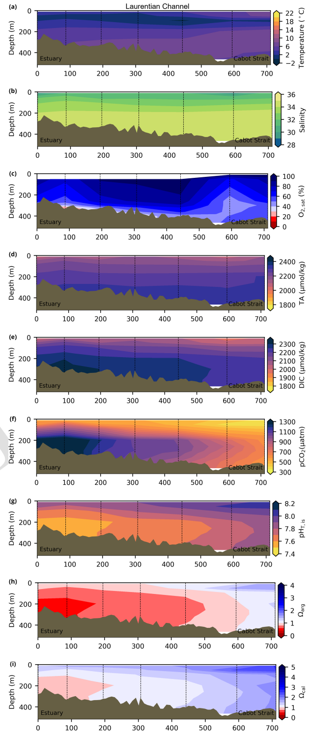
Figure B5. Same as in Fig. B1 but for the hydrographic section of the Laurentian Channel (GSL region; see Fig. 3 for location).
