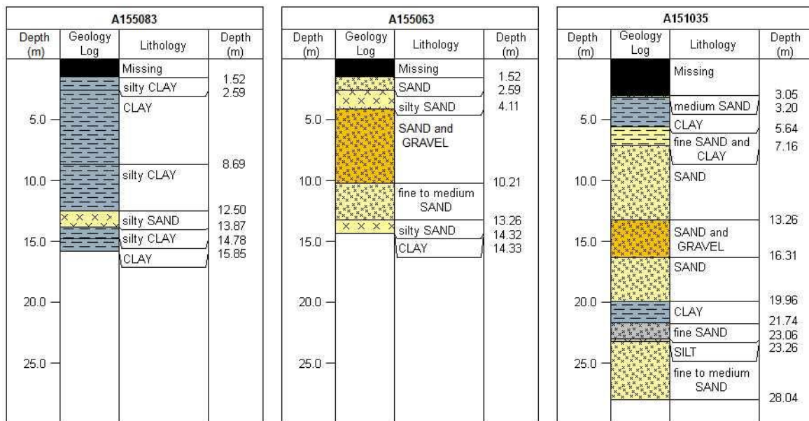
Figure 8: Deeper (> 10 m) borehole logs (Natural Environment Research Council, 2017). Splitspoon samples (length: 61 cm) were collected at the top of each 1.52 m interval and then interpolated and summarized to produce these logs.
