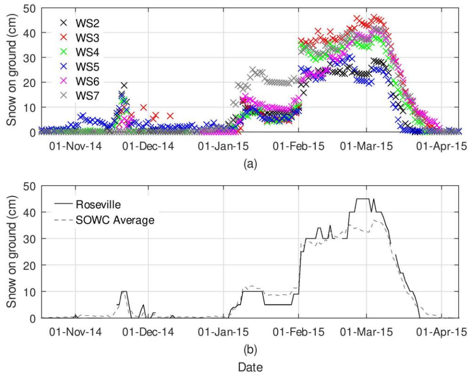
Figure 6: Snowpack thickness data (a) for individual Southern Ontario Water Consortium (SOWC) stations WS2 – WS7 (Wiebe et al., 2019), and (b) for the average from the SOWC stations and for Roseville (Government of Canada, 2019) for the 2014 to 2015 winter season (adapted from Wiebe, 2020). The average snowpack thicknesses are generally close to the Roseville weather station records, suggesting that uniform snowfall may be a reasonable assumption for the Alder Creek watershed.
