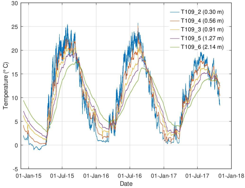
290 Figure 12: Average daily soil temperatures (Wiebe et al., 2019) at five depths beneath the base of a topographic depression at the Mannheim site.
