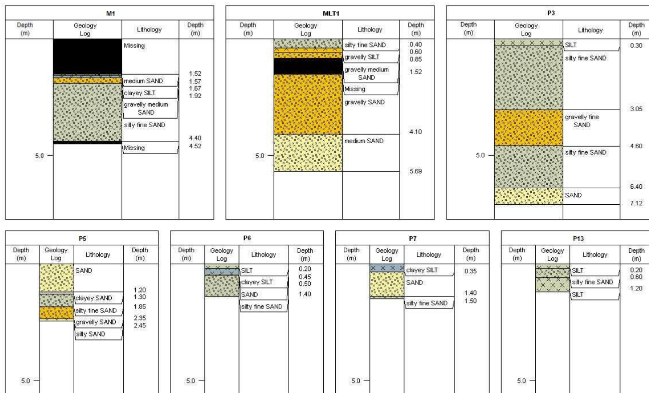
Figure 9: Shallow (< 10 m) borehole logs (NERC, 2017). The borehole logs for M1, MLT1, and P3 were based on the analysis of cores (length: 1.52 m) from a continuous coring method (7720DT GeoProbe®), while the borehole logs for P5, P6, P7, and P13 were based on analysis of a continuous series of samples (length: about 15 cm) collected with a hand auger.
