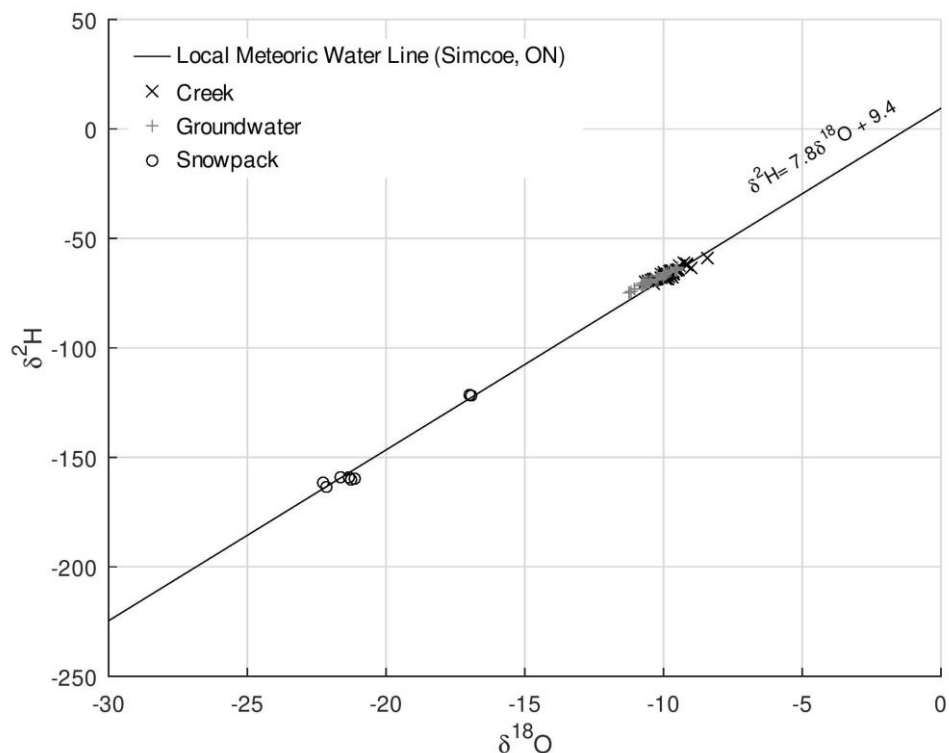
Figure 18: Isotope data from the watershed (Wiebe et al., 2019; local meteoric water line from Bajc et al., 2018). Groundwater and creek results coincide and show a contrast from snowpack results, suggesting that recharge is mostly derived from rainfall.
