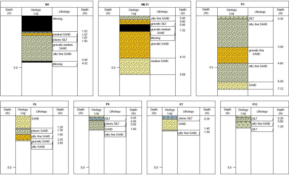
245 Figure 9: Shallow (< 10 m) borehole logs (NERC, 2017). The borehole logs for M1, MLT1, and P3 were based on the analysis of cores (length: 1.52 m) from a continuous coring method (7720DT GeoProbe®), while the borehole logs for P5, P6, P7, and P13 were based on analysis of a continuous series of samples (length: about 15 cm) collected with a hand auger.
