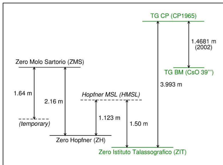
10 Figure 5: The relationships between the tide-gauge Zeros and their connections to the tide-gauge contact point (TG CP) and benchmark (TG BM).
