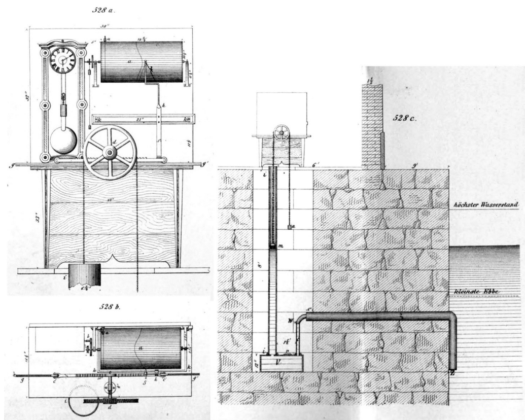
Figure 2: The tide gauge installed in 1859. View of the instrument from the front (528a) and from above (528b); vertical section of the northwest end of the building hosting the tide gauge and the stilling well (528c). Mean high and low waters are indicated by ‘höchster Wasserstand’ and ‘kleinste Ebbe’, respectively. The figures are adapted from Chiolich-Löwensberg (1865; 1866).
