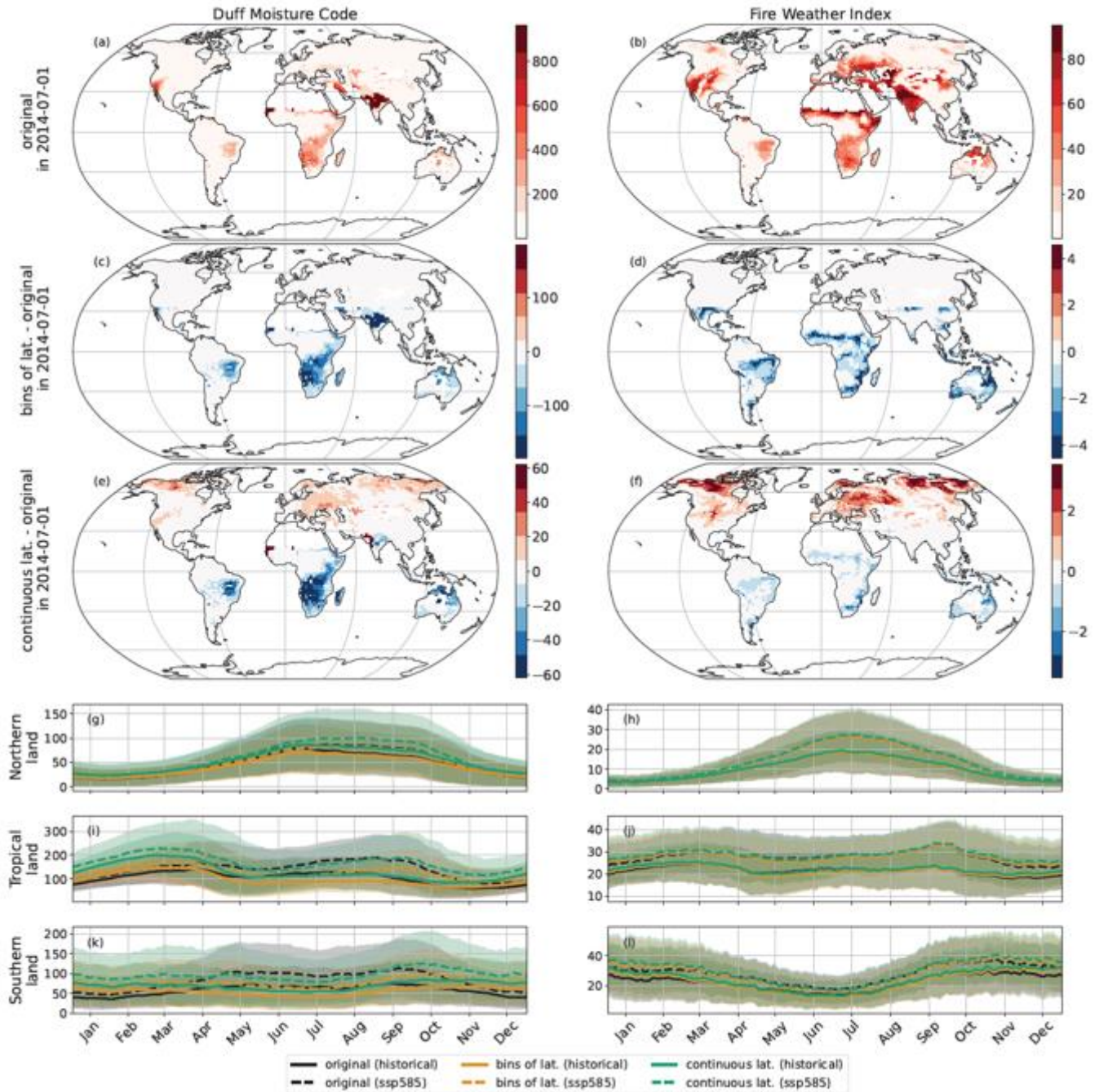
Figure 3. Sensitivity to the day length factor of ACCESS-CM2 in the experiments historical and ssp585 over the ensemble member r1i1p1f1 . The first row of maps (a & b) shows the values of the DMC and the FWI, the first and final indices affected by this factor, in the original version of the algorithm (Wang et al., 2015). The following maps (c to f) show the differences
