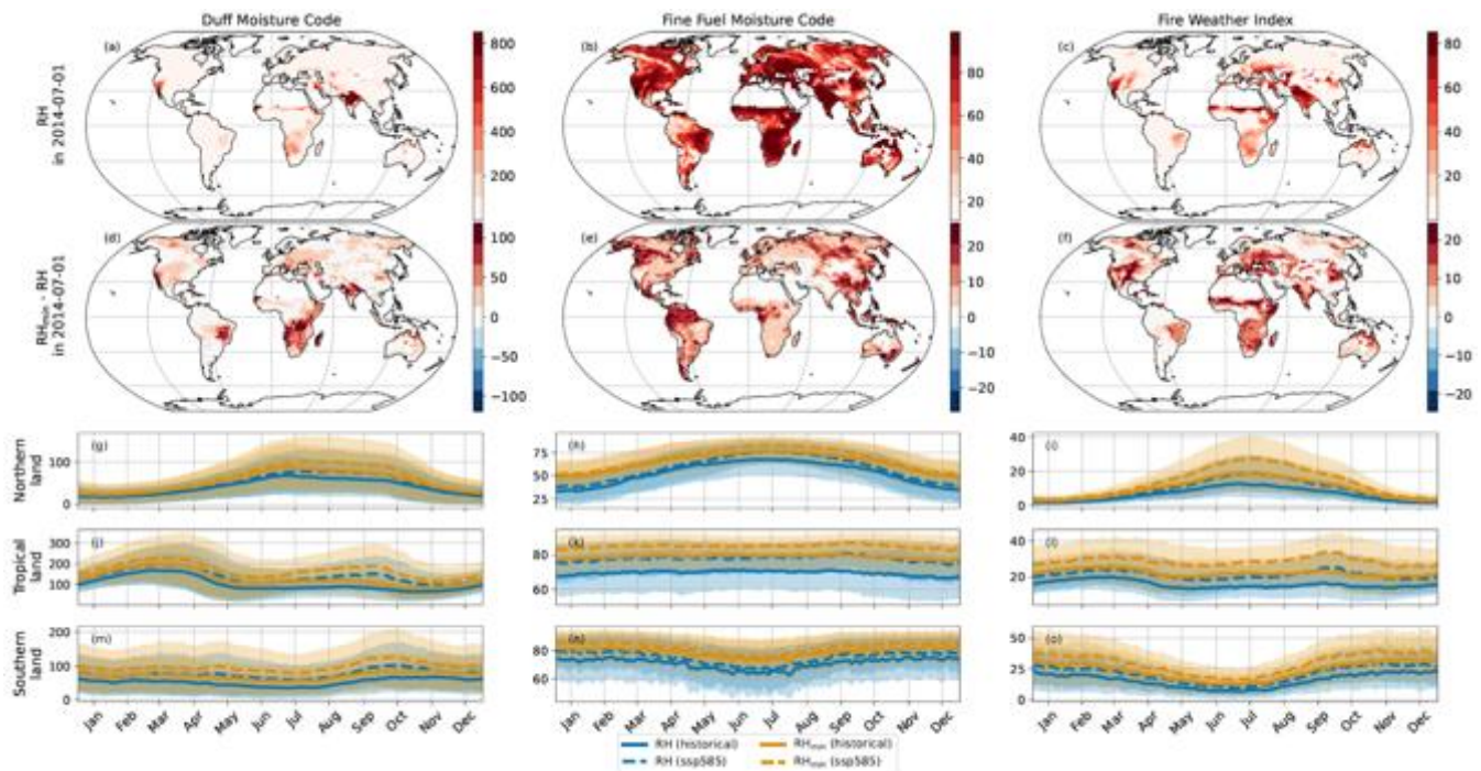
340 Figure 6. Sensitivity to the variable used for daily relative humidity of ACCESS-CM2 in the experiments historical and ssp585 over the ensemble member r11p1f1. The first row of maps (a to c) shows the values of the DMC, the FFMC and the FWI, the first and final indices affected when run with daily average relative humidity. The following maps (d to f) show the differences when run with daily minimum relative humidity. The following rows show the daily climatologies over 1995-2014 and 2081-2100, represented in terms of average and \pm 1 standard deviation range. The Northern land (g to i) is defined as grid cells over 20°N and not marked as infrequent burning. Similarly, Southern land (j to l) is below 20°S and Tropical land (m to o) is the intermediate latitude band.
