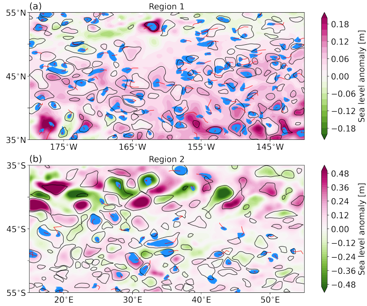
Figure 7. Locations of 30-day RCLVs (blue dots) and SSH eddies (>30 days, black contours) in (a) region 1 (blue box in Figure 6a) and (b) region 2 (red box in Figure 6a) on 1 January 2009. The red lines are the center trajectories of the RCLVs, and the color map represents the SLA field.
