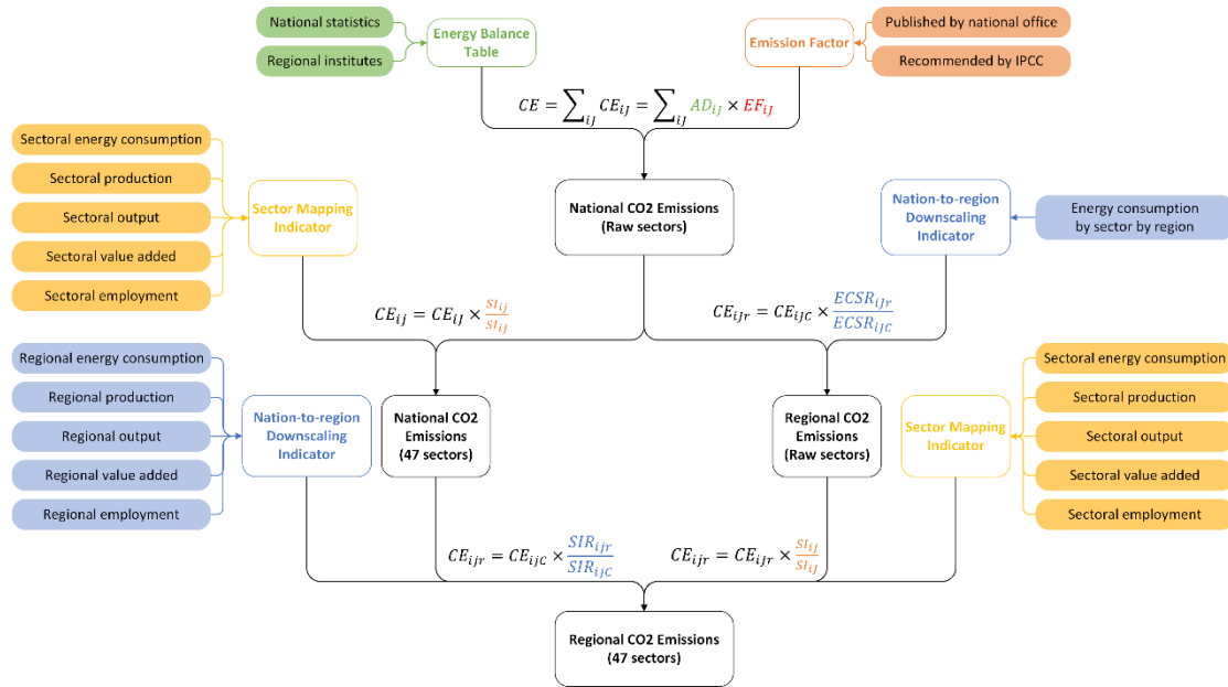
Figure 1: Overview of CO 2 emissions data collection and compilation. Blocks in color show the data sources for each step in the process. Blocks outlined in black show the phased calculated using the adjacent equations. Explanations of the Equations 1-5 are elaborated in detail in the Methods section.
