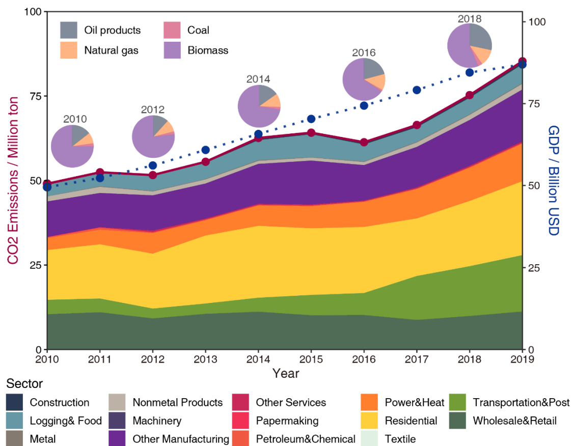
290 Figure 3: CO 2 emissions of Myanmar over 2010–2019. The red line shows the growth of CO 2 emissions; the blue dotted line charts the growth of GDP. The pie charts show CO 2 emissions by energy source; the area plot, CO 2 emissions by sector (17 sector aggregates merged from 47 sectors: see Table S4 in Supplemental Information for details).
