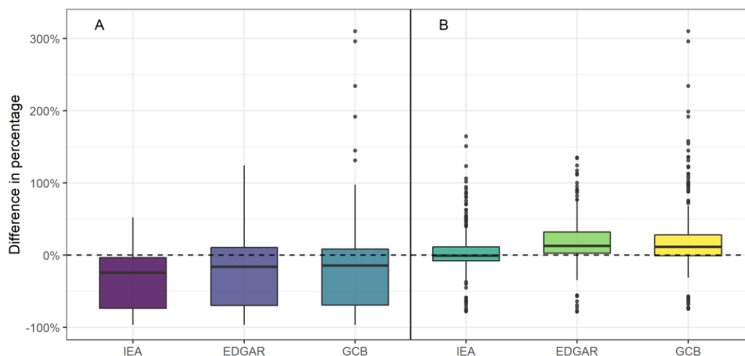
365 Figure 6: Disparities between the published data of three institutes (IEA, EDGAR and GCB) and the CEADs inventory with (A) and without (B) biomass emissions. The boxplots show the minimum, the first quartile, the median, the third quartile and the maximum of the differences across the nation-year emissions data among the institutes. The percentages are the relative difference between the three institutes and CEADs. For instance, (A) shows that emissions data from IEA, EDGAR and GCB are generally lower than those in the CEADs inventory, while (B) shows that the data from these three institutes are close to the CEADs inventory when biomass emissions are excluded from it.
