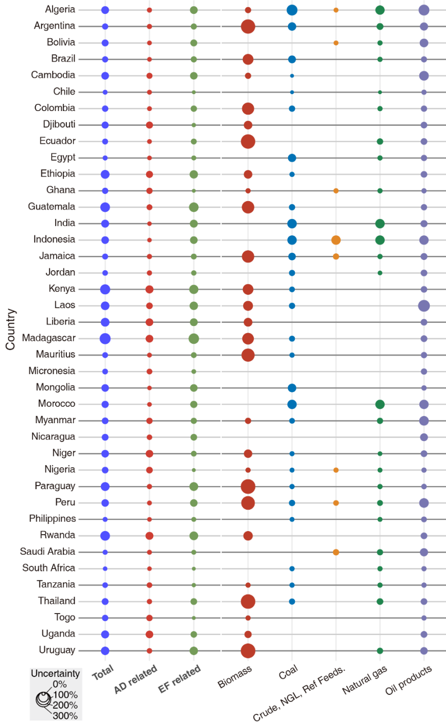
380 Figure 5: Data uncertainty of total emissions, from activity data, from emission factors, and by energy groups. CEADs collects energy consumption data from the energy balances of national energy bureaus, statistical offices, and regional institutes. Although the energy data are derived from national official statistics, there is significant variation in basic data from the 40 emerging economies. Mongolia and Djibouti, for instance, do not provide energy data for detailed sectors; thus their allocation
