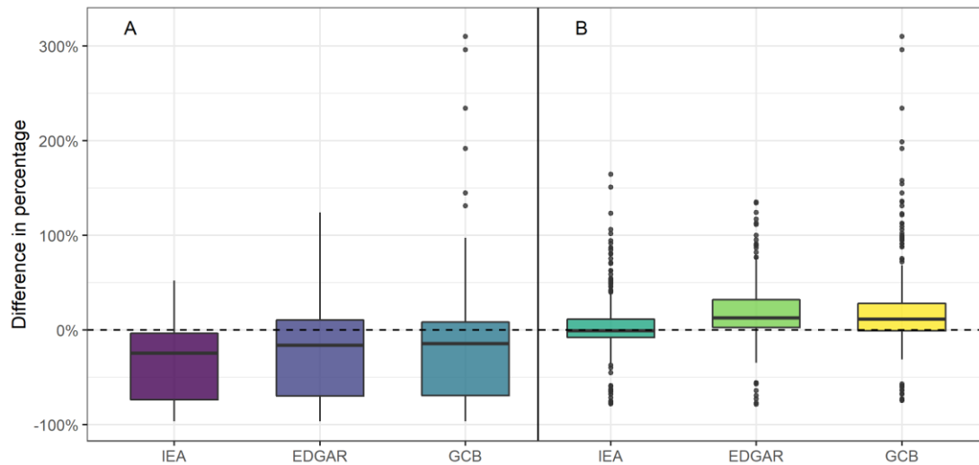
410 Figure 6: Disparities between the published data of three institutes (IEA, EDGAR and GCB) and the CEADs inventory with (A) and without (B) biomass emissions. The boxplots show the minimum, the first quartile, the median, the third quartile and the maximum of the differences across the nation-year emissions data among the institutes. The percentages are the relative difference between the three institutes and CEADs. For instance, (A) shows that emissions data from IEA, EDGAR and GCB are generally lower than those in the CEADs inventory, while (B) shows that the data from these three institutes are close to the CEADs inventory when biomass emissions are excluded from it.
