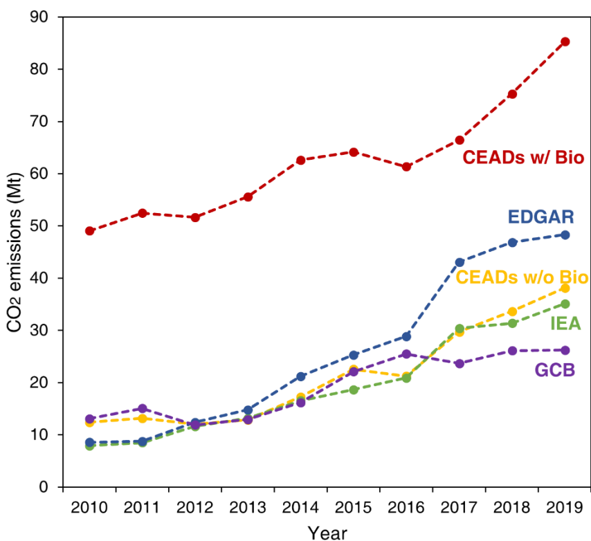
365 Figure 4: CO 2 emissions of Myanmar from different institutes, 2010-2019. Different colors represent the sourced datasets: red for CEADs with biomass emissions; blue for EDGAR; yellow for CEADs without biomass emissions; green for IEA; and purple for GCB.
