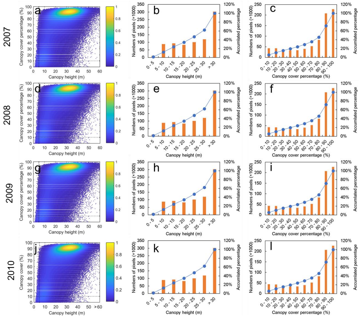
Fig. 4. Two-dimension scatter plots and histograms of ICESat/GLAS canopy height (m) and canopy coverage (%) at the footprint scale for the forest pixels in the annual PALSAR/MODIS forest cover maps during 2007-2010. Two-dimension scatter plots of ICESat/GLAS canopy height and canopy coverage for the forest pixels in the annual PALSAR/MODIS forest cover maps during 2007 (a), 2008 (d), 2009 (g), and 2010 (j). Histograms of ICESat/GLAS canopy height for the forest pixels in the annual PALSAR/MODIS forest cover maps during 2007 (b), 2008 (e), 2009 (h), and 2010 (k). Histograms of ICESat/GLAS canopy coverage for the forest pixels in the annual PALSAR/MODIS forest cover maps during 2007 (c), 2008 (f), 2009 (i), and 2010 (l).
