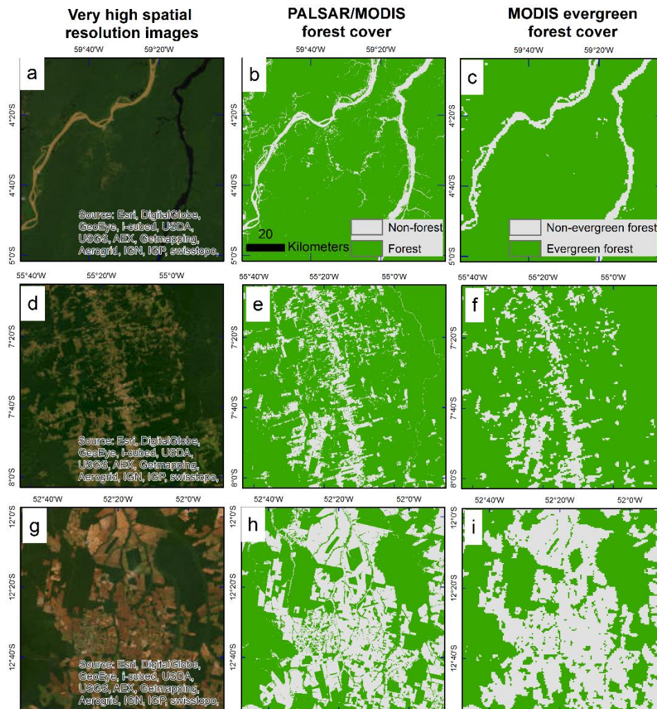
355 Fig. 8. Zoom-in windows of very high spatial resolution images, PALSAR/MODIS forest cover, and MODIS evergreen forest cover maps at three sites in the Brazilian Amazon. (a, d, and g) Very high spatial resolution images from ArcMap. (b, e, and h) PALSAR/MODIS forest cover maps. (c, f, and i) MODIS evergreen forest cover maps.
