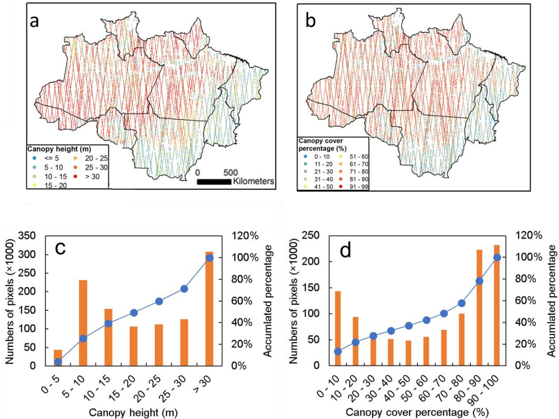
Fig. 1. Spatial distribution maps of ICESat-GLAS canopy height (a) and canopy coverage (b) at the footprint scale and their 185 histograms (c-d) in the Brazilian Amazon from 2003 to 2007.
