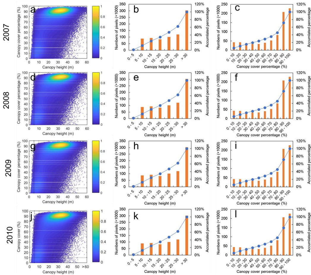
Fig. 4. Two-dimensional scatter plots and histograms of ICESat/GLAS canopy height (m) and canopy coverage (%) at the footprint scale for the forest pixels in the annual PALSAR/MODIS forest cover maps during 2007-2010. Two-dimensional scatter plots of ICESat/GLAS canopy height and canopy coverage for the forest pixels in the annual PALSAR/MODIS forest cover maps during 2007 (a), 2008 (d), 2009 (g), and 2010 (j). Histograms of ICESat/GLAS canopy height for the forest pixels in the annual PALSAR/MODIS forest cover maps during 2007 (b), 2008 (e), 2009 (h), and 2010 (k). Histograms of ICESat/GLAS canopy coverage for the forest pixels in the annual PALSAR/MODIS forest cover maps during 2007 (c), 2008 (f), 2009 (i), and 2010 (l).
