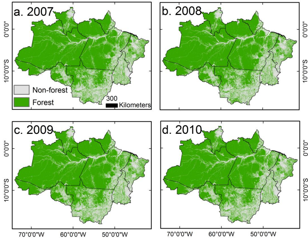
260 Fig. 3. Spatial distribution maps of annual PALSAR/MODIS forest cover maps during 2007 (a), 2008 (b), 2009 (c), and 2010 (d).
