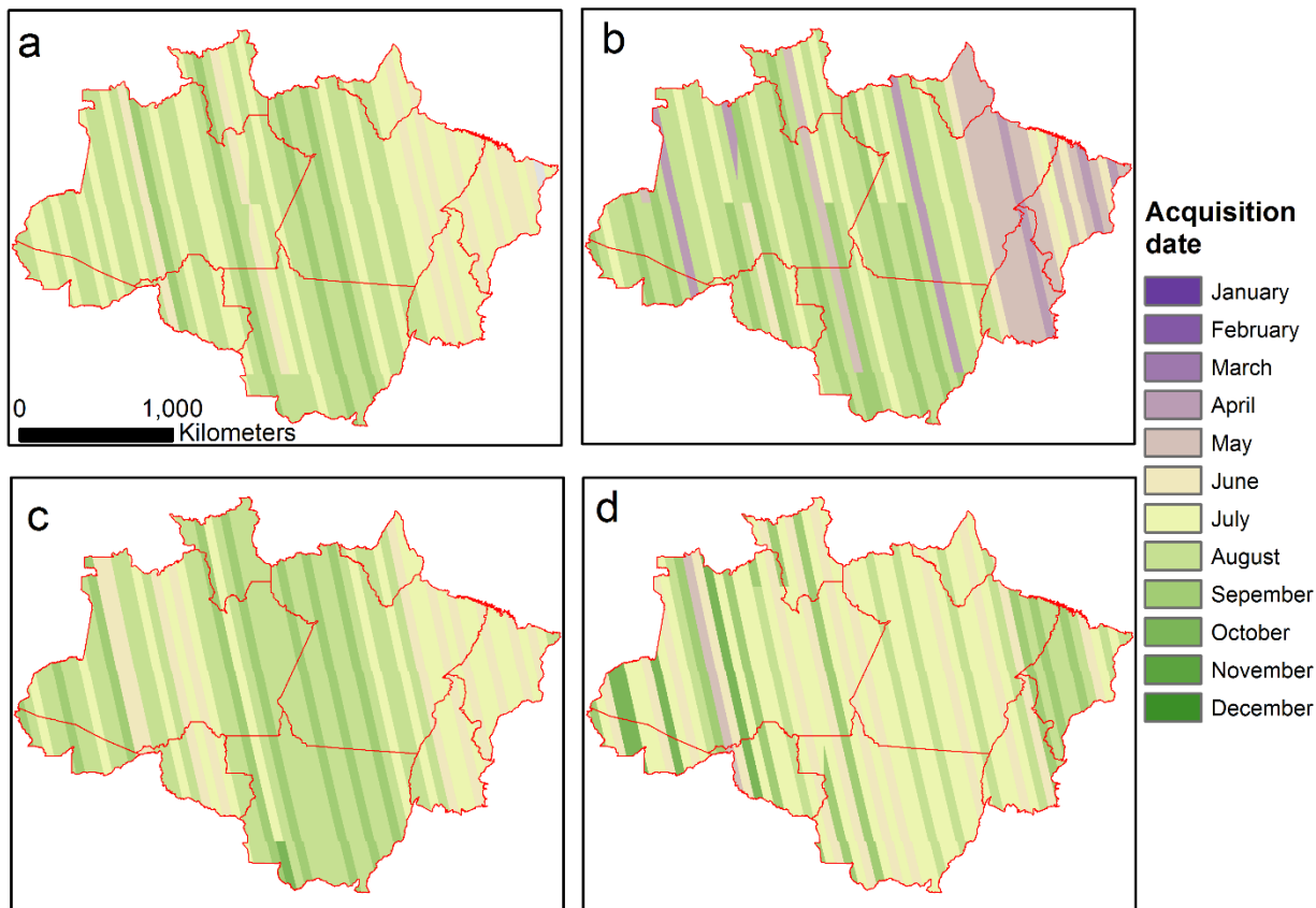
210 Fig. 2. Spatial distribution maps of ALOS PALSAR acquisition date during 2007 (a), 2008 (b), 2009 (c), and 2010 (d).
