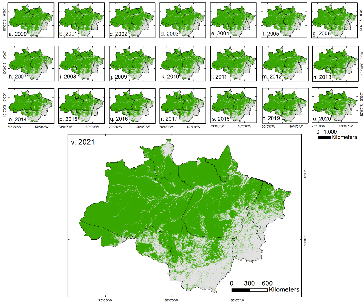
Fig. 5. Spatial distribution maps of annual MODIS evergreen forest cover maps in the Brazilian Amazon during 2000-2021.
