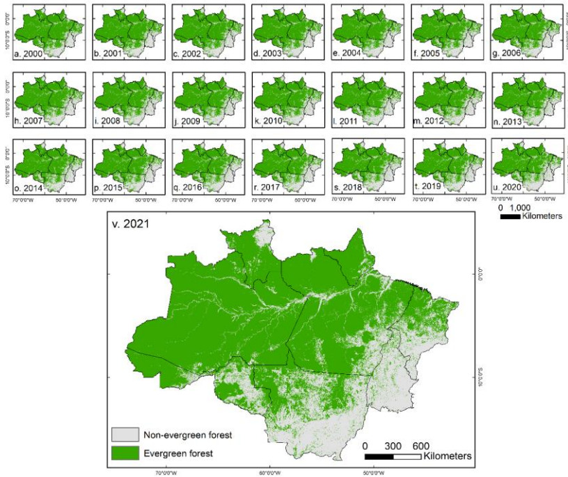
Fig. 5. Spatial distribution maps of annual MODIS evergreen forest cover maps in the Brazilian Amazon during 2000-2021.
