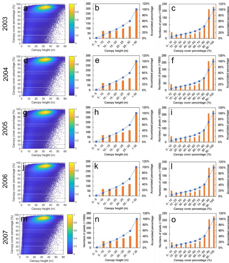
Fig. 6. Two-dimensional scatter plots and histograms of ICESat/GLAS canopy height (m) and canopy coverage (%) for the forest pixels from the annual MODIS evergreen forest maps during 2003-2007. Two-dimensional scatter plots of ICESat/GLAS canopy height and canopy coverage for the forest pixels from the annual MODIS evergreen forest maps during 2003 (a), 2004
