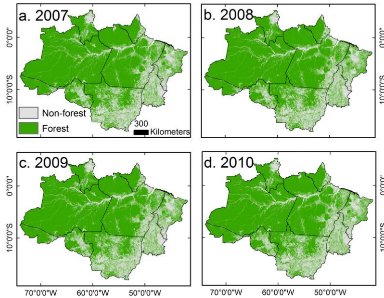
275 Fig. 3. Spatial distribution maps of annual PALSAR/MODIS forest cover maps during 2007 (a), 2008 (b), 2009 (c), and 2010 (d).
