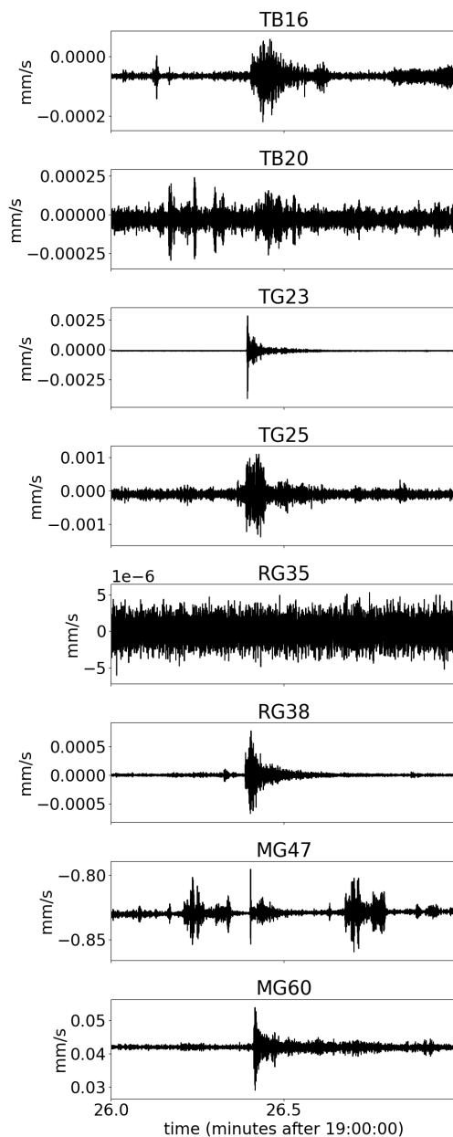
Figure 5. Traces on network stations recording on 05.05.2022. Traces are filtered between 10 Hz and 50 Hz around time of detected and located event in Eschweiler (308894 m Easting, 5629087 m Northing, close to station RG38) at 05.05.2022, 19:26:21.7 with a magnitude of ML1.1 (Earthquake Observatory Bensberg University Cologne, 2022)
