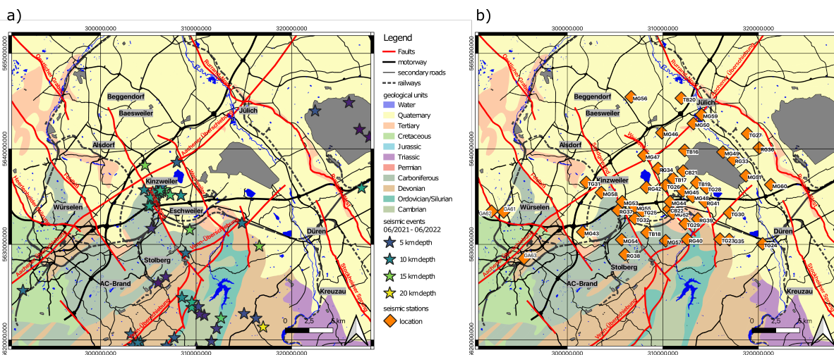
Figure 1. Study area in western Germany with major faults, roads and railways overlain on geological map (GD NRW, 2022). a) Seismic event locations as reported by Earthquake Observatory Bensberg University Cologne (2022) from June 2021 to June 2022. b) Station locations of the Weisweiler network are marked with squares.
