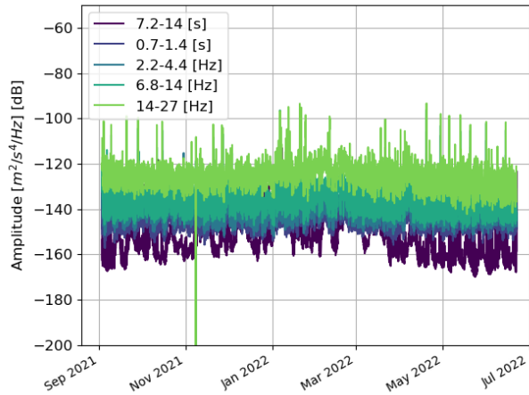
Figure 4. Temporal trend of PSD for selected frequencies created using obsSpy-ObsPy (Beyreuther et al., 2010) for the z component of station TG23.
