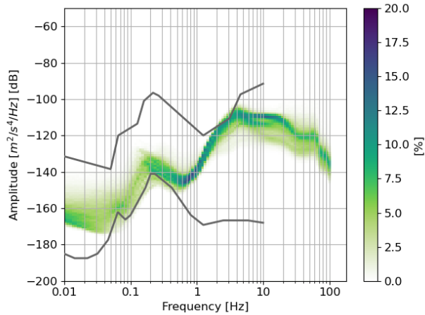
Figure 2. Probabilistic Power Spectral Density (PSD) created using obspsy-ObsPy (Beyreuther et al., 2010) for the z component of station TG32 (Northeast, thicker sediments) for all recorded data. Grey lines show new low/high noise model (Peterson, 1993). This station has high noise levels.
