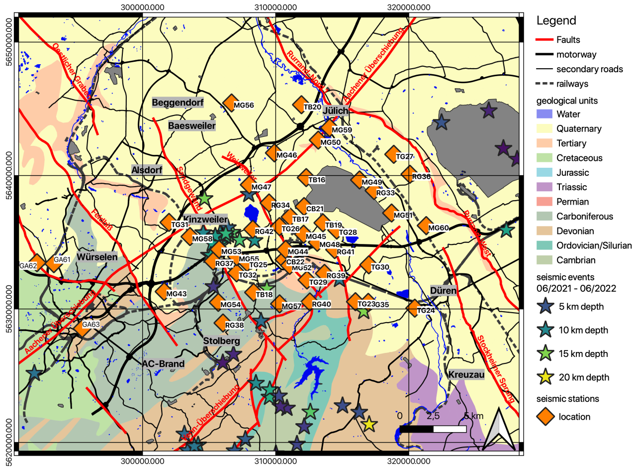
Figure 1. Study area in western Germany with major faults, roads and railways overlain on geological map (GD NRW, 2022) a) Seismic with seismic event locations as reported by Earthquake Observatory Bensberg University Cologne (2022) from June 2021 to June 2022. b) Station-2022 and station locations of the Weisweiler network are marked with squares.
