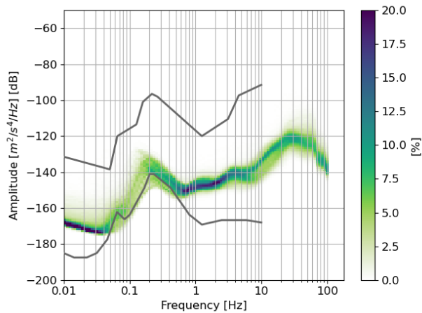
Figure 3. Probabilistic Power Spectral Density (PSD) created using obspsy-ObsPy (Beyreuther et al., 2010) for the z component of station TG23 (Southwest, thinner sediments) for all recorded data. Grey lines show new low/high noise model (Peterson, 1993). This station has overall the lowest noise levels.
