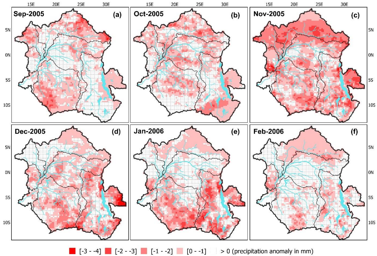
1185 Figure 12: Monthly mean spatial distribution of MSWEP precipitation anomaly in mm (resampled at 0.25° spatial resolution) from the period September 2005 to February 2006 based on the 1992-2015 climatology.
