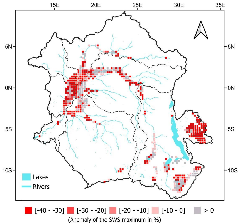
1180 Figure 11: The 2005-2006 drought over the CRB as seen from the hypsometric curve approach SWS dataset based on FABDEM. Anomaly of the maximum SWS over November 2005 to January 2006 as compared to the 1992-2015 November-December-January mean value. The unit is in percentage of the 24-years mean monthly value.
