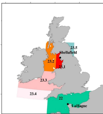
Figure 1: Boxes dividing the global ocean. (a) Global, (b) North Atlantic Ocean and its marginal Sea, and 220 (c) Irish Sea (Box23) and English Channel (Box22).
