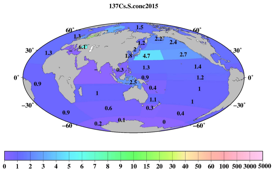
810 Figure 7: Horizontal distributions of the 0.5-yr median 137 Cs value in the surface mixed layer in the global ocean. The unit is Bqm -3 . (a) 1970, (b) 1975, (c) 1980, (d) 1985, (e) 1990, (f) 1995, (g) 2000, (h) 2005, (i) 2010, and (j) 2015.
