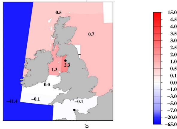
Figure 18: Horizontal distribution of the ^{137}\text{Cs} net in/outflow amount in each box against the deposition amount in 1970 based on the 0.5-year ^{137}\text{Cs} activity concentration data. The amount of ^{137}\text{Cs} net outflow includes the downwards transport portion below the surface mixed layer and horizontal transport in the surface mixed layer to the downstream boxes. A positive value (red) indicates the net inflow amount, and negative values (blue) indicate the net outflow amount. (a) Global ocean, (b) northern North Pacific Ocean and its marginal seas, (c) Irish Sea and English Channel. The unit is PBq.
