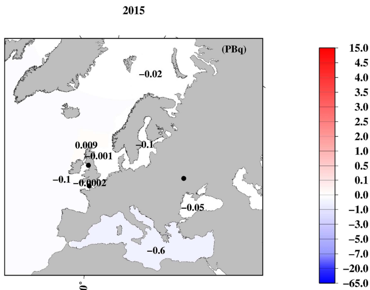
1615 Figure 20: Mass balance of ^{137}\text{Cs} in the surface seawater in each box in the northern North Atlantic Ocean and its marginal seas. A positive value (red) means the net inflowed ^{137}\text{Cs} from the upstream boxes, and a negative value (blue) indicates net outflowed ^{137}\text{Cs} to the downstream boxes or below the surface mixed layer compared to the previous 5 years. The unit is PBq. (a) 1975, (b) 1980, (c) 1985, (d) 1990, (e) 1995, (f) 2000, (g) 2005, (h) 2010, and (i) 2015.
