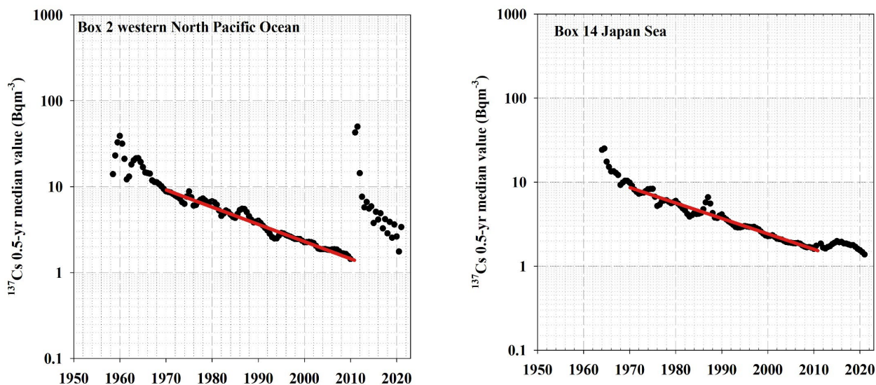
Figure 4: Temporal variation in the 0.5-yr median ^{137}\text{Cs} values. (a) Western North Pacific Ocean, (b) Japan Sea. The lines represent the exponential decay of the 0.5-yr ^{137}\text{Cs} median value between 1970 and 2010.
