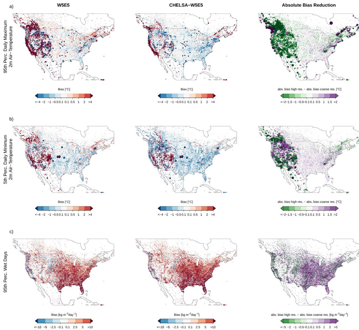
10 Figure 7: Mean bias of the extremes in maximum and minimum daily 2 m air temperatures and precipitation rates (from top to bottom) in North America averaged over the entire observational period of each station between 1979-2016. Left: Mean bias between W5E5 and observations from GHCN-D meteorological stations for extreme values in air temperature and precipitation. Middle: Bias between CHELSA-W5E5 and observations from GHCN-D meteorological stations for extreme values in air temperature and precipitation. Right: Absolute bias reduction after downscaling from 0.5° to 30 arcsec for extreme values in air temperature and precipitation, defined as the difference between the absolute bias of W5E5 and the absolute bias of CHELSA-W5E5. 15
