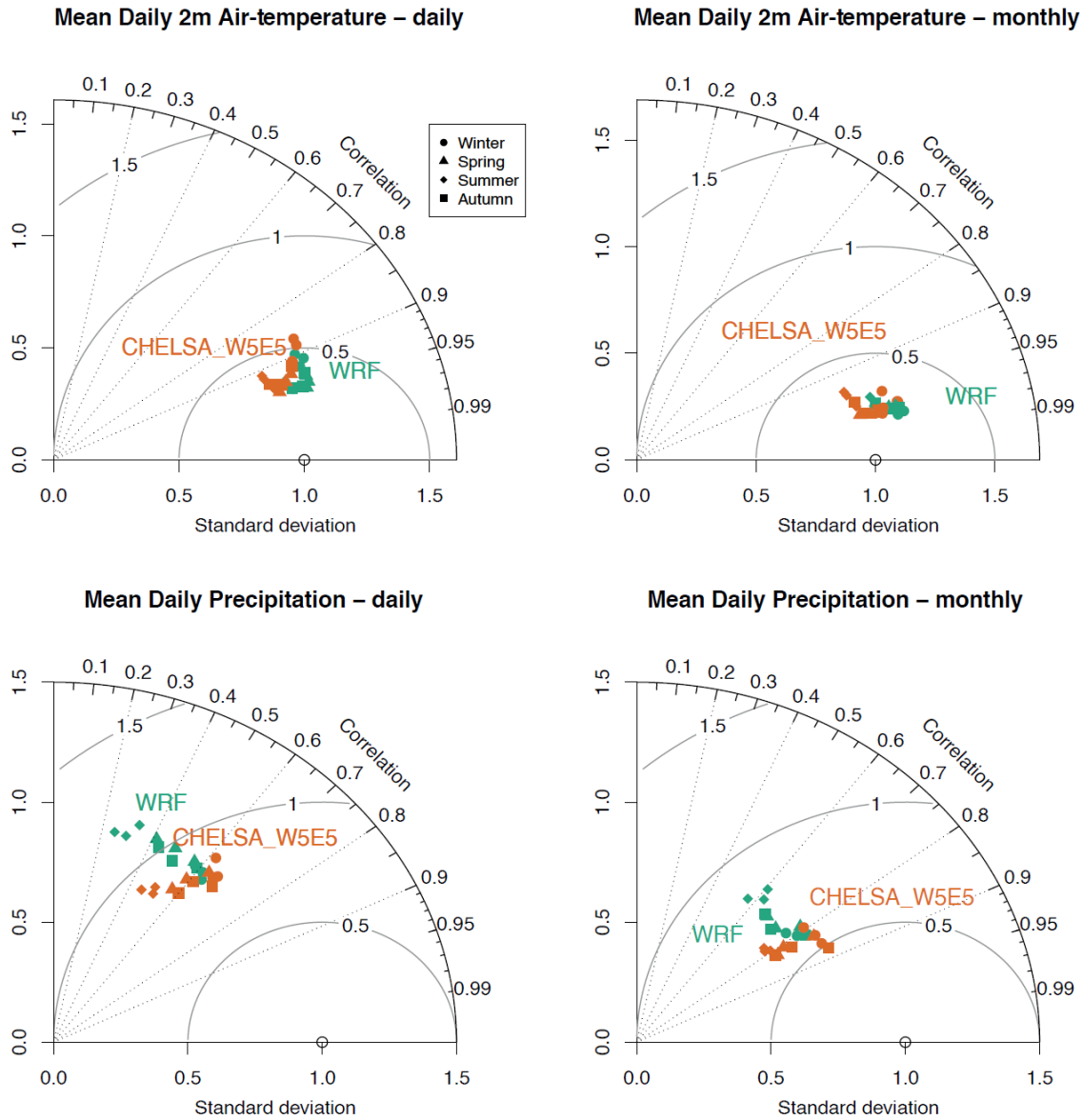
Figure 8: Performance based on a comparison of global long term monthly means of the topographically downscaled high-resolution (~1 km) data (CHELSA-W5E5, orange) with dynamically downscaled high-resolution (4 km) data (WRF, green) over North America, for the climatic variables daily mean 2 m air temperature and daily mean precipitation. The long-term means are shown separately for the four seasons; winter (DJF), spring (MAM), summer (JJA), autumn (SON).
