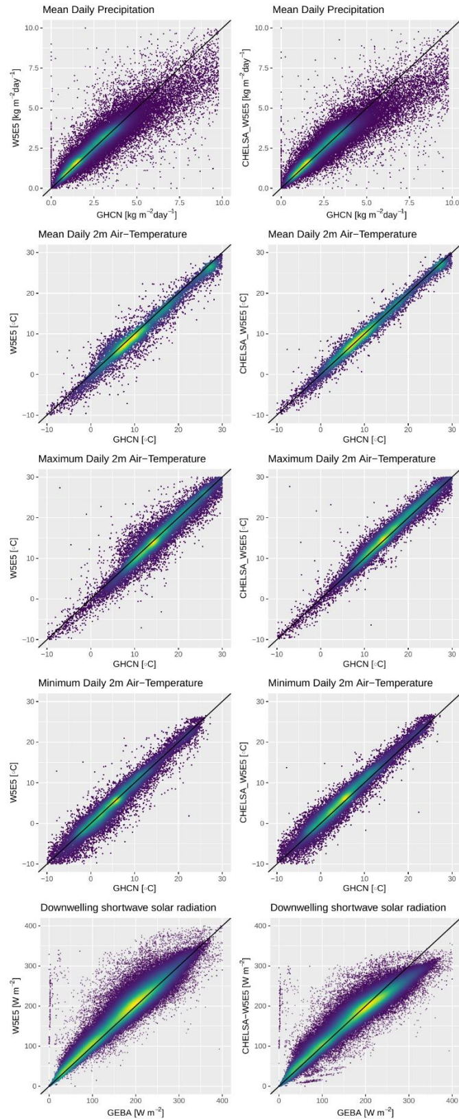
5 Figure 5: Scatterplots comparing long term mean observations from GHCN-D with values from W5E5 (left column, before downscaling), and CHELSA-W5E5 (right column, after downscaling). Each point represents the mean of all observations at a specific GHCN-D station in the period 1979-2016, except for downwelling shortwave solar radiation where each point represents a specific month.
