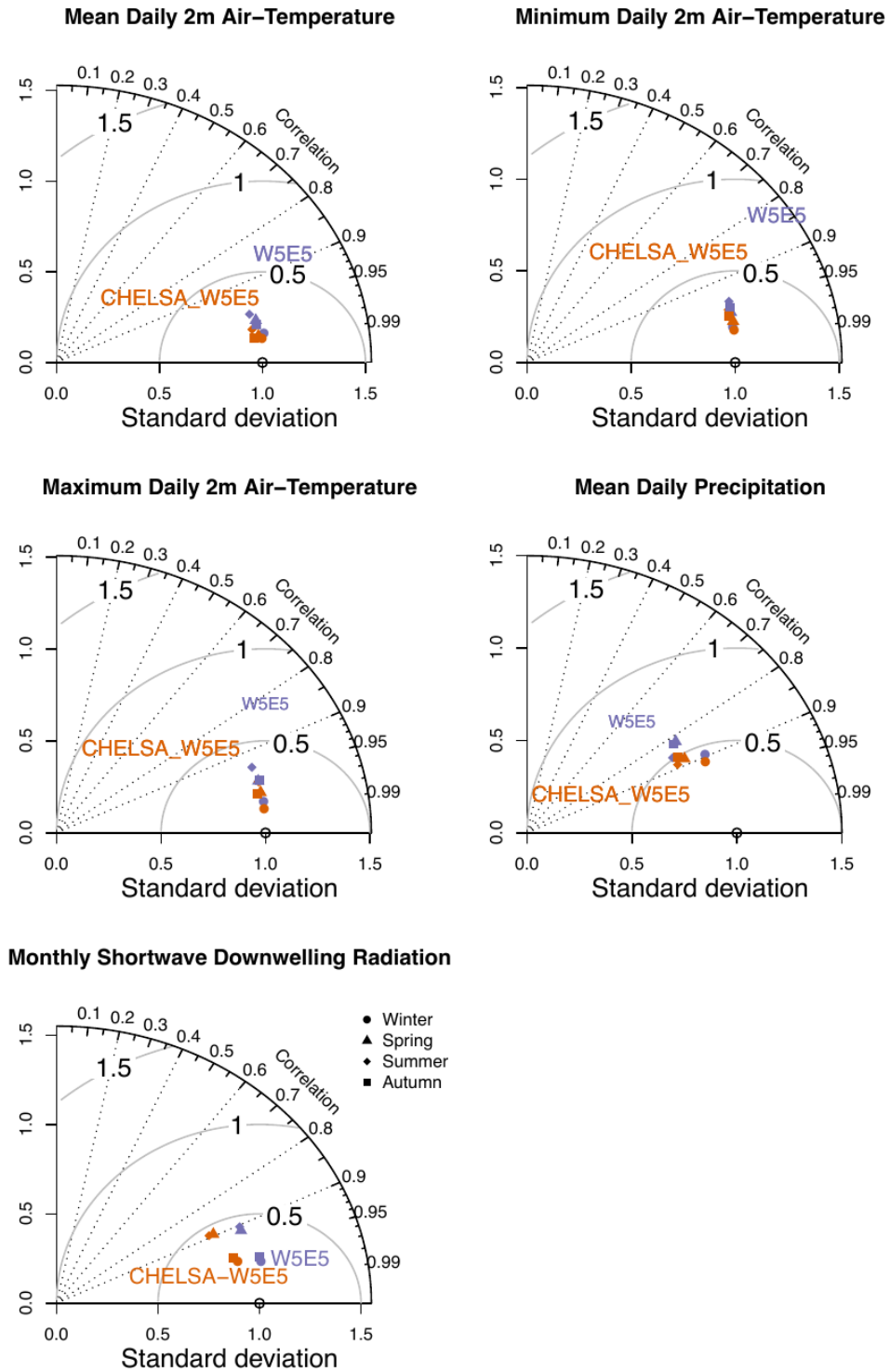
Figure 2: Seasonal performance based on a comparison of global long term seasonal means normals (1979-2016) of the global topographically downscaled high-resolution (30 arcsec, i.e. ~1 km) data (CHELSA-W5E5, orange) and the coarse (0.5°) original data (W5E5, violet) with GHCN-D for daily mean 2 m air temperature ( tas ), daily minimum 2 m air temperature ( tasmin ), daily maximum 2 m air temperature ( tasmax ), precipitation ( pr ), and shortwave downwelling radiation ( rsds ), based on monthly aggregated data. Values are shown separately for the four seasons: winter (DJF), spring (MAM), summer (JJA), autumn (SON). For the variables tas , tasmin , tasmax , and pr , the observational dataset GHCN-D was used for comparison. For rsds , the GEBA dataset was used.
