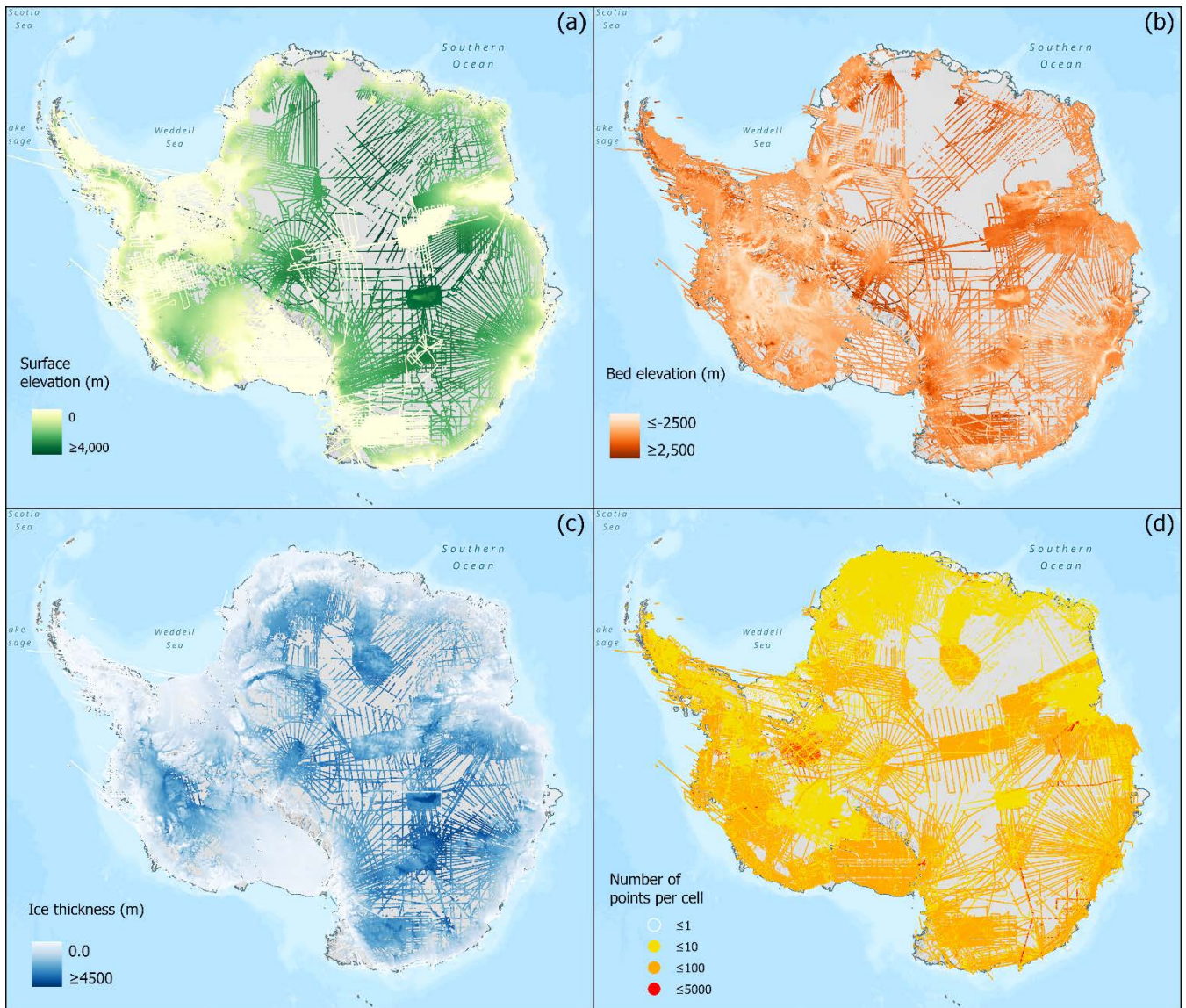
300 Figure 3 Statistically-summarised data points. (a) Mean surface elevation in meters over Antarctica. (b) Mean bed elevation in meters over Antarctica. (c) Mean ice thickness in meters over Antarctica. (d) Number of points per cell used for the calculation of ice thickness. All elevation values in (a-b) are given with reference to the WGS84 ellipsoid.
