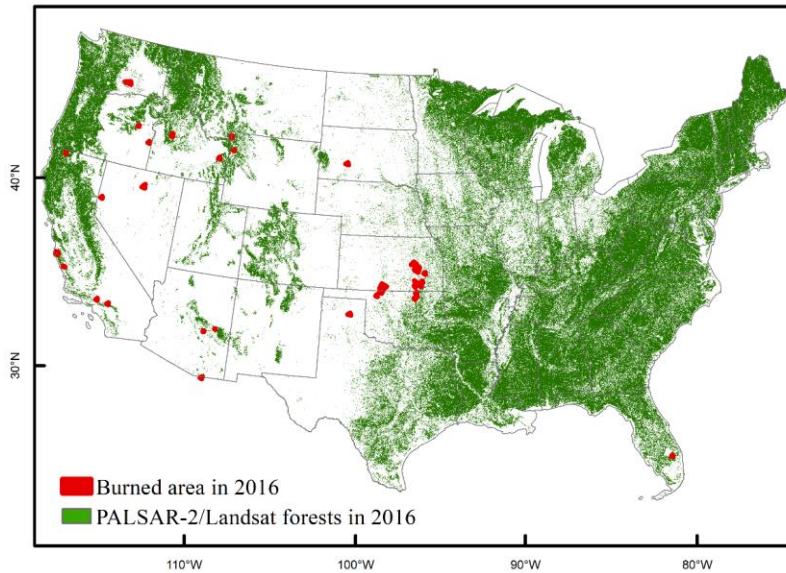
440 Figure 8: Distribution of burned area overlaid with the PALSAR-2/Landsat forests in 2016. The burned area in 2016 was generated from the MODIS Burned Area Monthly Global 500m products (MCD64A1.061). If a pixel was burned in any month, the pixel was considered a burned area in 2016.
