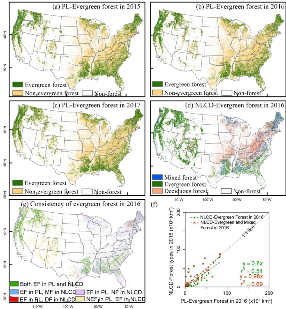
465 Figure 98: Spatial distributions of evergreen forests in the CONUS. (a, b, c) Annual evergreen and non-evergreen forest maps generated from the PALSAR-2/Landsat (PL) images in 2015-2017. (d) The forest-type map from the National Land Cover Database (NLCD) in the 2016 dataset. (e) shows the consistency between the PALSAR-365-2/Landsat evergreen forest (PL-Evergreen forest) in 2016 and the NLCD-Evergreen forest in 2016 (NLCD-Evergreen). The abbreviations are Evergreen Forest (EF), PL-Evergreen Forest in 2016 (PL), Mixed Forest (MF), Non-Forest (NF), Deciduous Forest (DF), and Non-Evergreen Forest (NEF). (f) shows the comparison between PL-Evergreen forest and NLCD-Evergreen and NLCD-Evergreen and mixed forest in 2016 at the state scale using the linear regression analysis. 470
