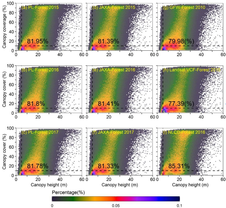
495 Figure 110: The frequency distributions of the forest pixels with tree canopy height (CH) and canopy cover (CC) features. The forest pixels were from the five satellite-based forest products, respectively. The CH and CC data were extracted from the ICESat-1 observations. PL-Forest is PALSAR-2/Landsat-based forest maps generated in this study. JAXA-Forest is the Japan Aerospace Exploration Agency (JAXA) forest map from 2015 to 2017. GFW-Forest 2010 is the forest map 2010 from the Global Forest Watch (GFW) program of the World Resources Institute. Landsat VCF-Forest 2015 is the Landsat-based forest cover fraction (Landsat VCF) product 2015 from the Global Land Cover Facility Data Center at the University of Maryland. The NLCD-Forest 2016 refers to the forest map from the National Land Cover Database (NLCD) in 2016 provided by the United States Geological Survey.
