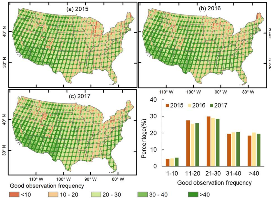
Figure 3: The summary of the good-quality observation (GOBs) numbers for individual pixels in a year over the CONUS using all Landsat images in a year from 2015 to 2017.
