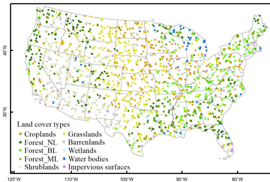
240 Figure 4: The land cover samples for accuracy assessment in this study. These samples were from the global validation sample set released by the third-party researchers from Tsinghua University, China ( http://data.ess.tsinghua.edu.cn/ , last access: 20 February 2022) (Gong et al. 2013). They were revised by excluding the samples with land cover change according to the Google Earth images. Forest_NL, Forest_BL, and Forest_ML denote needle-leaved forest, broad-leaved forest, and mixed-leaved forest, respectively.
