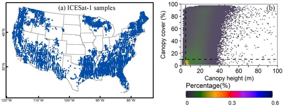
270 Figure 5. The ICESat samples in the CONUS, (a) Spatial distribution of ICESat-1 samples. (b) the histogram of canopy height (m) and canopy coverage (%) for the ICESat-1 samples.
