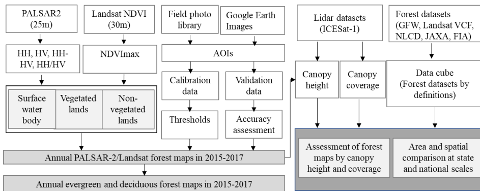
Figure 1: The workflow of this study. It includes three major study sections and the detailed processes of each section in this study. GFW, Landsat VCF, NLCD, JAXA, and FIA present different forest cover datasets that have been released. HH, HV, HH-HV, and HH/HV denote the horizontal-horizontal (HH) and horizontal-vertical (HV) polarization bands, and two
