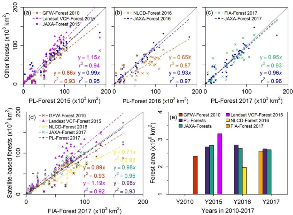
Figure 12-1: The comparisons of forest area estimates between satellite-based forest products and the FIA statistics at the state and national scales. PL-Forest is the PALSAR-2/Landsat-based forest map generated in this study. JAXA-Forest is the Japan Aerospace Exploration Agency (JAXA) forest map from 2015 to 2017. GFW-Forest 2010 is the forest map in 2010 from the Global Forest Watch (GFW) program of the World Resources Institute. Landsat VCF-Forest 2015 is the Landsat-based forest cover fraction (Landsat VCF) product in 2015 from the Global Land Cover Facility Data Center at the University of Maryland. The NLCD-Forest 2016 refers to the forest map from the National Land Cover Database (NLCD) in 2016 provided by the United States Geological Survey. FIA-Forest 2017 presents the forest cover datasets from the Forest Inventory and Analysis (FIA) program in 2017.
