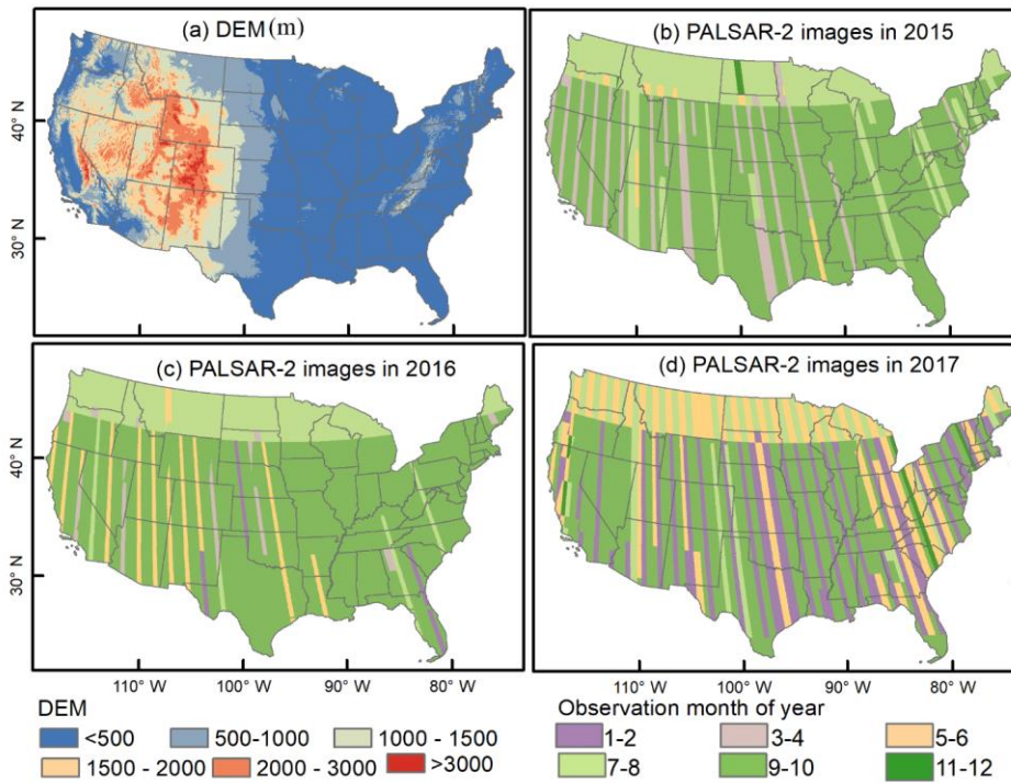
Figure 2: The spatial distributions of (a) the topography of the CONUS using the digital elevation model (DEM), data from the U.S. Geological Survey, 3D Elevation Program 10-Meter Resolution Digital Elevation Model (DEM). (b, c, d) the acquisition dates of PALSAR-2 images in a year during 2015 - 2017.
