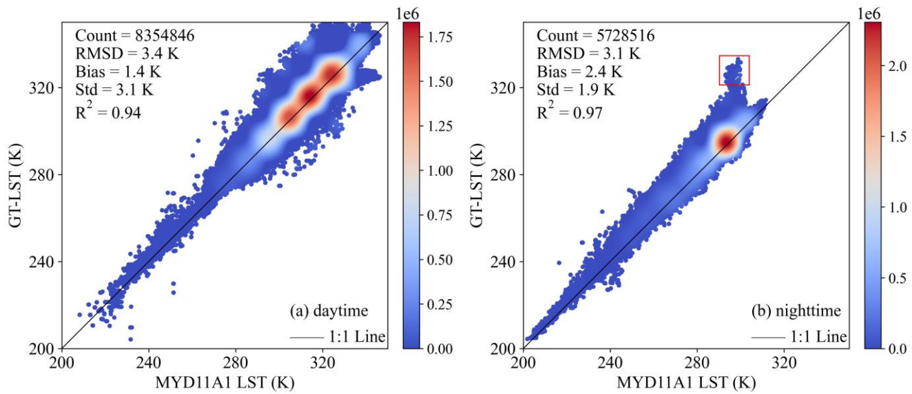
790 Figure 6: Inter-comparison of GT-LST and MYD11A1 LST in 2004: (a) daytime; (b) nighttime.
