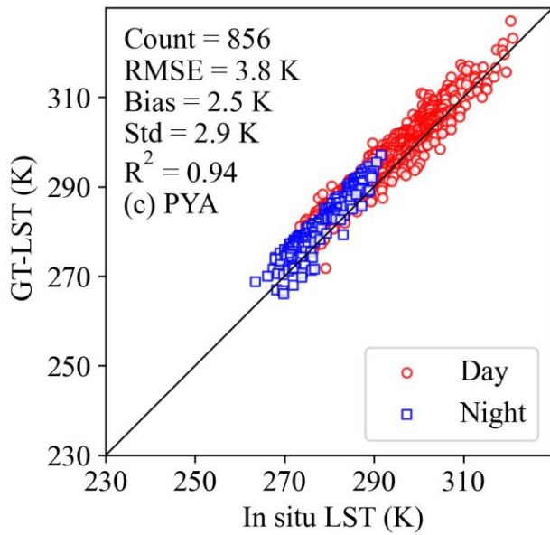
785 Figure 5: Scatterplots between GT-LST and in situ LST at (a) BAR, (b) NYA, (c) PYA, and (d) TAT.
