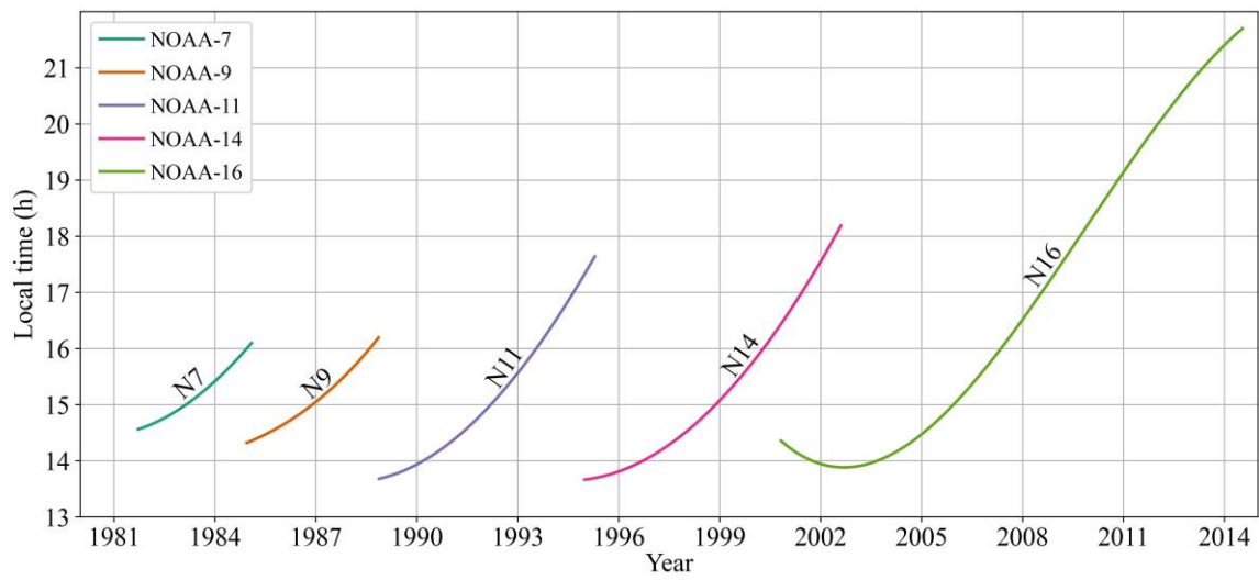
Figure 15: Equatorial crossing time of NOAA afternoon satellites (Adapted from https://www.star.nesdis.noaa.gov/smcd/emb/vci/VH/vh_avhrr_ect.php ).
