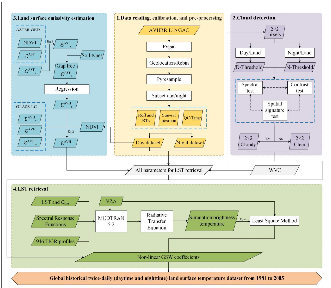
780 Figure 3: Schematic of the workflow used to generate the GT-LST product.
