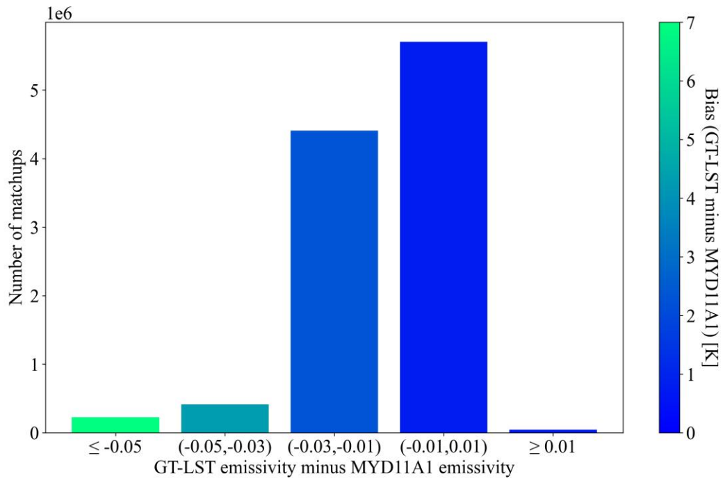
515 Figure A3: Difference between GT-LST and MYD11A1 LST stratified by the difference between GT-LST and MYD11A1 emissivity (water vapor content < 5 g cm -2 ; satellite zenith angle < 50°).
