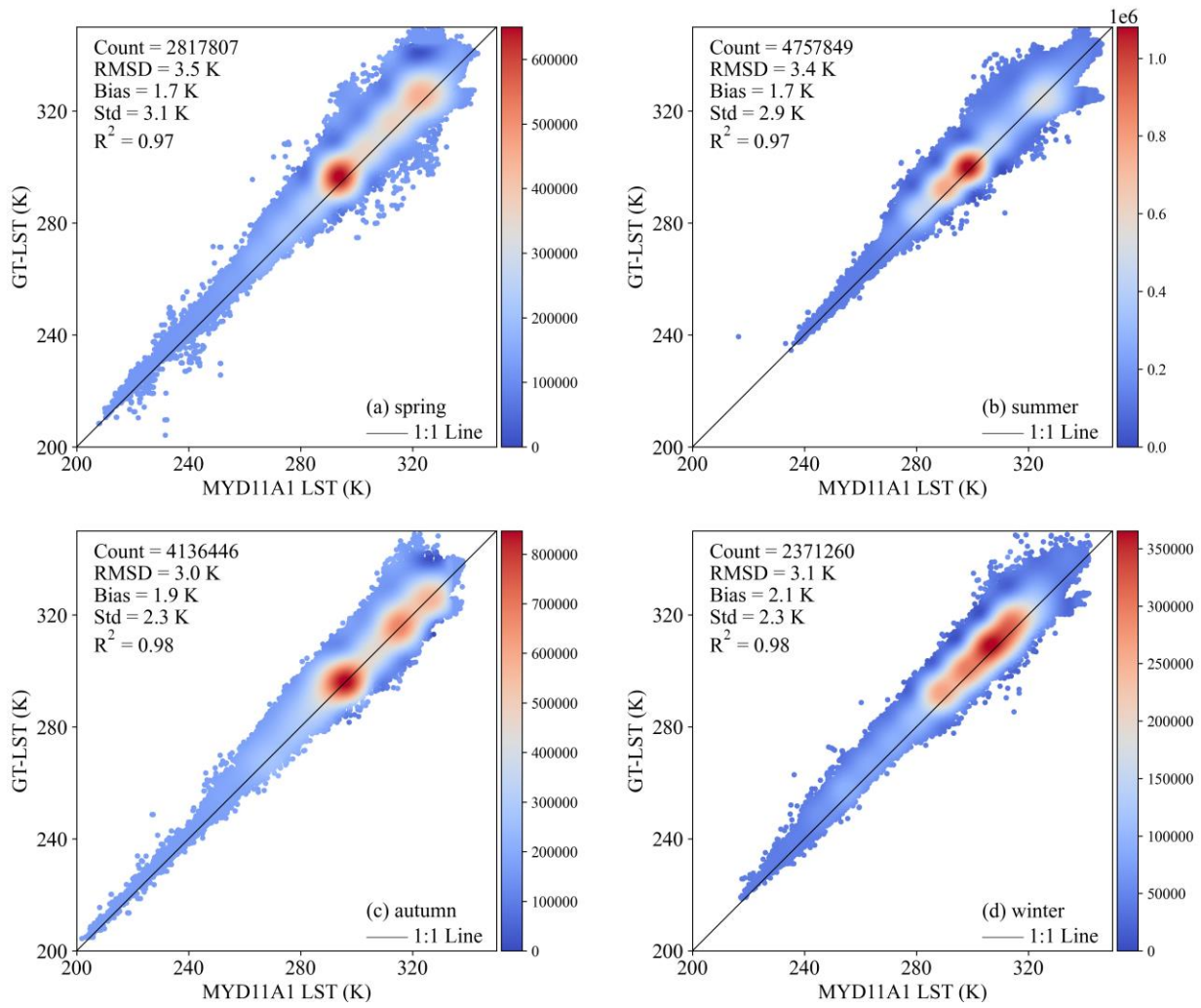
800 Figure 8: Inter-comparison of GT-LST and MYD11A1 LST in 2003: (a) spring; (b) summer; (c) autumn; (d) winter.
