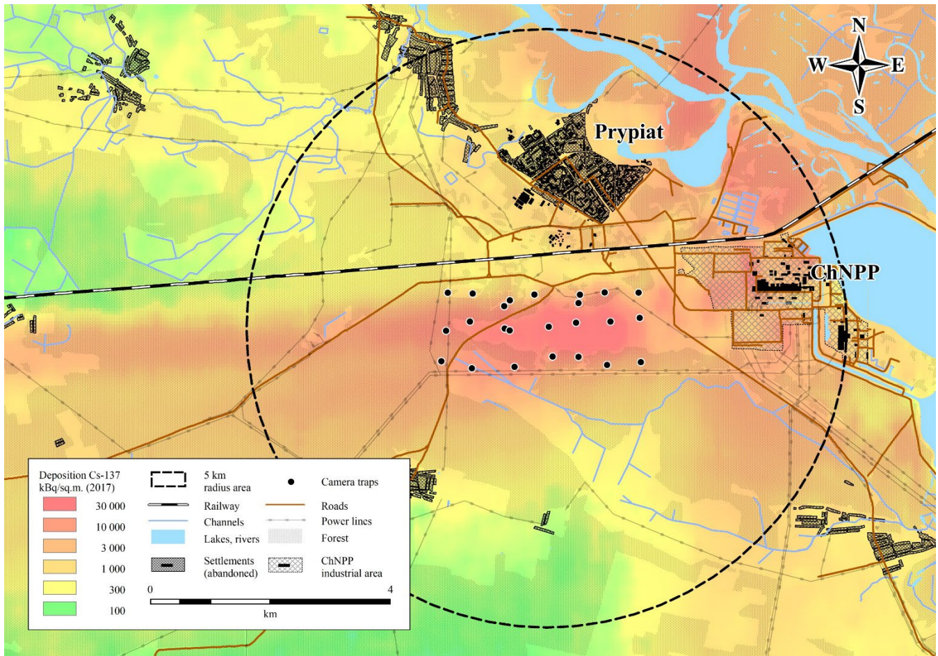
60 Figure 1: Map showing the location of the study cameras overlaid on a ^{137}\text{Cs} deposition surface (decay corrected to 2017). The large circle is the 5 km radius area over which absorbed weighted dose rates were calculated. Figure produced by and published with the permission of the Chernobyl Center.
