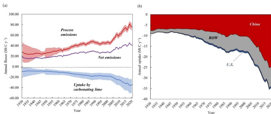
Figure 3: (a) Net lime emissions from 1930 to 2020. Shadows represent uncertainty ranges. (b) Annual uptake of carbon dioxide by lime in different regions. ROW: Rest of World.
