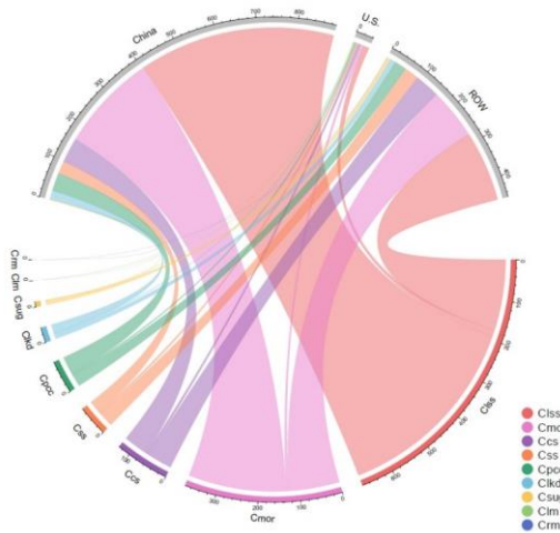
305 Figure 4: Cumulative uptake of CO 2 uptake by lime-containing materials in different regions. ROW: Rest of World, Ccs: CO 2 uptake by carbide slag, Clkd: CO 2 uptake by lime kiln dust, Ciss: CO 2 uptake by lime-stabilised soil, Cmor: CO 2 uptake by lime mortar, Cpec: CO 2 uptake by Precipitated calcium carbonate, Crm: CO 2 uptake by red mud, Css: CO 2 uptake by steel slag, Cslag: CO 2 uptake by carbonation sugar, Clm: CO 2 uptake by lime mud.
