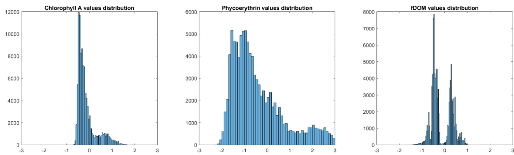
Figure 2: Histogram of values distribution of chlorophyll A, phycoerythrin and fDOM
