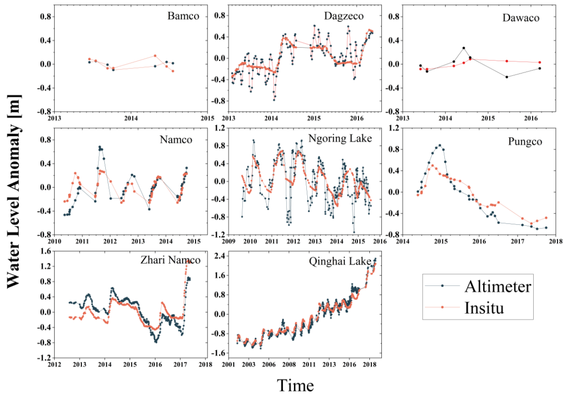
Fig. 6 Comparison of the water level anomaly between in situ data and lake level extracted from altimetry data
