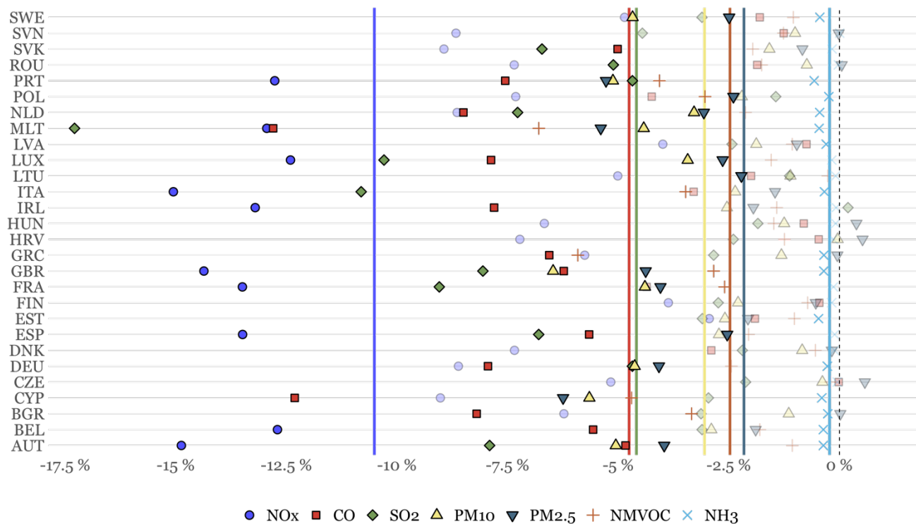
Figure 6 Relative decline in emissions of criteria pollutants [%] per species and country in 2020. The vertical lines indicate the average relative declines at the EU27 + UK level. Non-shaded marks highlight those countries/species for which reductions are larger than the ones computed at the EU27 + UK level.
