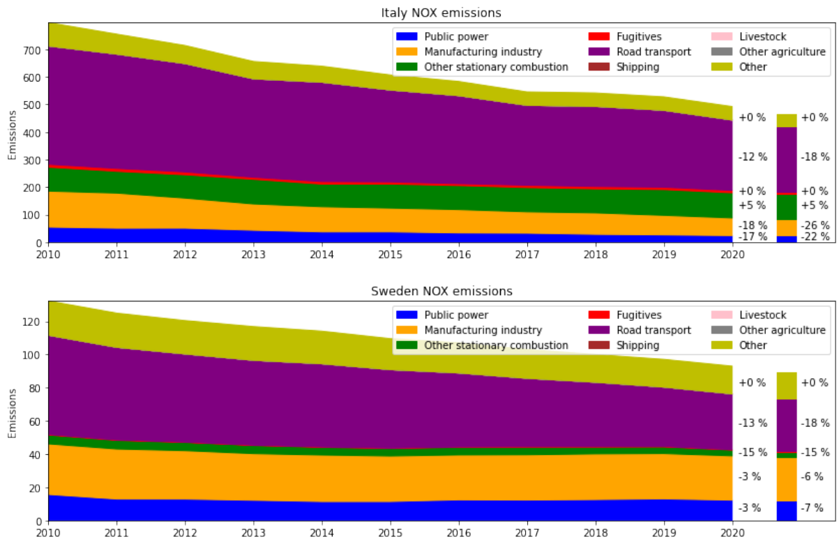
475 Figure 1: Time series of NO x emissions [kg/year] for Italy and Sweden. Up to 2018 official reported emissions are used. For 2019 and BAU 2020 emissions are estimated. For 2020 a second estimate is made (separate bar on the right) that includes AD affected by COVID-19. Percentages refer to the difference compared to 2018.
