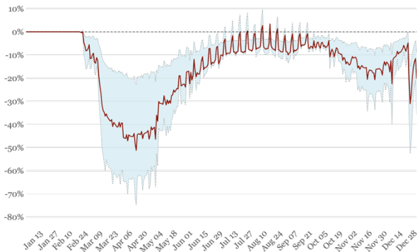
535 Figure 12 Map of the absolute cumulative NO x emission decline [kg·cell -1 ] in 2020 as compared to the business-as-usual scenario. Gridded emission changes are reported at a resolution of 0.1 x 0.05 degrees. Administrative boundaries are derived from the Micro World Data Bank (MWDB2, 2011). (Top), Average (dark red) and 5 th and 95 th percentiles (light blue shading) of the relative changes [%] in gridded NO x emissions in Italy (bottom-left) and Germany (bottom-right) for the period 1 January to 31 December 2020.
