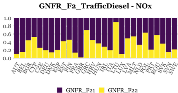
490 Figure 3 Average contribution of each GNFR subcategory (see definitions in Table 2) to total annual emissions for selected pollutants per country (EU27 + UK) for year 2020.
