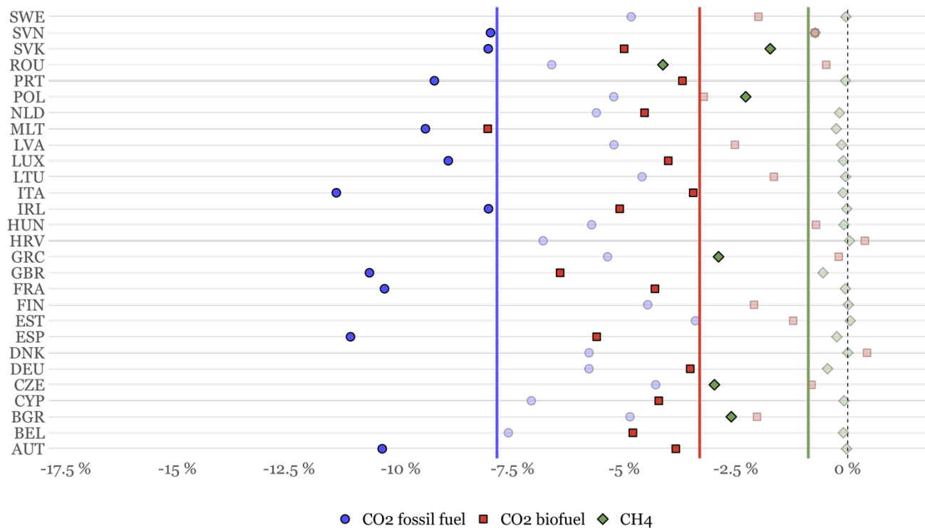
Figure 7 Same as Figure 6 for greenhouse gases
