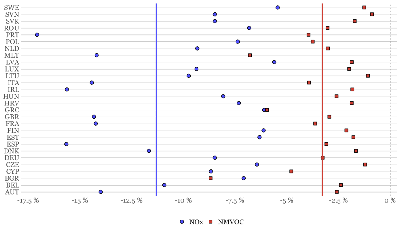
540 Figure 13 Relative NO x and NMVOC emission declines [%] per country occurring in high-density urban areas between January 1 st and December 31 st 2020. High-density urban areas were defined according to the Global Human Settlement Layer (GHSL) project (Pesaresi et al., 2019). The blue and red solid lines represent the average NO x and NMVOC emission declines at the EU27 + UK level, respectively.
