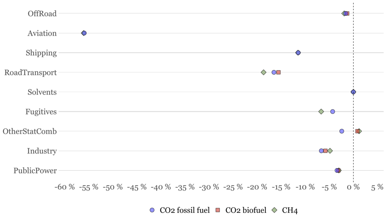
520 Figure 9 Same as Figure 8 for greenhouse gases. Note that for Aviation, shipping, use of solvents and fugitives no emissions are reported for CO 2 biofuel.
