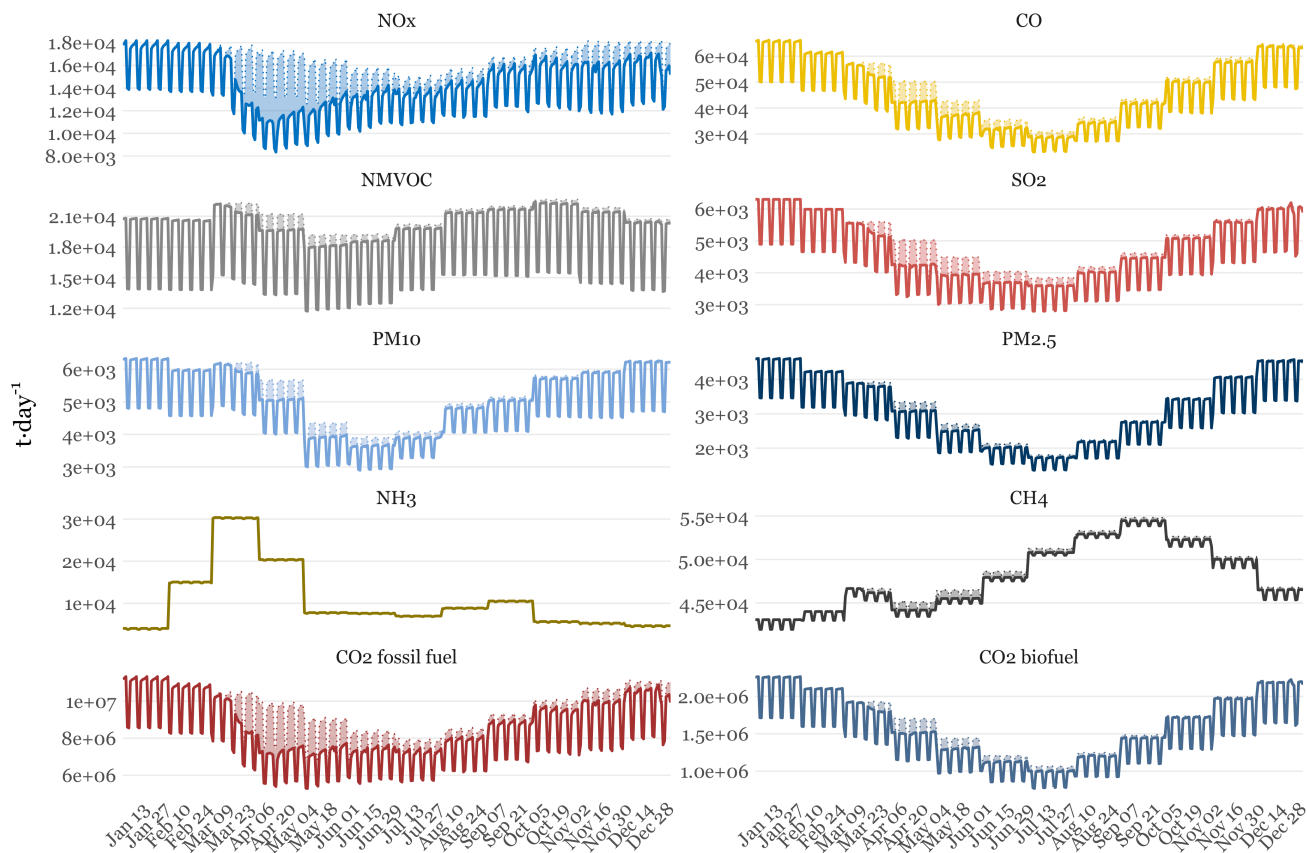
500 Figure 5 Daily emissions [ t \cdot day^{-1} ] by pollutant computed for the 2020 business-as-usual (BAU) (dotted lines) and COVID-19 (solid lines) scenarios between January 1 st and December 31 st 2020 for EU27 + UK. The areas highlighted between the two lines represent the emission differences between scenarios.
