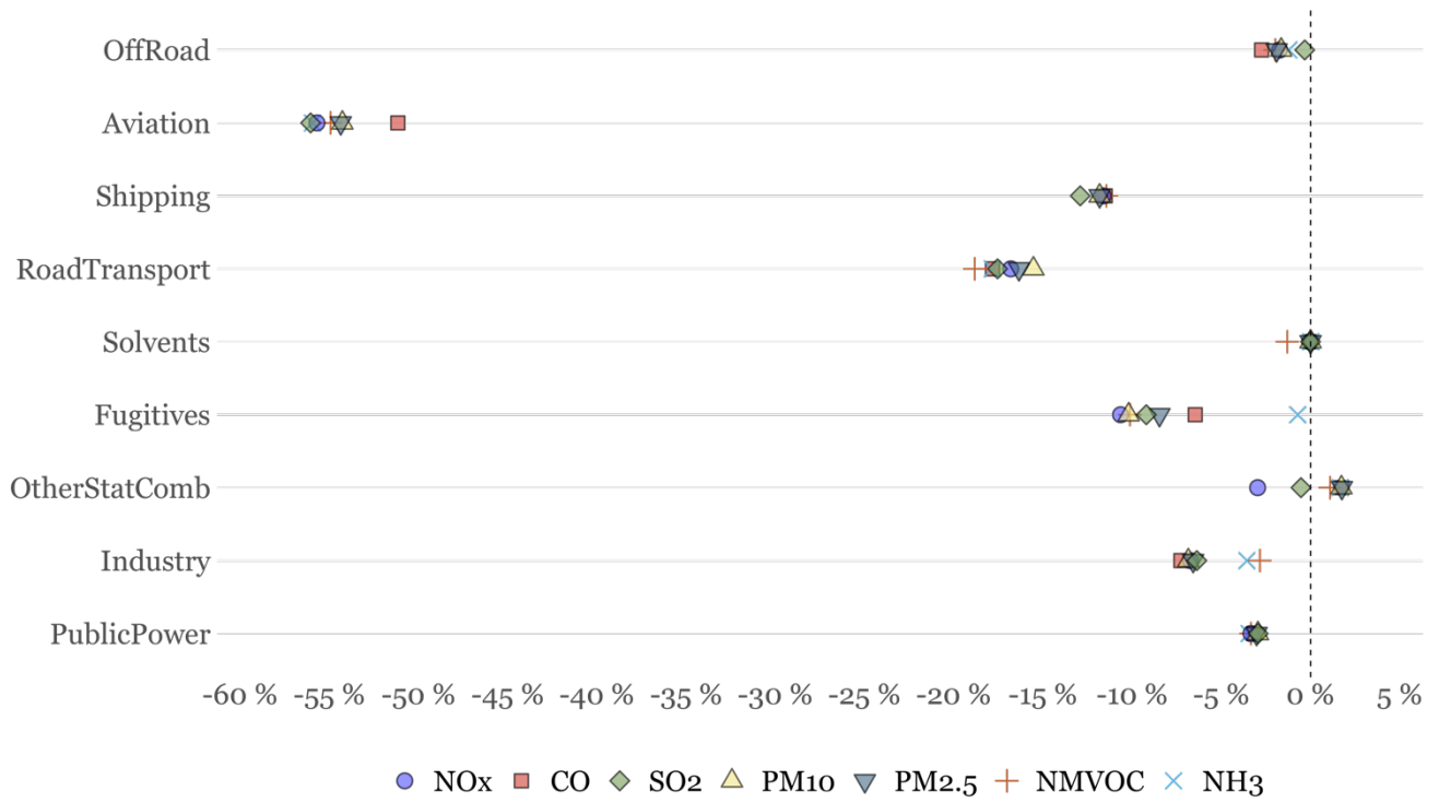
515 Figure 8 Relative decline in emissions of criteria pollutants [%] by sector and species between January 1 st and December 31 st 2020 for EU27 + UK. For the shipping sector the relative differences consider both inland and sea shipping sectors.
