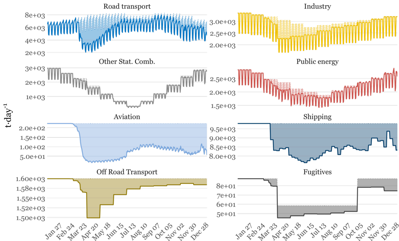
525 Figure 10 Daily NOx emissions [t·day -1 ] by sector computed for the 2020 business-as-usual (dotted line) and COVID-19 (solid line) scenarios between January 1st and December 31st 2020 for EU27 + UK. For the shipping sector the relative differences consider both inland and sea shipping sectors. The areas highlighted between the two lines represent the emission differences between the two scenarios.
