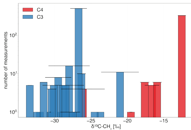
Figure A3. Measured \delta^{13}\text{C}_{\text{CH}_4} signatures from biomass burning in literature studies 3 according to the type of vegetation: a majority of C3 plants (blue) or C4 plants (red). Bar heights represent the number of measurements and black lines standard deviations.
