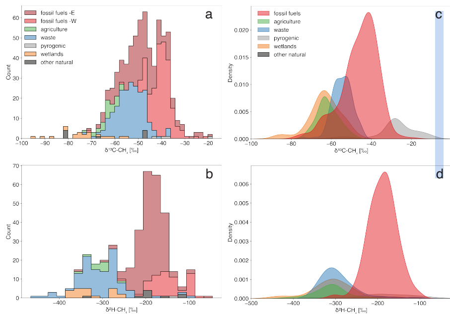
Figure 5. Distribution of \delta^{13}\text{C} (a, c) and \delta^2\text{H} (b, d) of \text{CH}_4 for different source categories. (a, b) Single measurements reported in the EMID (absolute numbers). "fossil fuels -E" shows fossil fuels data from Poland and Romania, and "fossil fuels -W" from the UK, the Netherlands, Germany, and France. (c, d) measured locations in all datasets (Sherwood et al., 2021), with EMID locations and additional literature (normalized probability density). "agriculture" represents ruminants and rice paddies emissions.
