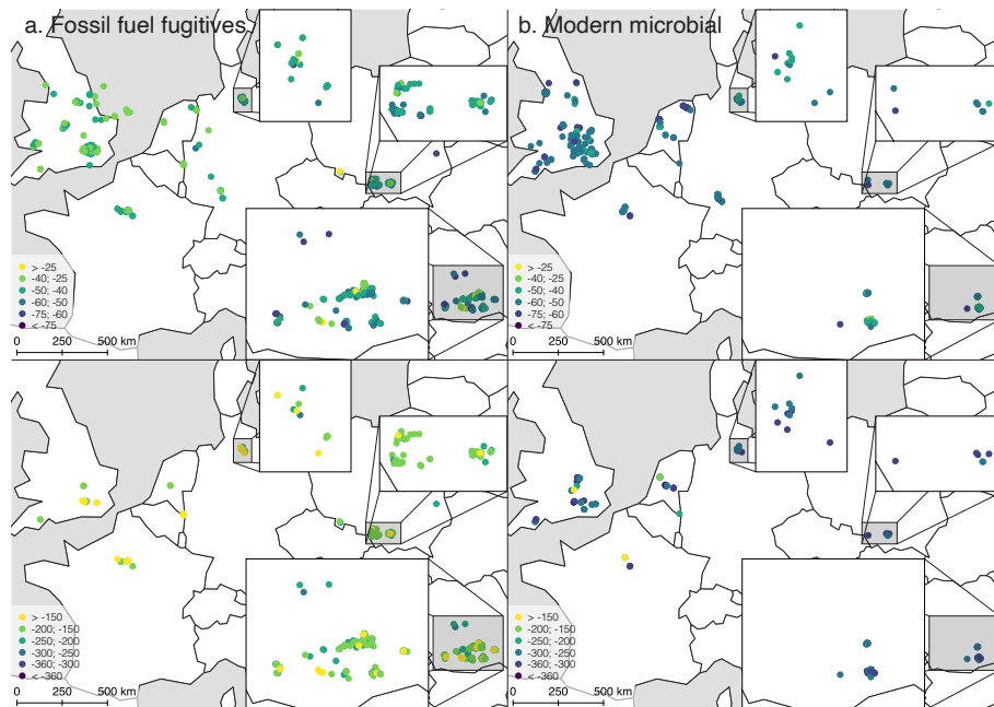
Figure 3. Measurement results of \delta^{13}\text{C} (top) and \delta^2\text{H} (bottom) of \text{CH}_4 from the EMID. A. \text{CH}_4 fugitive emissions from the exploitation of fossil fuels (gas leaks, oil and gas extraction and processing sites). B. \text{CH}_4 emissions from modern microbial fermentation sources (ruminants, landfills, sewage treatment plants and biogas plants).
