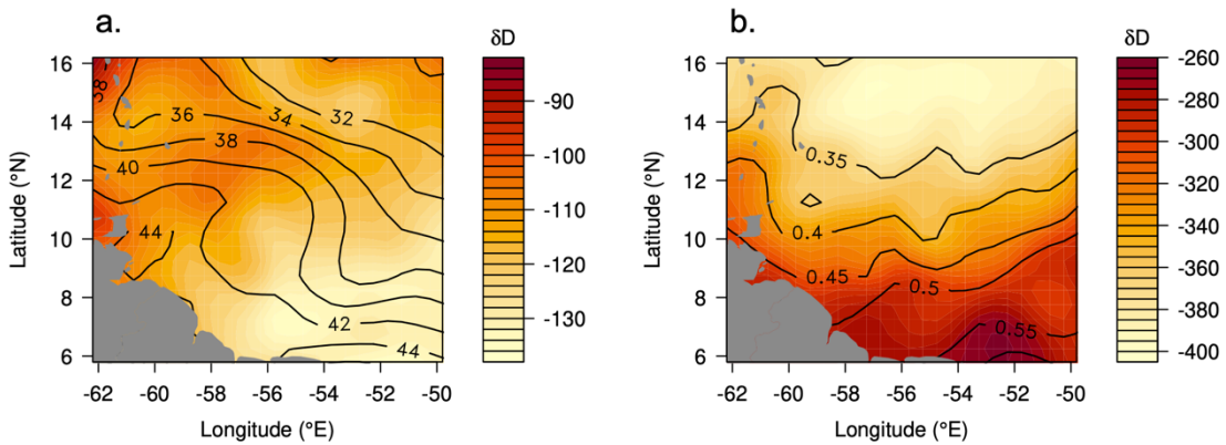
1585 Figure 14: a) TROPOMI total column \delta D (permil, shading) and total column water ( \text{kg m}^2 , contours), averaged on a 0.5-degree grid and smoothed for the period 11 Jan - 20 Feb 2020 (DOY 11-51). Only retrievals with a quality value of 0.5 or higher are selected. b) IASI \delta D (permil, shading) and specific humidity ( \text{g kg}^{-1} ; contours) at 6.4 km, averaged on a 0.5-degree grid and smoothed for the same period. (Note that the two water vapor fields represent distinct quantities.) Only data marked "good quality" in terms of spectral fit are used. 1590
