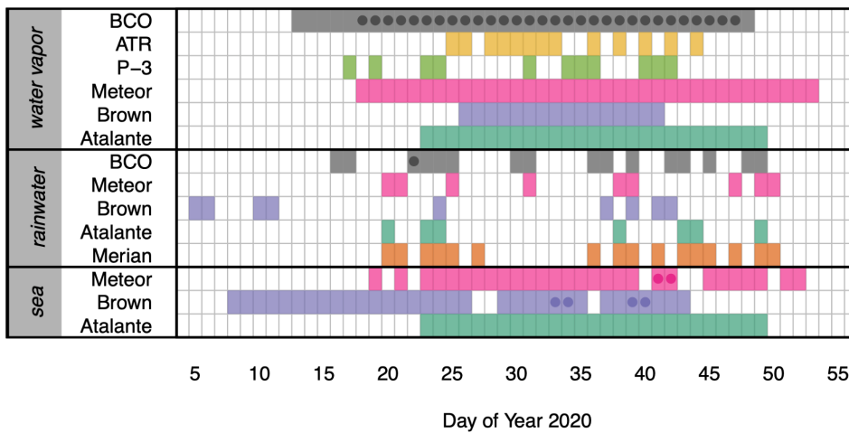
1505 Figure 3: Timeline of continuous (water vapor) and discrete (rain and seawater) isotopic sampling during EUREC 4 A. Dots either represent days when two laser analyzers were operating at the BCO or indicate intensive observation periods for rain or seawater (see main text for additional details). Discrete samples are represented by their collection times, which, in the case of Brown rainwater, were delayed in some cases by up to several days following precipitation.
