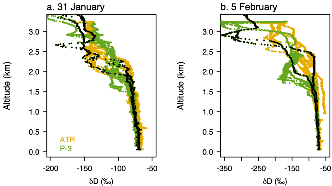
1580 Figure 13: Vertical \delta D profiles from the ATR (yellow) and the P-3 (green) for (a) 31 January (DOY 31) and (b) 5 February (DOY 36), the two days on which both aircraft were in the air simultaneously. P-3 observations with black centers represent takeoffs and landings, which were flown in closest proximity to the ATR and show the greatest structural similarity to ATR \delta D profiles.
