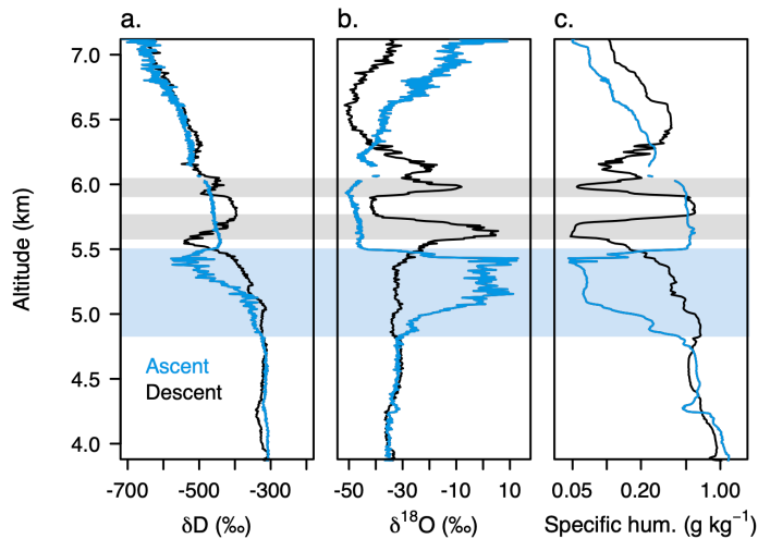
1540 Figure 9: Strong hysteresis causes (a) the \delta D vertical profile to differ substantially from vertical profiles of (b) \delta^{18}O and (c) specific humidity during aircraft ascents (blue) and descents (black) on P-3 Research Flight 8. Three dry layers, in which the delayed response and weaker signal in \delta D are most evident, are indicated by shading. \delta^{18}O is characterized by a better time response than \delta D but shows unphysical enrichment at altitude due to a shifting humidity-dependent bias over the course of the campaign. 1545
