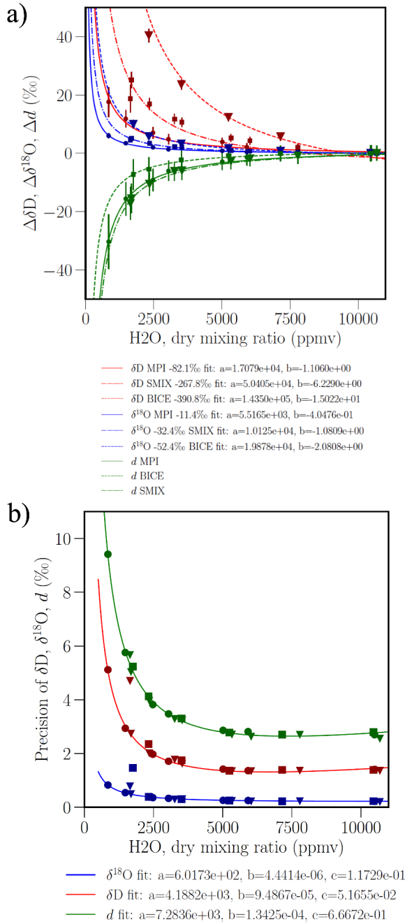
1530 Figure 7: Bias corrections and uncertainties associated with the ATR water vapor isotopic measurements: a) symbols illustrate the humidity dependence of the isotopic measurements for three distinct liquid standards (MPI, SMIX, BICE) while lines show the correction functions used to remove the detected biases in \delta^{18}O (blue) and \delta D (red); b) precision of the isotopic measurements as a function of the measured water vapor concentration.
