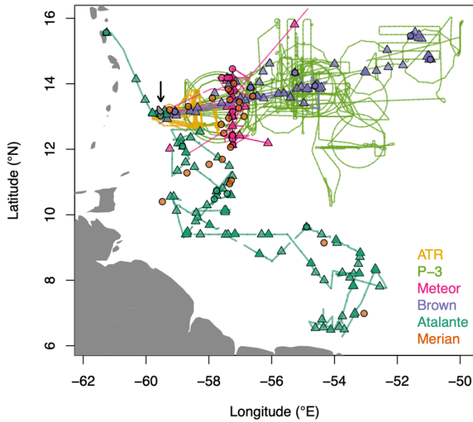
1495 Figure 2: Map of continuous (water vapor) and discrete (rain and seawater) isotopic sampling during the EUREC 4 A 2020 field experiment. Tracks for the various aircraft and ships are plotted only for periods during which water vapor isotopic sampling occurred. Circles and triangles indicate locations of rain and seawater sampling, respectively. The arrow points to Barbados, whose landmass is outlined in black. Readers are referred to Stevens et al. (2016) for a detailed map of Barbados and a photograph of Deebles Point and the Barbados Cloud Observatory (BCO).
