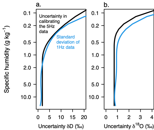
1535 Figure 8: P-3 isotopic uncertainties (x-axis) plotted as a function of specific humidity (y-axis). The y-axis is plotted on a logarithmic scale to convey the tendency toward higher uncertainty with aircraft altitude. Black lines represent the uncertainties associated with calibrating the 5 Hz data. Blue lines represent the standard deviations associated with the 1 s averages from the first two research flights: they reflect both the variability of the environment and the imprecision of the isotopic analyzer in flight.
