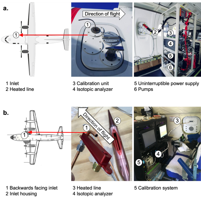
Figure 5: Water vapor isotopic sampling installations on the a) ATR and b) P-3 aircraft. (ATR schematic downloaded from https://t3projects.mpimet.mpg.de/coordination/platform-schematics . P3 schematic provided by NOAA.)
