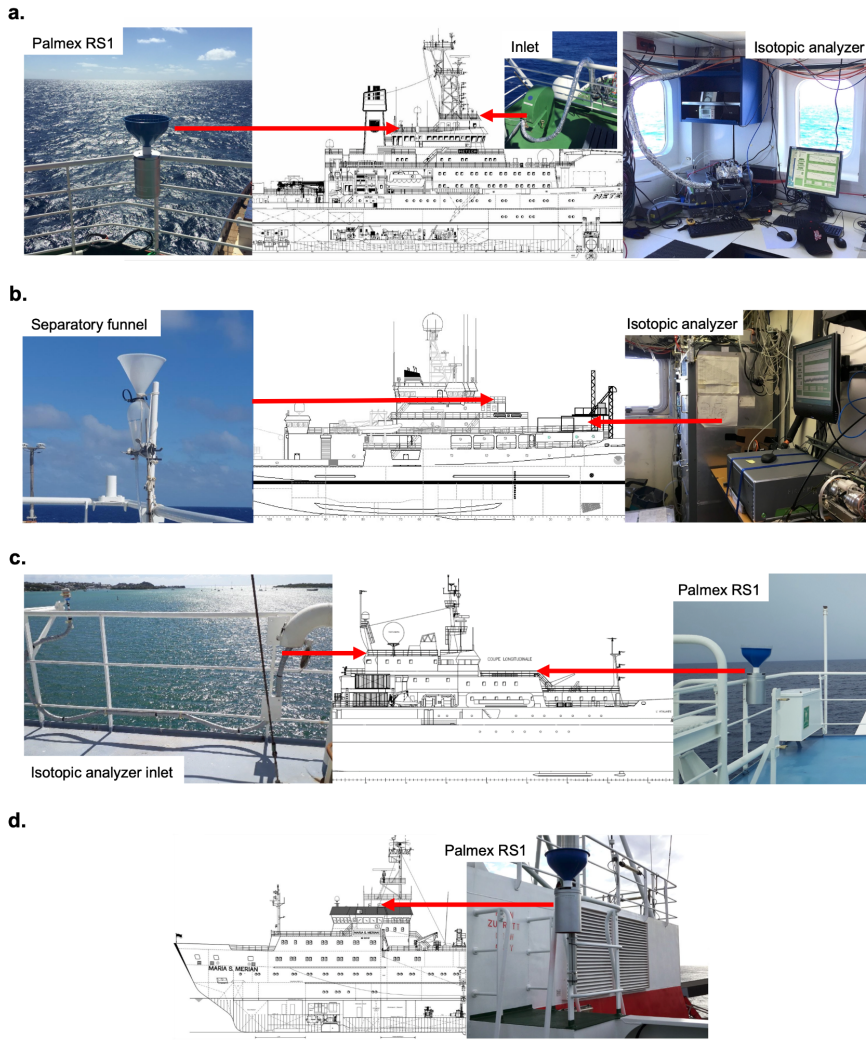
1705 Figure 6: Water isotopic sampling installations aboard a) the Meteor, b) the Brown, c) the Atalante, and d) the Merian. (Meteor and Merian ship schematics provided by University of Hamburg. Brown ship schematic provided by NOAA. Atalante ship schematic copyright ©Ifremer. Atalante photos courtesy of Jérôme Demange.)
