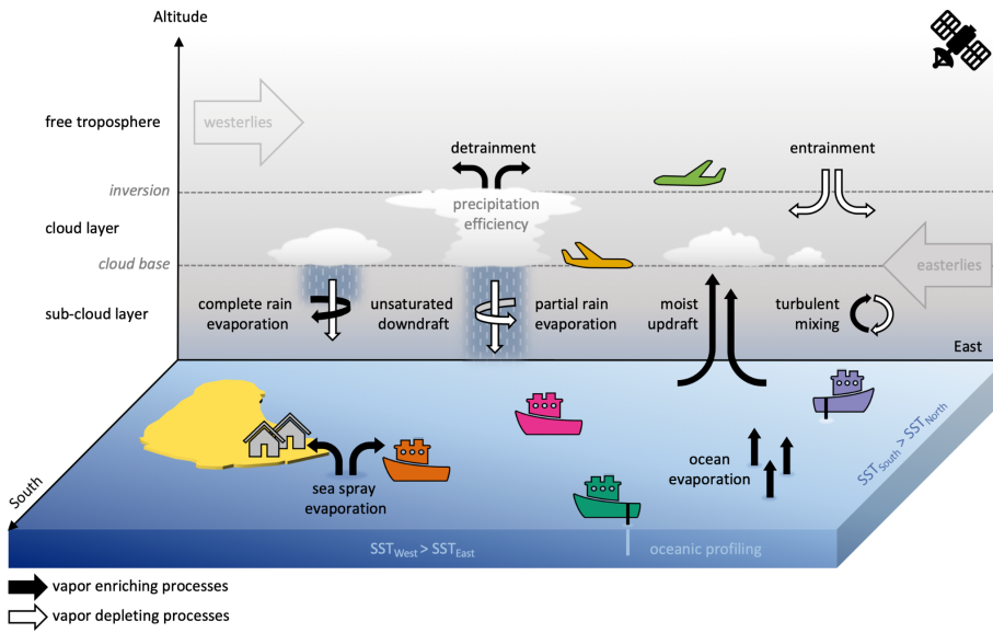
1670 Figure 1: Examples of moist processes that influence the water vapor isotopic composition of the trade wind environment around Barbados (yellow landmass) and that can be studied using the EUREC 4 A-iso dataset collection. Black arrows indicate processes expected to increase water vapor isotope ratios, while white arrows indicate processes expected to lower them. The ships and aircraft in the schematic represent the six mobile EUREC 4 A-iso in-situ sampling platforms.
