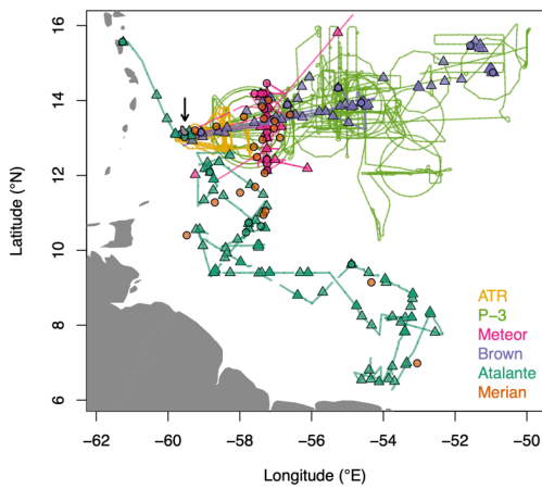
1675 Figure 2: Map of continuous (water vapor) and discrete (rain and seawater) isotopic sampling during the EUREC 4 A 2020 field experiment. Tracks for the various aircraft and ships are plotted only for periods during which water vapor isotopic sampling occurred. Circles and triangles indicate locations of rain and seawater sampling, respectively. The arrow points to Barbados, whose landmass is outlined in black. Readers are referred to Stevens et al. (2016) for a detailed map of Barbados and a photograph of Deebles Point and the Barbados Cloud Observatory (BCO). 1680
