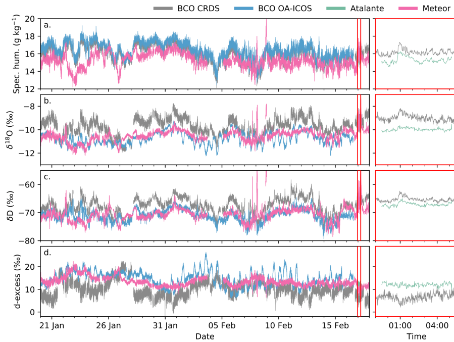
1755 Figure 12: Time series of (a) water vapor concentration, (b) \delta^{18}\text{O} , (c) \delta\text{D} , and (d) d from the BCO CRDS analyzer (gray), 1760 the BCO OA-ICOS analyzer (blue), and the Meteor (magenta) for the period 20 January to 17 February 2020 (DOY 20-48). The Meteor trace is shifted by 9 hours. Rightmost panels show an enlarged view of the BCO CRDS system and the Atalante (teal) for the period 23:30 16 Feb - 05:10 17 Feb UTC (DOY 47-48), when the Atalante was 2-6 km northeast of the BCO. The Atalante trace is shifted by 10 minutes. (Note that the time series shown here are not smoothed as they are for the comparisons described in Table 2.)
