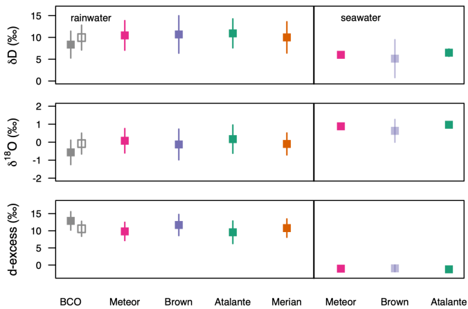
1745 Figure 11: Campaign-mean rainwater and near-surface seawater values from the BCO and ship-based platforms. Whiskers represent standard deviations. The rainwater comparison excludes Brown samples flagged for delayed collection times, the first Atalante sample, and BCO and Merian samples flagged because no precipitation was detected by the platform's primary meteorological station. Filled symbols for the BCO include rainwater collected every 10
