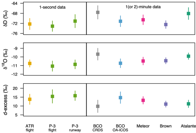
1735 Figure 10: Campaign-mean near-surface water vapor isotopic values from the various ground, airborne, and ship-based 1740 platforms. Whiskers represent standard deviations. Values from in flight represent a height of 150±15 m.a.s.l. With the exception of the BCO OA-ICOS measurements, only data that are not flagged for suspect quality are included in the comparison.
