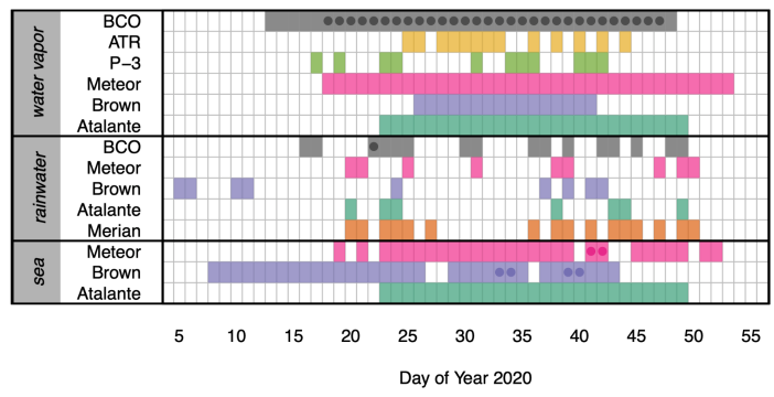
1685 Figure 3: Timeline of continuous (water vapor) and discrete (rain and seawater) isotopic sampling during EUREC 4 A. Dots either represent days when two laser analyzers were operating at the BCO or indicate intensive observation periods for rain or seawater (see main text for additional details). Discrete samples are represented by their collection times, which, in the case of Brown rainwater, were delayed in some cases by up to several days following precipitation.
