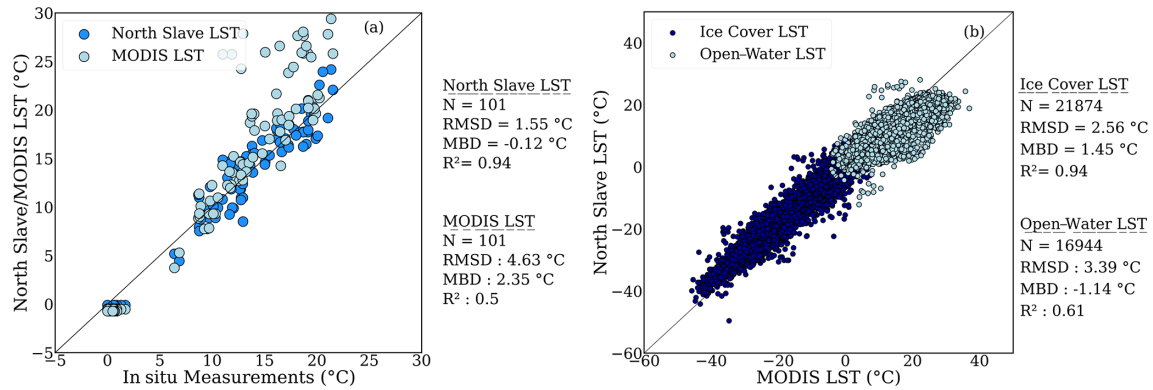
Figure 6. Comparison of North Slave LST and MODIS LST to (a) DataStream and ECCC in situ water surface temperature measurements during open-water seasons (b) MODIS LST during open-water and ice-covered seasons.
