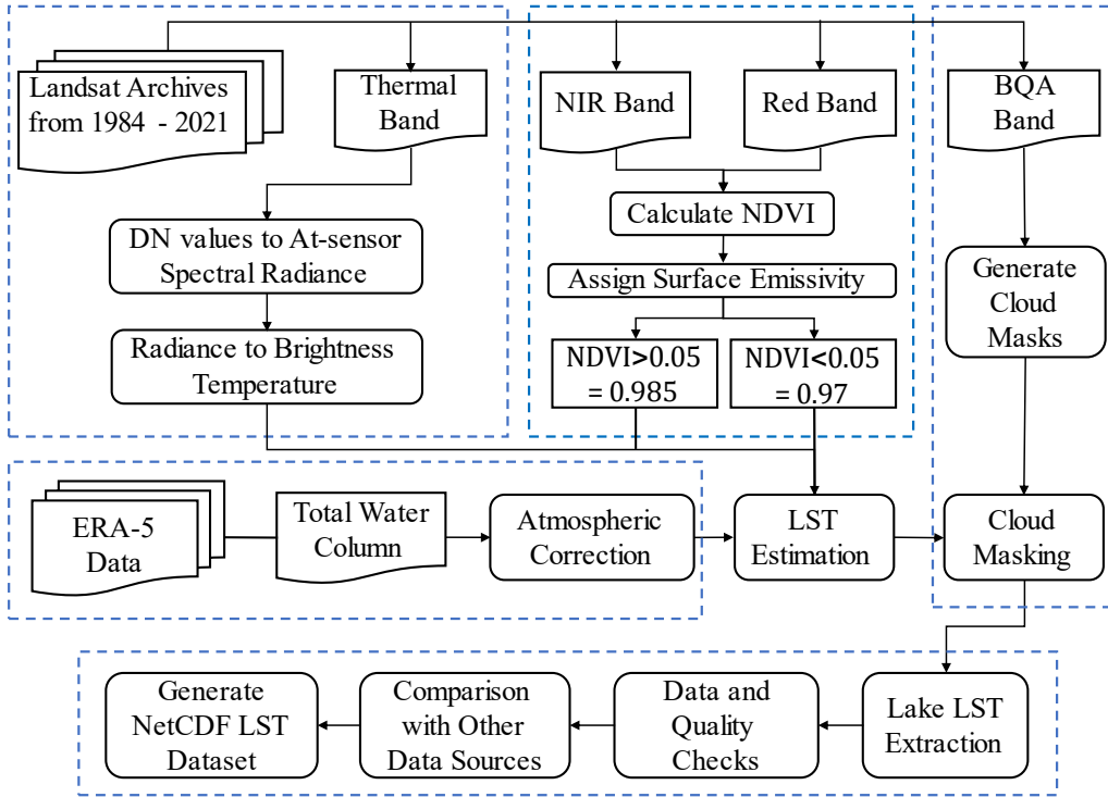
215 Figure 2: Workflow and methods for generating LST dataset from Landsat archives.
