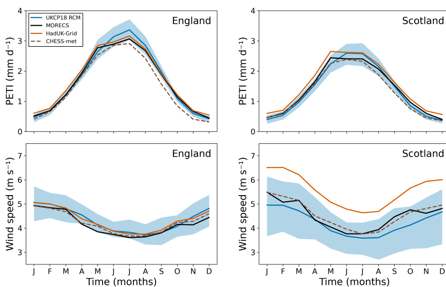
Figure 12. Monthly mean PETI (top row) and wind speed (bottom row) averaged over England (left) and Scotland (right) (1981–2017) from MORECS (black line), UKCP18 RCM (blue line shows the ensemble mean and light blue area shows the ensemble range), HadUK-Grid (orange line), and CHES (brown dashed line).
