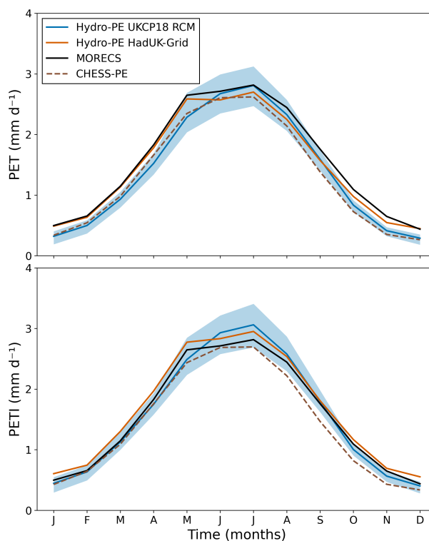
Figure 11. Monthly mean PET (top) and PETI (bottom) averaged over GB for 1981-2017. The black line in both panels is MORECS PE (which includes the interception correction, so is PETI). The blue line shows the ensemble mean of Hydro-PE UKCP18 RCM, and the light blue area shows the ensemble range. The orange line shows Hydro-PE HadUK-Grid. The brown dashed line shows CHES-PE.
