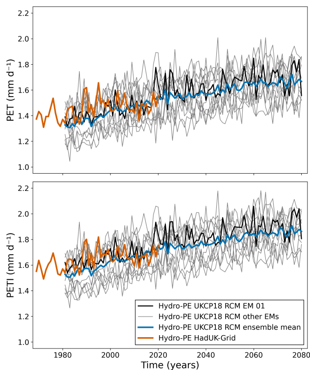
Figure 6. Time-series of annual mean PET (top) and PETI (bottom). The black line shows ensemble member 01 of Hydro-PE UKCP18 RCM, the grey lines show the other ensemble members, and the blue line shows the ensemble mean. The orange line shows Hydro-PE HadUK-Grid. Note that the regions averaged are slightly different — Hydro-PE UKCP18 RCM averages over the UK, the Republic of Ireland and a small amount of northern France, while Hydro-PE HadUK-Grid only includes the UK.
