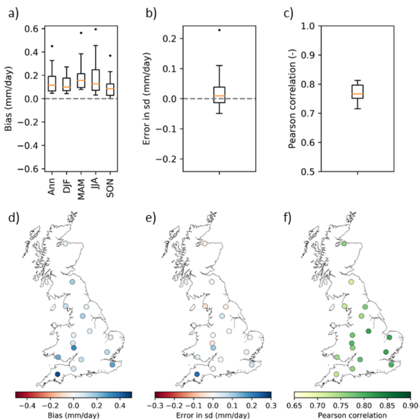
Figure 13. Evaluation of the Hydro-PE HadUK-Grid PETI against daily MORECS PE (which is also PETI) across 16 MORECS sites. Boxplots summarise results over all 16 sites including: a) bias in mean PETI values calculated annually (Ann), over winter (DJF), spring (MAM), summer (JJA) and autumn (SON), b) difference in the standard deviation, c) Pearson correlation coefficient. Maps show annual bias, difference in the standard deviation and Pearson correlation coefficient values at each of the MORECS sites.
