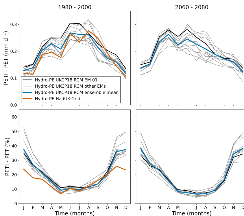
Figure 9. Mean monthly climatology of the difference between PETI and PET as an absolute value (top row) and as a percentage of PET (bottom row). The left hand column shows the mean over 1980–2000, the right hand column shows the mean over 2060–2080. Line styles as in Fig. 6
