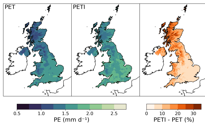
Figure 3. Annual mean PET (left) and PETI (centre) from Hydro-PE HadUK-Grid (1969-2020). The right hand panel shows the relative difference between PETI and PET as a percentage of PET.
