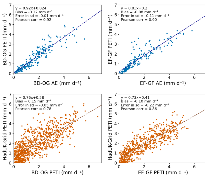
Figure 15. The top panels show PETI calculated from site meteorology plotted against observed AE, for values in winter (DJF), spring (MAM) and autumn (SON). The bottom panels show the HadUK-Grid PETI against the EC site PETI. The left-hand column is the BD-OG site, the right-hand column is the EF-GF site. Dashed lines show the least squares linear fit to the data.
