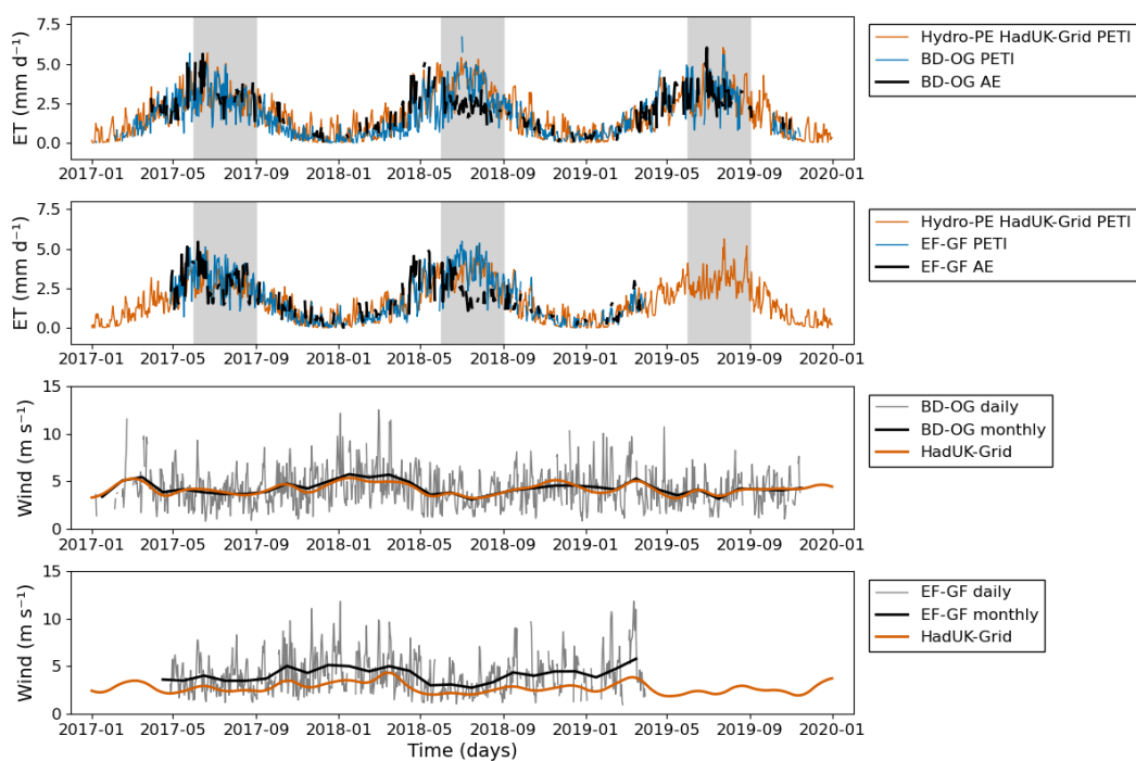
Figure 14. Upper two panels show time series of measured daily AE (black), calculated daily PETI (blue) and HadUK-Grid PETI (orange) for two EC sites (BD-OG and EF-GF). The grey regions show the summer data that are excluded from calculating the metrics. Lower two panels show observed daily wind speed (grey), observed monthly mean wind speed (black) and HadUK-Grid interpolated wind speed (orange) for two EC sites.
