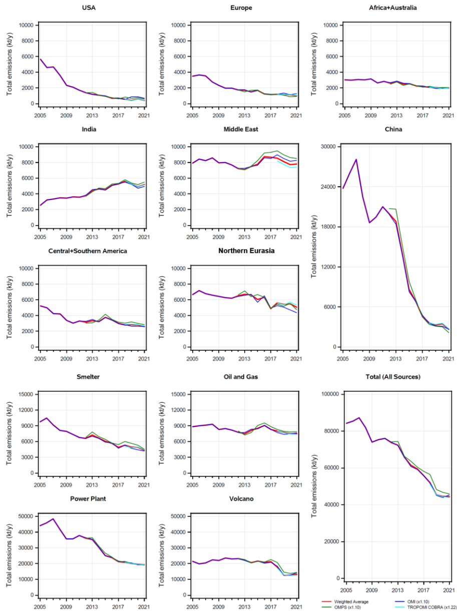
740 Figure 56. Annual SO 2 emissions from four satellite data sets: version 2 catalogue OMI VCD data (blue), version 2 catalogue OMPS data (green), version 2 catalogue TROPOMI COBRA data (cyan) and the weighted average (red). The data are grouped by region (8 top panels), by emission source type (bottom 4 panels) and the bottom right panel shows total emissions from all sources. TROPOMI-based estimates were increased by 22% and OMI and OMPS data were increased by 10% as discussed in the text. The weighted average is based on OMI data only in 2005-2011, on OMI and OMPS data in 2012-2017, and on data from all three instruments in 2018-2021.
