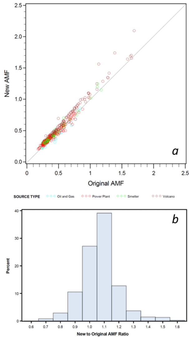
Figure 2. (a) Scatter plot of the AMFs used in the original catalogue vs. the AMFs used in the version 2 catalogue. Each dot corresponds to one emission source and the dot color reflects the source type as shown in the legend. There are total of 555 sources on the plot. The correlation coefficient between the two data sets is 0.98. (b) The distribution of the ratio of the new AMF values to the AMF values in the original catalogue.
