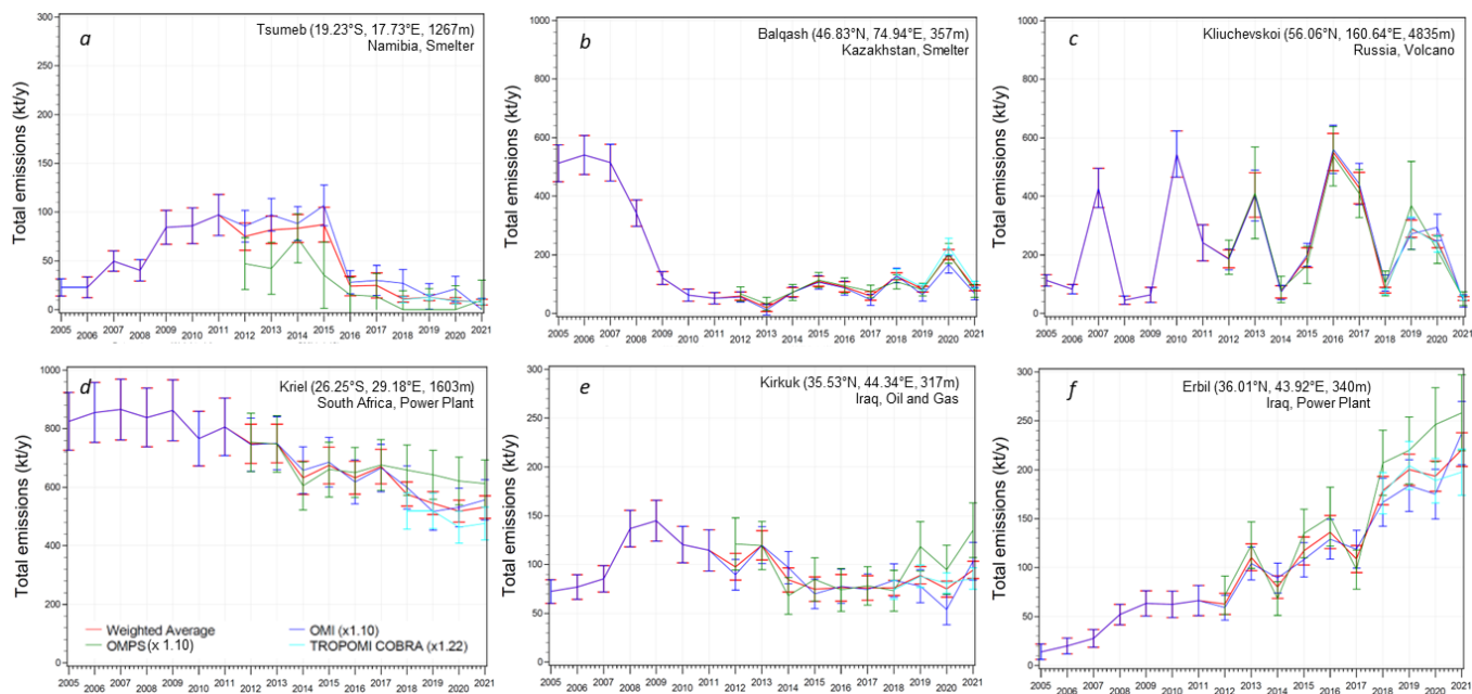
Figure 4 Annual emission estimates from the three satellite data sources: OMI (blue), OMPS (green) and TROPOMI (cyan), and their weighted average (red) with 2\sigma error bars. TROPOMI-based estimates were increased by 22% and OMI and OMPS data were increased by 10% as discussed in the text. The emission source names, types, coordinates, and elevations above sea level are shown.
