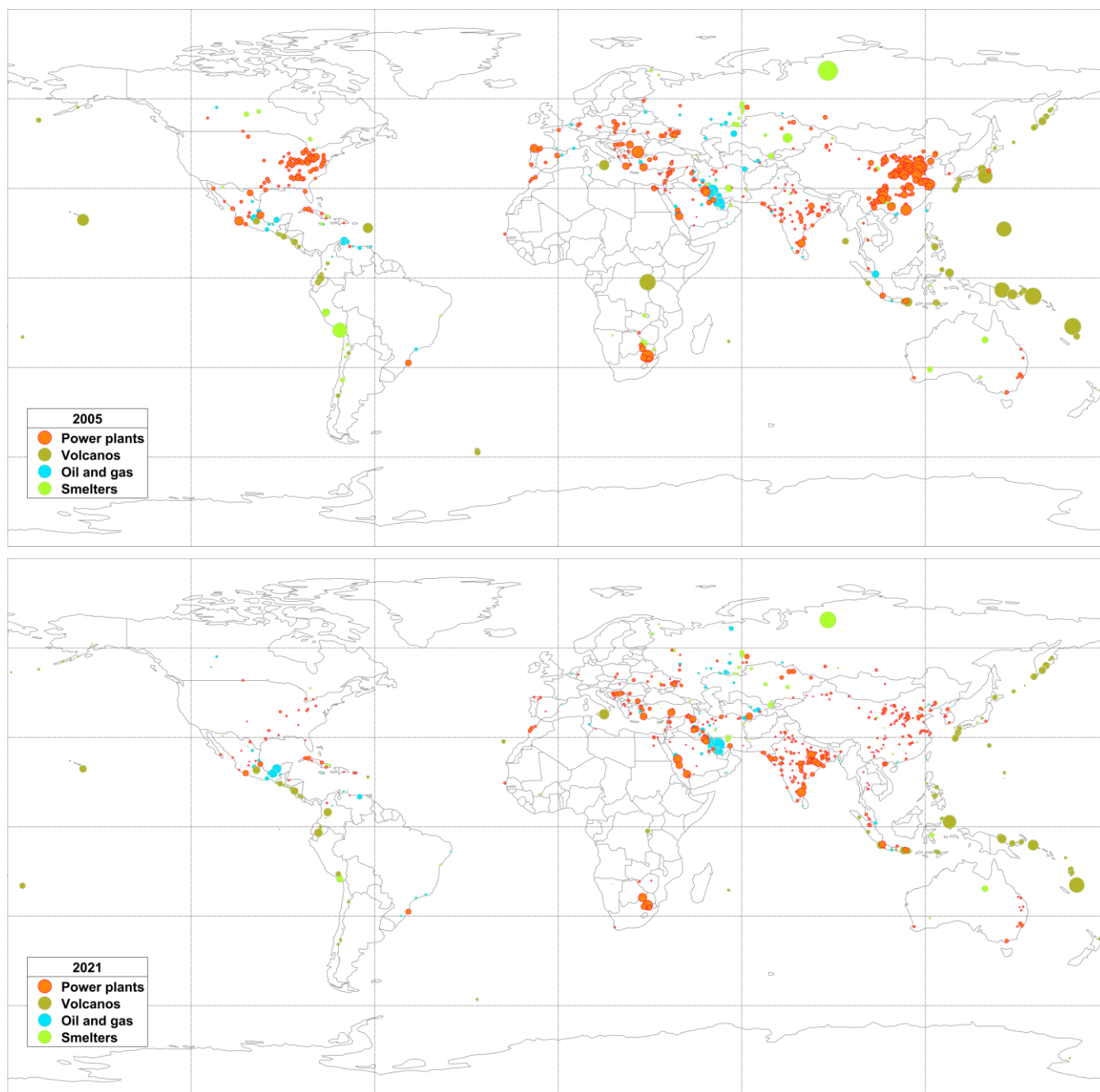
Figure 7. SO 2 emissions sources listed in the version 2 catalogue for 2005 (top) and 2021 (bottom). Only sources where the ratio of the emission value to its standard deviation is greater than 3 are shown. The size of the symbols is proportional to the annual emission values.
