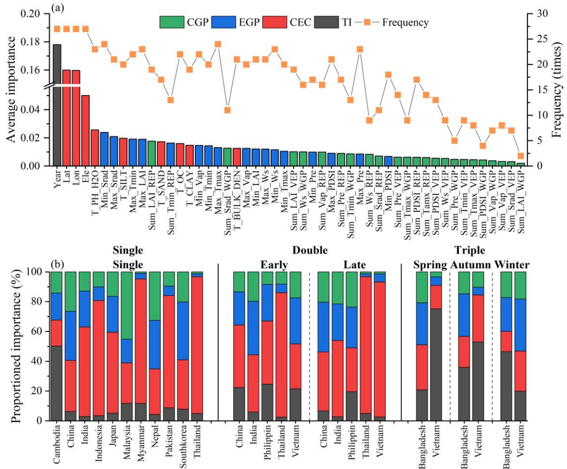
405 Figure 9: (a) Average frequency and importance of each predictor. (b) The proportioned importance of each predictor category for seasonal rice.
