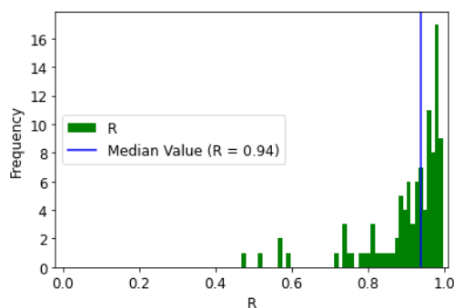
Figure 7 The distribution of R of relative water storage benchmarking results against Tortini et al. (2022) for 104 lakes (vertical blue line: the median value).
