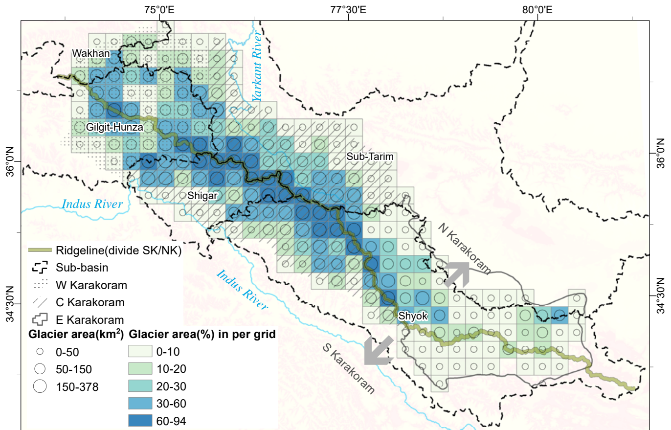
Fig. 6. Spatial distribution of Karakoram glaciers. For regional comparison, the Karakoram mountains were divided into western, central and eastern Karakoram (WK, CK and EK) according to the Indus and Tarim sub-basins, and into Northern and Southern Karakoram based on the main central ridgeline (green line). The major sub-basin divisions (Wakhan, Gilgit-Hunza, Shigar, Sub-Tarim and Shyok) in the Karakoram mountains also are shown. Hollow circles and coloured grids represent the glacier area and glacier proportion on the 20 \text{ km} \times 20 \text{ km} grid.
