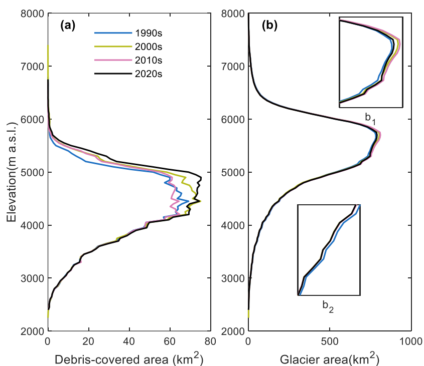
350 Fig. 7 Altitudinal profiles of the glacier surface area at 50 m intervals for debris-covered ice (a) and all glaciers (b), showing variations from 1990 to 2020. The subpanel b 1 and b 2 inserted in figure (b) correspond to zooms on the altitude interval 5000~6000 m a.s.l. and 3500~4000 m a.s.l..
