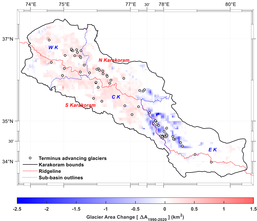
Fig.11 Glacier change in the Karakoram during 1990~2020. Glacier area aggregated on a 5 km × 5 km grid. White dots represent the glaciers advanced during the period 1990-2020. The Karakoram Mountains were divided into western, central and eastern Karakoram (WK, CK and EK) according to the Indus and Tarim sub-basins, and into Northern and Southern Karakoram based on the main central ridgeline.
