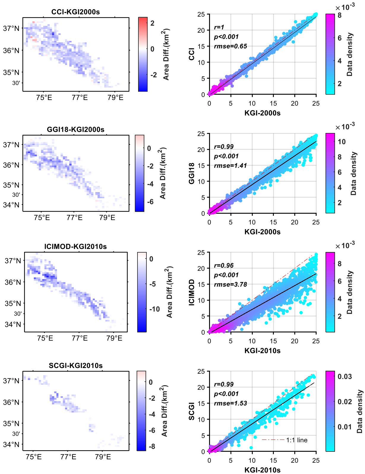
Fig.7.10. Comparison between the KGI inventory and previous glacier inventories. All data are aggregated on a 5km \times 5km grid. The map in the left column represents the area difference between previous glacier inventories and the KGI inventory from the same or closest period (SCGI and ICIMOD inventories are compared with KGI-2010s, while the updated GAMDAM (GGI18) and CCI inventories are compared with KGI-2000s). The right column illustrates, from top to bottom, the scattergrams of glacier area in each 5 km grid cell of the KGI inventory, plotted against the GGI18, CCI, ICIMOD and SCGI inventories in the Karakoram mountains.
