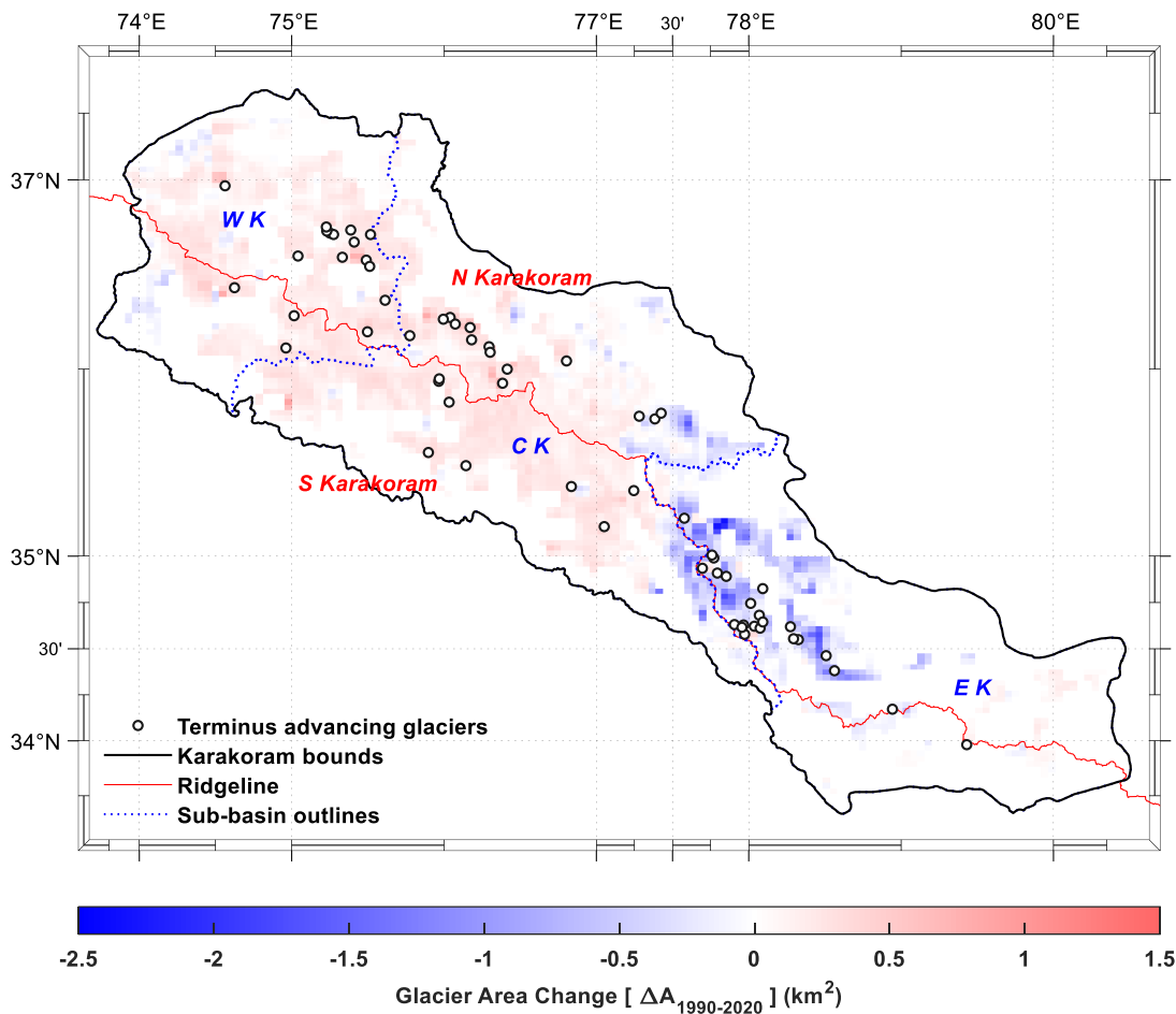
Fig.8-11 Glacier change in the Karakoram during 1990–2020. Glacier area aggregated on a 20\text{-}5 km \times 20\text{-}5 km grid. Hollow-White dots represent the glaciers advanced during the period 1990–2020. The Karakoram Mountains were divided into western, central and eastern Karakoram (WK, CK and EK) according to the Indus and Tarim sub-basins-, and into Northern and Southern Karakoram based on the main central ridgeline.
