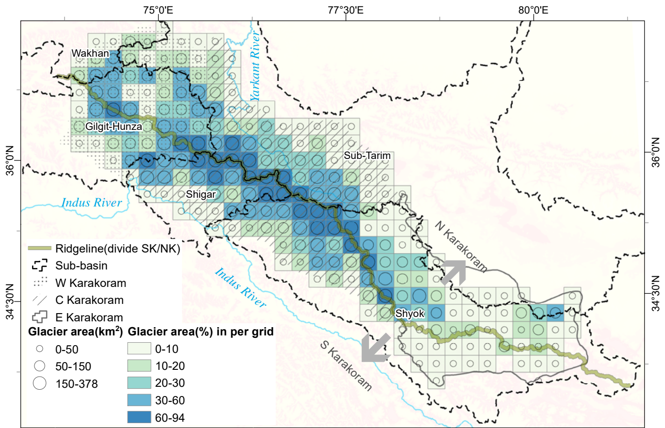
Fig. 56. Spatial distribution of Karakoram glaciers. For regional comparison, the Karakoram Mountains were divided into western, central and eastern Karakoram (WK, CK and EK) according to the Indus and Tarim sub-basins, and into Northern and Southern Karakoram based on the main central ridgeline (green line). The major sub-basin divisions (Wakhan, Gilgit-Hunza, Shigar, Sub-Tarim and Shyok) in the Karakoram mountains also are shown. Hollow circles and coloured grids represent the glacier areas, and glacier proportion on the aggregated on a 20 km × 20 km grid.
