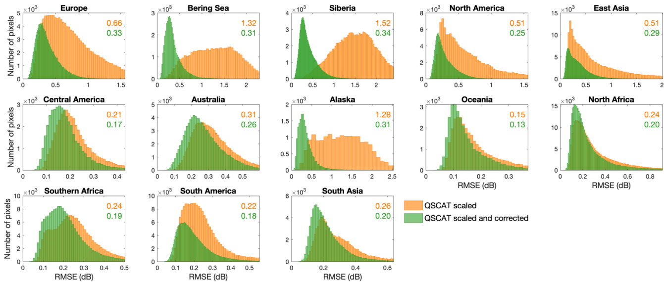
800 Figure 7. RMSE-based quality assessment of the LHScat CSea data set at the pixel level. Each panel shows the result of one region. Inside each panel, the RMSE values (unit dB) between the C-band and the scaled Ku-band signals in the overlapping years (1999-2001 and 2007-2009) were calculated for all pixels and colored in orange. As a comparison, the RMSE values between the C-band and the corrected Ku-band signals in the overlapping years were also calculated and colored in green. The medians of the RMSE values are labelled inside each panel. The rRMSE-based quality assessment is 805 available in supplementary material (Figs. S2 & S3).
