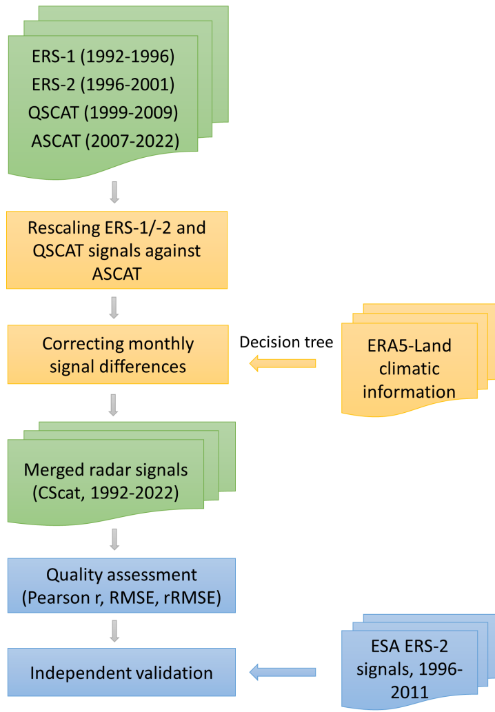
Figure 2. Flow chart illustrating the development and assessment of the CScat data set. Inputs/outputs are colored in green, the signal merging procedures colored in yellow, and assessment and validation for the merged signals colored in blue.
