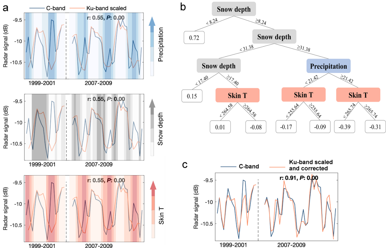
815 Figure 4. Illustration on the correction of the monthly signal differences between the C-band and the scaled Ku-band signals in the overlapping years (1999-2001 and 2007-2009), taking one pixel in the Tibetan Plateau (88.01E, 33.73N) as an example. (a) The C-band and the scaled Ku-band signals before correction in one pixel of Amazonia. The location of the pixel is indicated by a red dot in the left-most map. The three panels in (a) show the radar signals against monthly precipitation (unit mm), skin temperature (unit K), and snow depth (unit mm). The blue-white background shows the monthly precipitations. The vertical dotted line in each panel a and c separates the ERS-QSCAT overlapping (1999–2001) and QSCAT-ASCAT (2007–2009) overlapping periods. (b) Decision tree regression with monthly precipitation, skin temperature, and snow depths as predictors of the signal differences. Predicted signal differences by decision tree regression with precipitation as input versus observed signal differences. (c) The C-band and the final corrected Ku-band signals by the decision tree regression. The vertical dotted line in a and c separates the ERS-QSCAT overlapping (1999–2001) and QSCAT-ASCAT (2007–2009) overlapping periods. (d-f) show one example of the signal correction in Alaska with snow depth as the predictor of the signal differences. (g-i) show one example of the signal correction in Alaska with skin temperature as the predictor of the signal differences. 820 825
