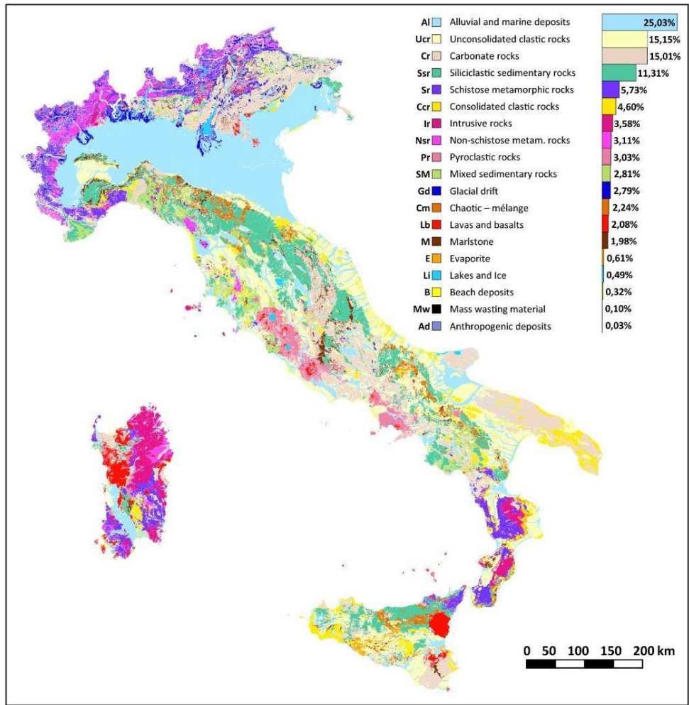
261 Figure 5: Map of Italy showing the 19 lithological classes identified both with the short ID and the extended name. 262 Percentage distribution of each lithological class over the Italian territory is indicated and visualized in a bar chart. 263
