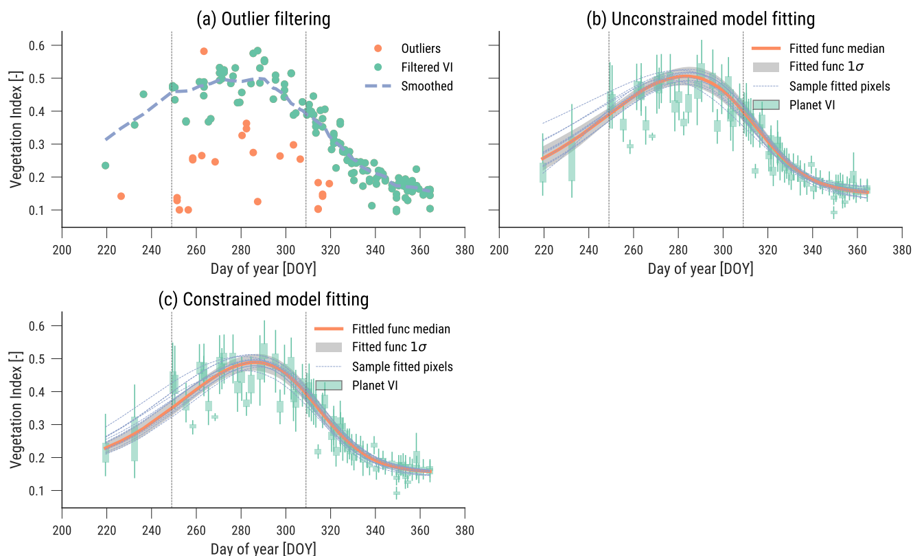
Figure 5. Planet VI time series processing steps example for field 7074ZIN. (a) Outlier filtering. (b) First pass single pixel double logistic fitting (unconstrained). (c) Second pass single pixel double logistic fitting (phenology parameters constrained by median field). The vertical lines show the extent of the ground campaign period.
