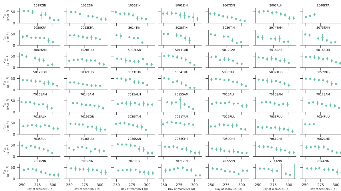
Figure 7. Per field temporal evolution of in situ leaf area chlorophyll concentration ( C_{ab} ). For any date, the mean is shown, and errorbars represent \pm 1\sigma .
