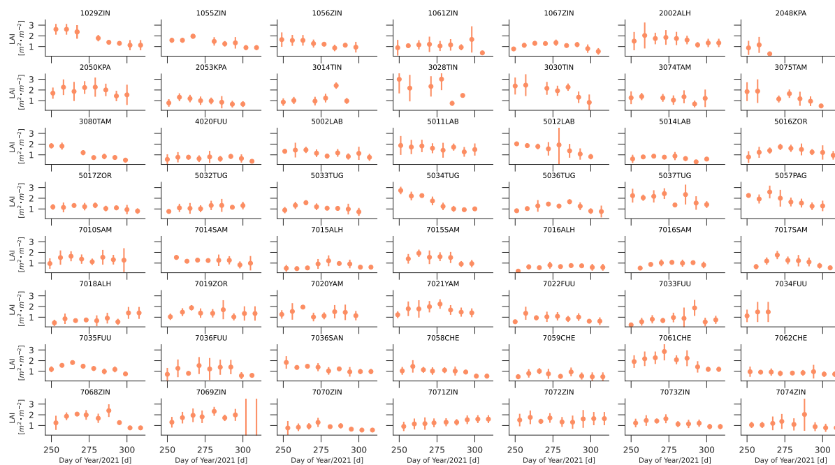
Figure 6. Per field temporal evolution of in situ leaf area index (LAI). For any date, the mean is shown, and error bars represent \pm 1\sigma .
