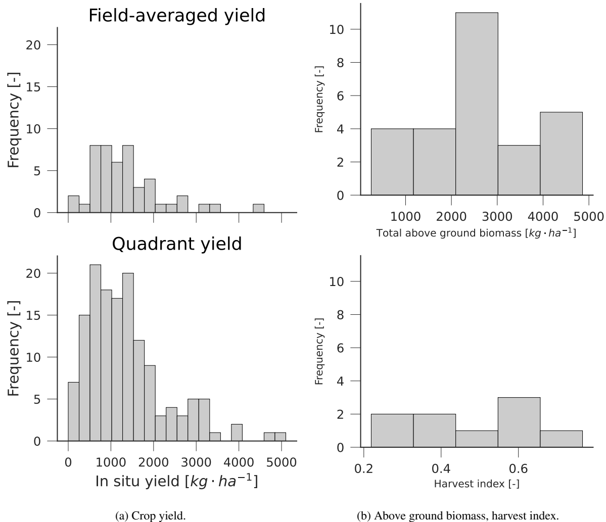
Figure 8. Crop yield distribution (top left: field averaged, bottom left: individual quadrants), field averaged above ground biomass (top right) and field averaged harvest index (bottom right).
