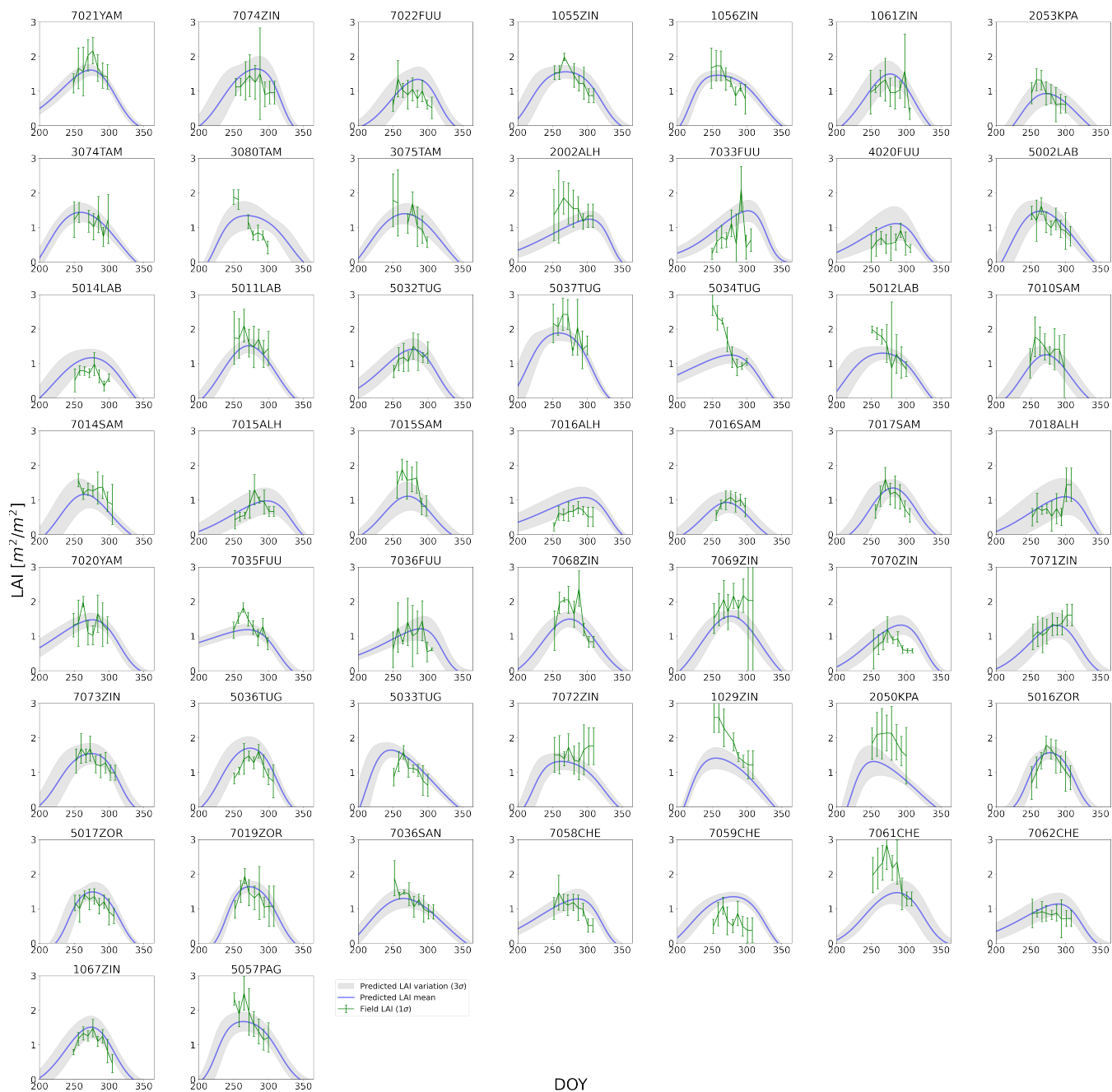
Figure 10. Predicted LAI time series and associated standard deviation (blue line and grey area) in comparison with field measurements (per field mean and standard deviation, green lines).
