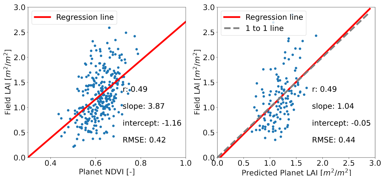
Figure 9. NDVI to LAI calibration (left) and validation (right)
