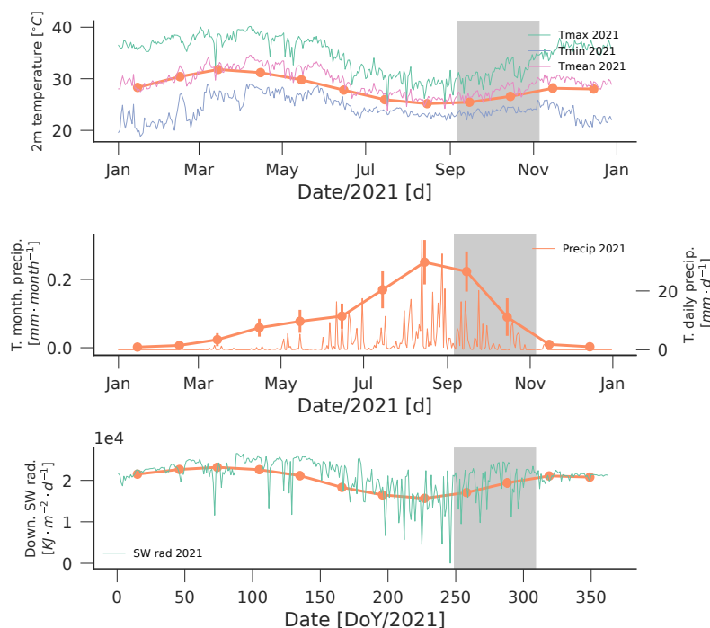
Figure 3. Monthly climatologies for temperature (top), precipitation and shortwave downwelling radiation over the Tamale area (derived from ERA5/Land dataset between 1990 and 2021), as well as daily temperatures, precipitation and downwelling radiation for 2021. Grey area indicates biophysical parameter collection period.
