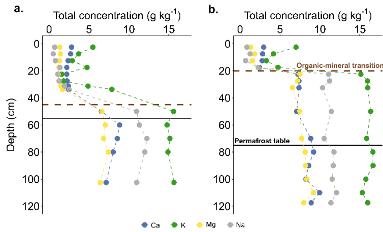
240 Figure 4: Distribution of total concentrations in Ca, K, Mg, and Na (g kg -1 ) in an “organic-thick” soil profile (Min1) and an “organic-thin” soil profile (Mod3). Permafrost table is indicated by the straight black line, and the transition between the organic (SOC ≥ 20%) and mineral (SOC < 20%) soil is indicated by the dotted brown line.
