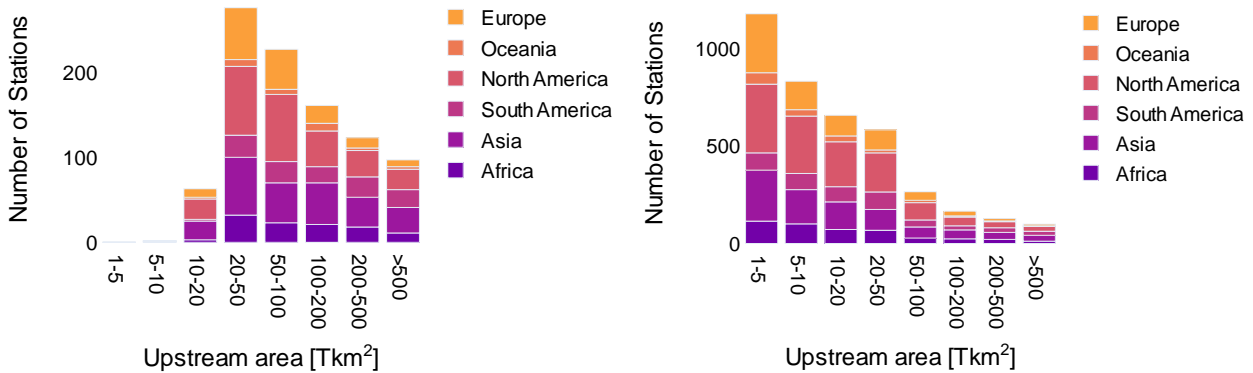
400 Figure 9: Histogram of selected calibration stations (a) 949 stations for 30' (b) 3,917 stations for 5', classified by upstream area and continent
