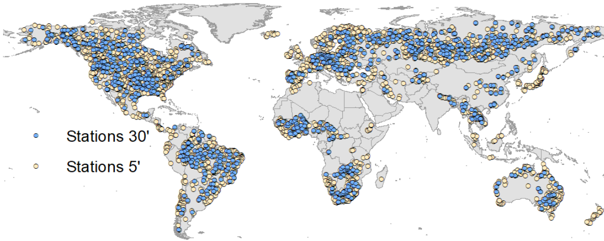
395 Figure 8: Selected station for calibration on 30' (949 stations) and 5' (3,917 stations) (World administrative boundaries by https://www.opendatasoft.com )
