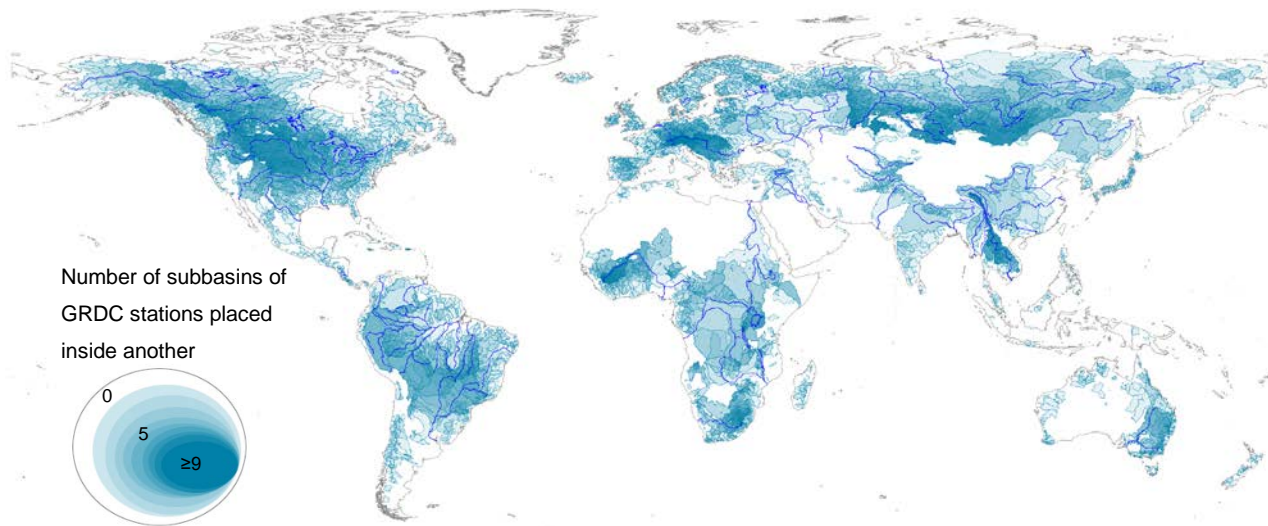
Figure 6. Watershed shapefile of 10241 station using GRDC stations and MERIT network map (World administrative boundaries by https://www.opendatasoft.com )
