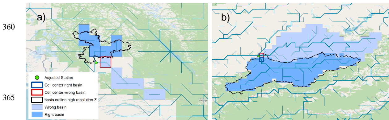
Figure 7: Mismatch of basin allocation because of selection from upstream area only. A) shows the Skeena River, Canada at 30' resolution b) shows the river Khudan, Russia at 5' resolution. © OpenStreetMap contributors 2022. Distributed under the Open Data Commons Open Database License (ODbL) v1.0.
