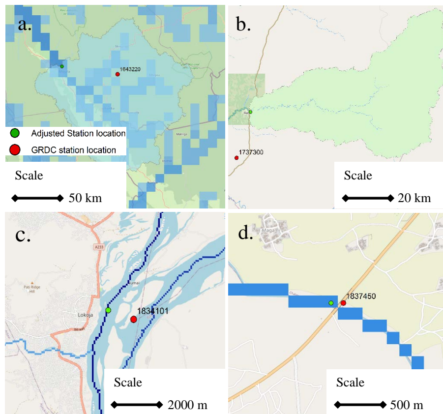
300 Figure 5: Possible errors in station location. © OpenStreetMap contributors 2022. Distributed under the Open Data Commons Open Database License (ODbL) v1.0.
