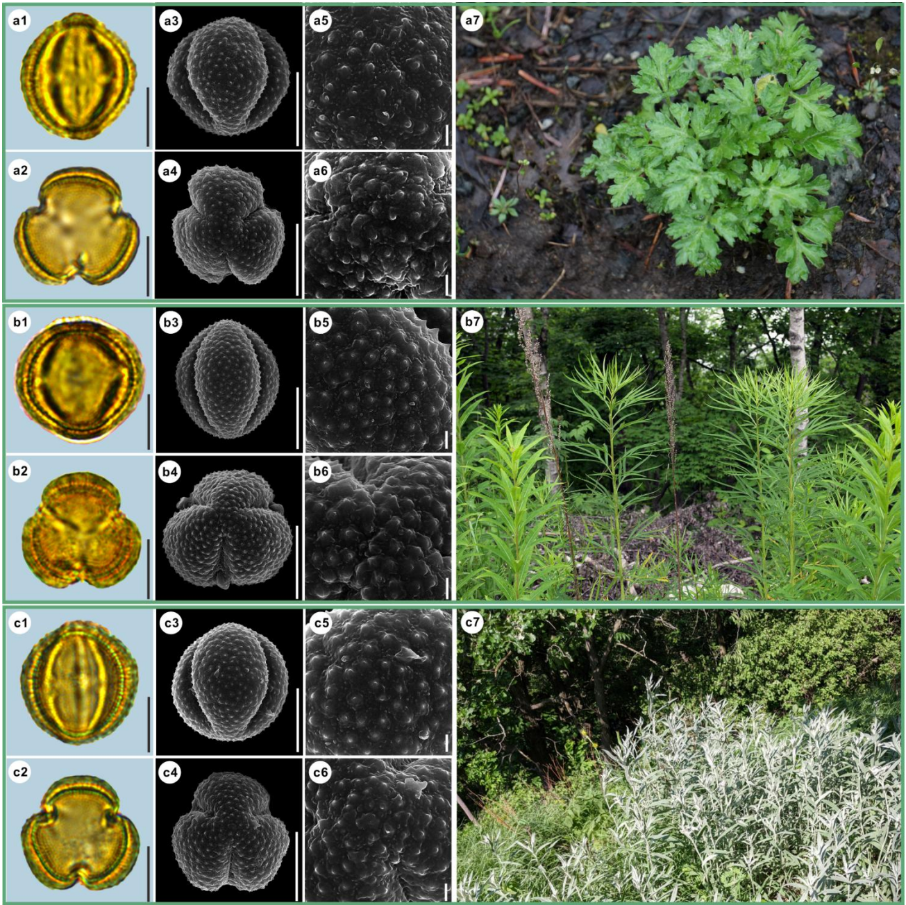
185 186 Figure 5. Pollen grains and the habitats of their source plants. 187 a. Artemisia vulgaris ; b. Artemisia selengensis ; c. Artemisia ludoviciana . 188 Pollen grains in equatorial view under LM (a1, b1, c1) and SEM (a3, a5, b3, b5, c3, c5), in polar view under 189 LM (a2, b2, c2) and SEM (a4, a6, b4, b6, c4, c6), along with the habitats of their source plants (a7 cited from 190 https://www.inaturalist.org/photos/120600448 by © Sara Rall, b7 cited from 191 https://www.inaturalist.org/photos/46352423 by © Gularjanz Grigoryi Mihajlovich, c7 cited from 192 https://www.inaturalist.org/photos/77690333 by © Ethan Rose). 193 Scale bar in LM and SEM overview 10 µm, in SEM close-up 1 µm.
