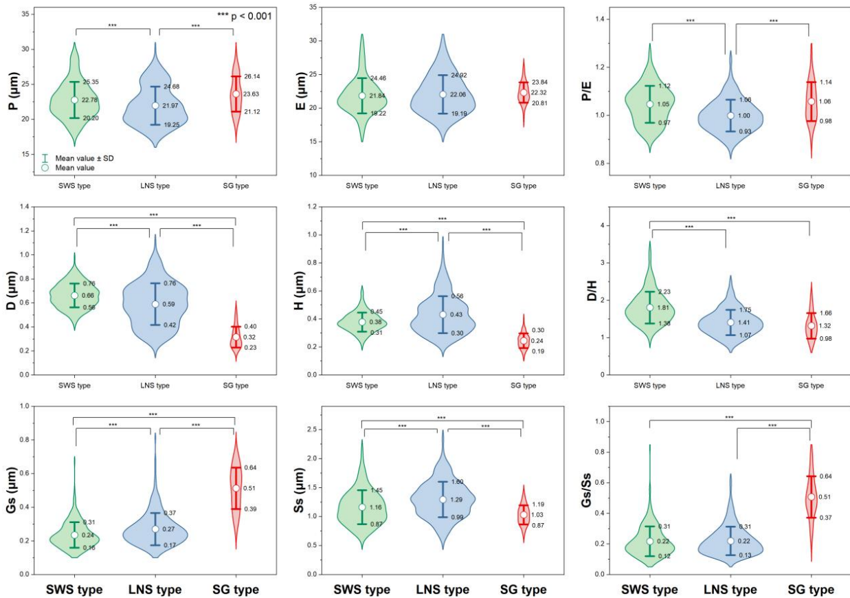
356 357 Figure 19. Violin diagrams of three pollen types from Artemisia , showing the variations ( M \pm SD ) in nine 358 pollen characters (P: length of polar axis; E: length of equatorial axis; D: diameter of spinule base; H: spinule 359 height; Gs: granule spacing; Ss: spinule spacing; Ps: perforation spacing). Asterisks indicate statistically 360 significant differences ( p < 0.001 ).
