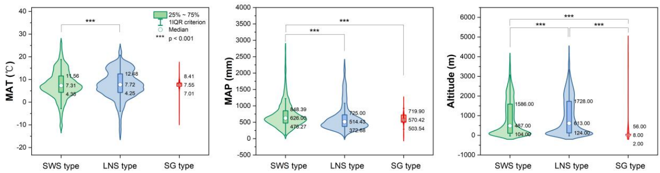
396 397 Figure 21. Violin diagrams of three pollen types from Artemisia , showing the variations (25%-75%) in MAT, 398 MAP, and altitude. Asterisks indicate statistically significant differences ( p < 0.001 ).
