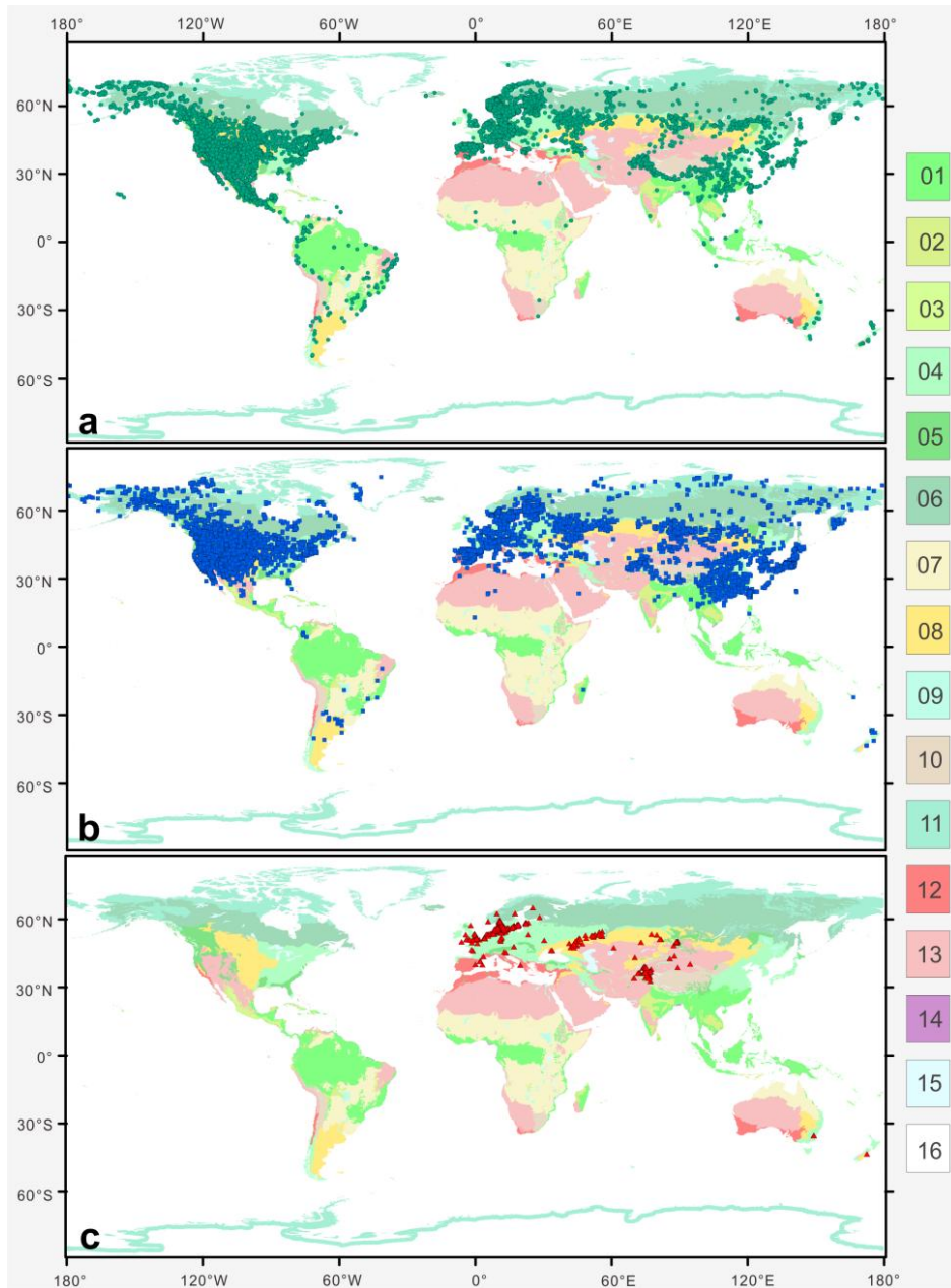
376 377 Figure 20. The global distribution pattern of 3 Artemisia pollen types in terrestrial biomes (modified from 378 Olson et al., 2001). a. SG type; b. LNS type; c. SWS type.
